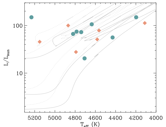
HRD diagram showing the position of our targets falling on silicon in field 2 (green circles) and field 3 (red diamonds), together with isochrones of 1, 5, and 15 Gyr at solar (solid lines) and subsolar (dotted lines) metallicities.
