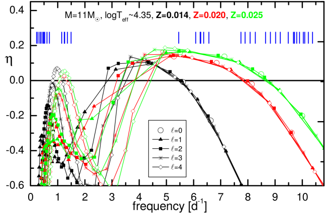
Figure 4. Effect of metallicity on pulsational driving of modes with 0 \leq l \leq 4, m = 0 for a 11 M_{\odot} model of HN Aqr. Theoretical modes with a stability parameter \eta > 0 are driven; the vertical blue bars denote the observed independent frequencies. An initial hydrogen abundance X = 0.71 (?), OPAL opacities, the Asplund et al. (2009) element mixture and no convective core overshooting were used.
