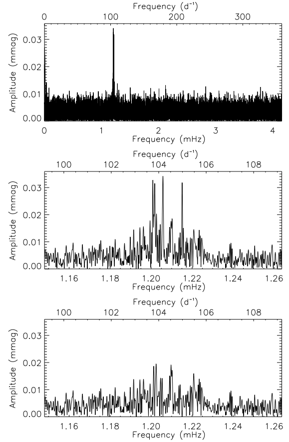
Figure 10. Top: full amplitude spectrum of TIC 139191168 to almost the Nyquist frequency. Middle: zoom of the pulsation modes found in this star. Bottom: the amplitude spectrum of the residuals after removing the frequencies shown in Table 10. There is still excess power in the spectrum, indicating further, unresolved modes or frequency modulation in this star.
