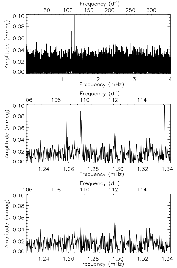
Figure 3. Top: full amplitude spectrum of TIC 12968953 to almost the Nyquist frequency. Clearly evident are the pulsations around 1.3 mHz. Middle: zoom of the pulsation mode frequencies. Bottom: the amplitude spectrum of the residuals after removing the frequencies shown in Table 3, showing no remaining significant signals.
