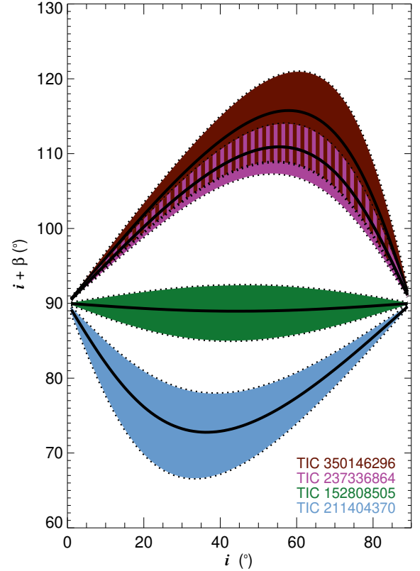
Figure 6. Display of the possible i + \beta combinations, for the four stars where the analysis of the multiplets allows us to set constraints on the stellar pulsation geometry. The full lines and coloured regions limited by dashed lines correspond, respectively, to the values and uncertainties of i + \beta for each star. In stars for which i + \beta \leq 90^\circ only one pulsation pole is observed. Different colours show the results for different stars. The brown and purple stripes indicate regions of overlap of possible solution for TIC 350146296 and TIC 237336864.
