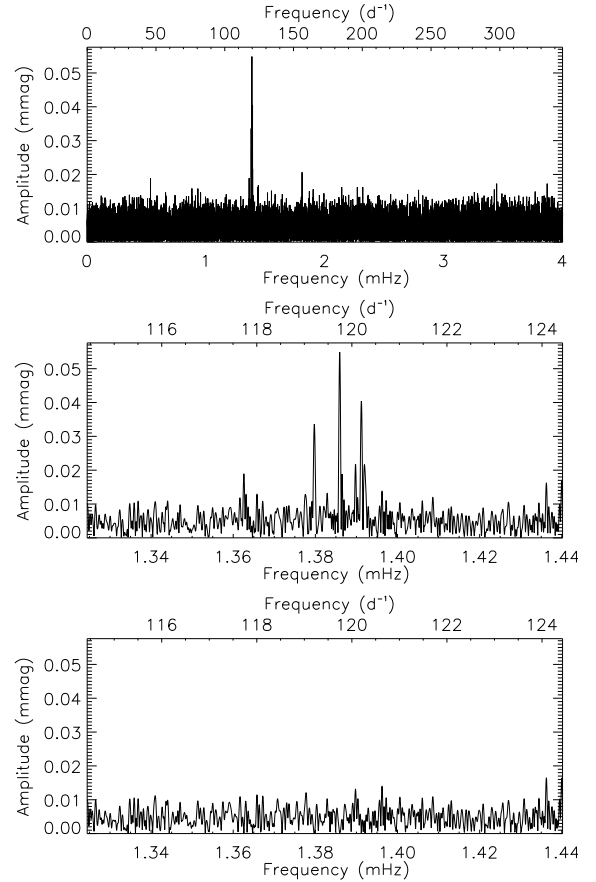
Figure 5. Top: amplitude spectrum of TIC 152808505 to almost the Nyquist frequency. Middle: zoom of the pulsation modes found in this star. Bottom: the amplitude spectrum of the residuals after removing the frequencies shown in Table 5 showing no remaining significant signals.
