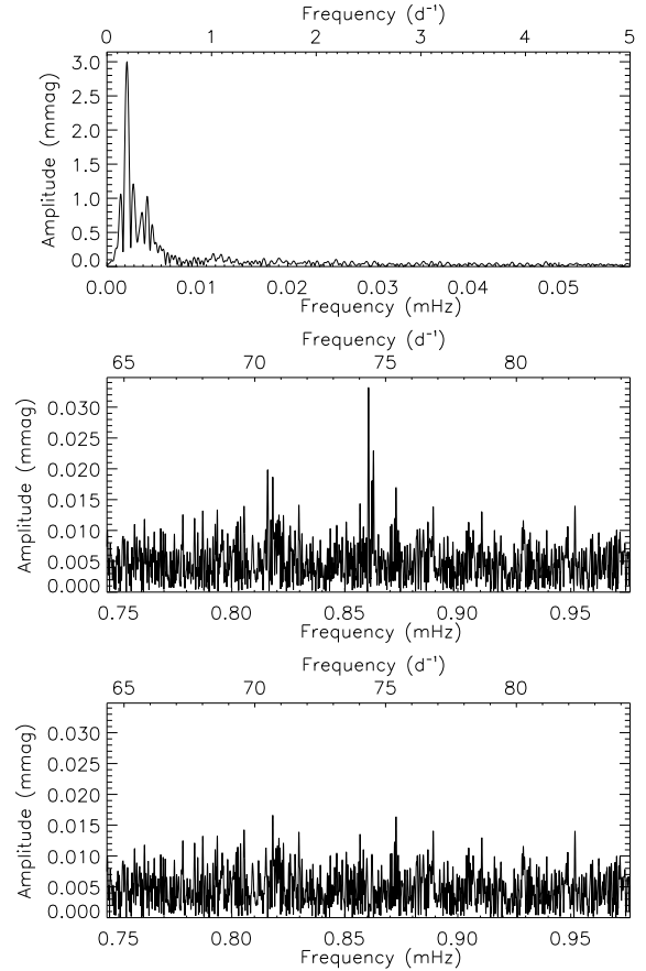
Figure 8. Top: amplitude spectrum at low frequency showing the rotation signal of TIC 431380369. Middle: zoom of the pulsation modes found in this star. Bottom: the amplitude spectrum of the residuals after removing the significant frequencies given in Table 8 showing no remaining significant signals.
