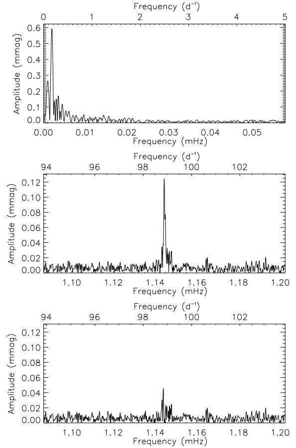
Figure 16. Top: amplitude spectrum at low-frequency showing the rotation signal of TIC 394124612. Middle: zoom of the pulsation mode found in this star. Bottom: the amplitude spectrum of the residuals after removing the frequency shown in Table 15. There is clearly some remaining signal, but this is not resolved in the 27.88-d data set.
