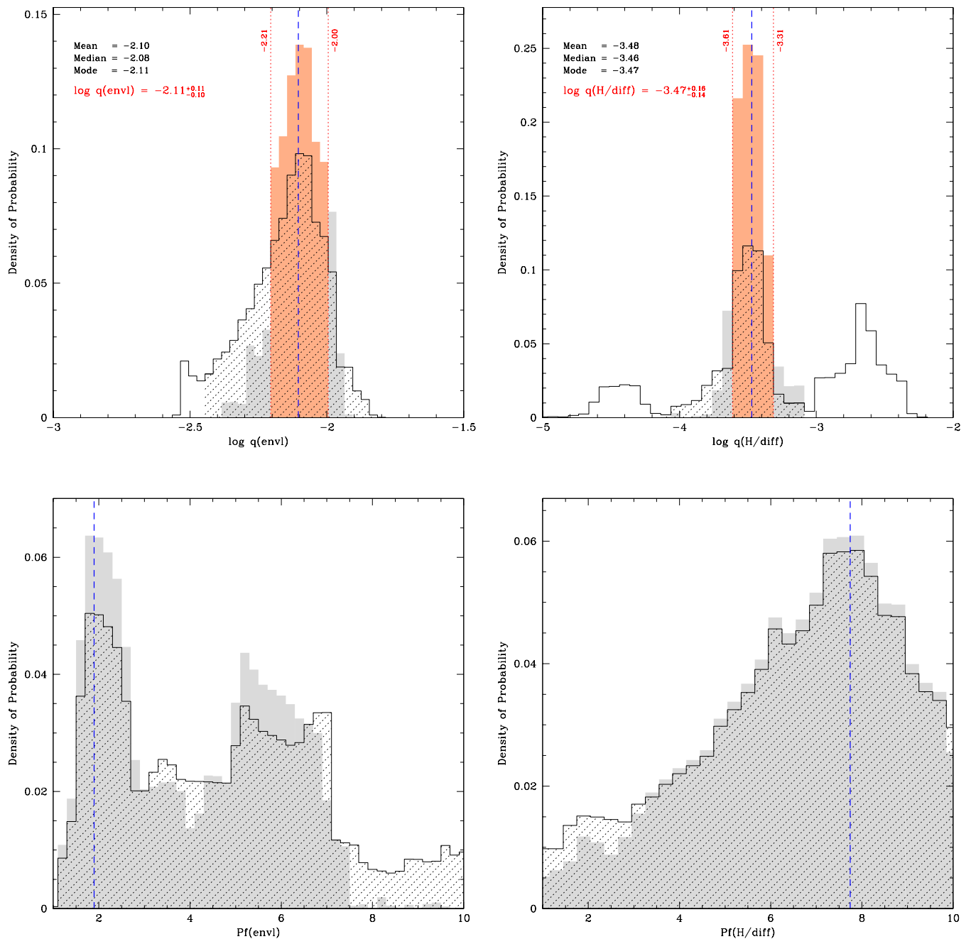
Fig. 8. Same as Figure 6 but for the remaining envelope structural parameters defining the seismic model of TIC278659026. No errors are estimated for Pf(envl) and Pf(H/diff) considering the spread of their distribution.
