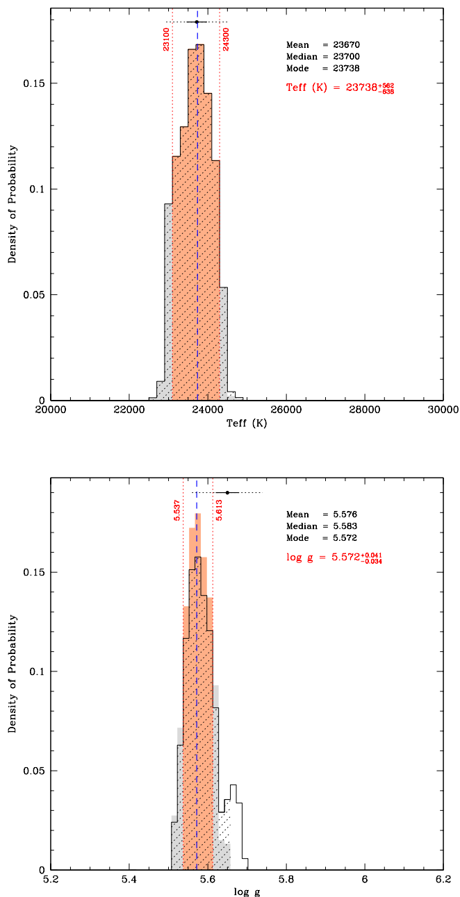
Fig. 6. Probability distributions for T_{\text{eff}} (top panel) and \log g (bottom panel) around the optimal seismic solution for TIC 278659026. Two distributions are superimposed, one resulting from the full sample including all secondary optima (black histograms), and the other computed from a restricted sample focusing on the global optimum (red and grey shaded histogram). This restricted sample is built from excluding parts of the parameter space as indicated in the bottom panel for example and in some panels of Fig. 7, 8, 9, and 10, by bins that do not show the dotted hatched areas. Red-shaded areas delimited by the red vertical dotted lines contain 68% of the restricted probability distribution and provide our estimate of the 1\sigma -error range for the quantity considered. For internal physical consistency of the derived parameters, the adopted value is the one from the optimal model (blue vertical dashed line), which closely corresponds to the mode (maximum) of the distribution. The black dots, and their associated horizontal lines, indicate the measurement obtained independently from spectroscopy, and the 1\sigma (solid) and 3\sigma (dotted) ranges around that value.
