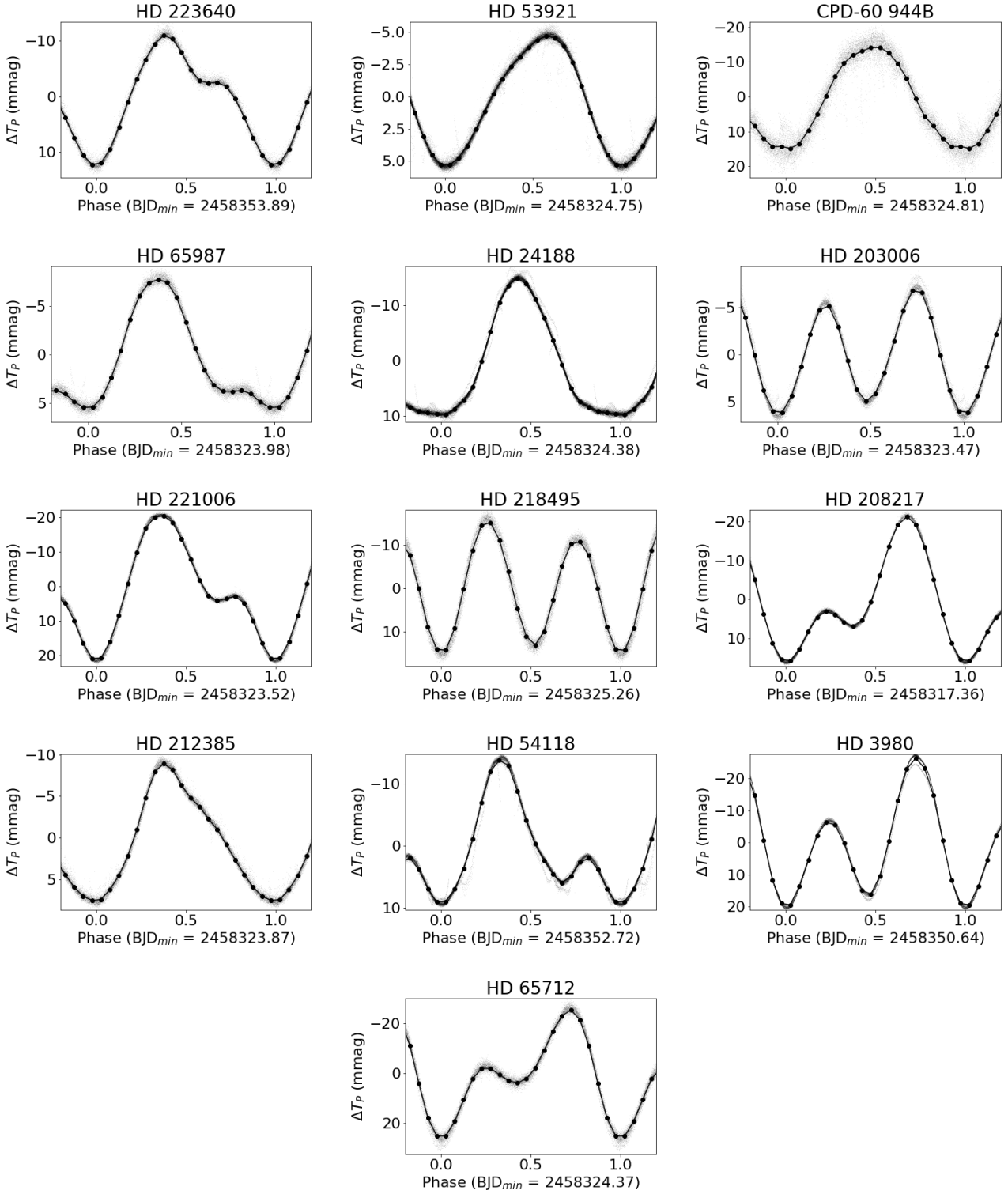
Figure A1. Phase folded light curves (with phase 0 corresponding approximately to minimum light; the time of minimum light used to phase the light curve is indicated on the x-axis of each plot for reference) for the thirteen stars showing potential rotational modulation. The light grey points correspond to individual measurements, and the larger black points connected by a line correspond to binned data (with bins of 0.05 in phase). For some stars, we see streaks of outliers; these are due to artefacts which could not be completely detrended. We find that the light curves have diverse morphologies, with at least nine out of the thirteen showing signs of double-wave variations, and all of them having an asymmetric profile.
