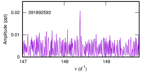
Figure 19. Periodogram of TIC 391892593.
