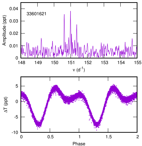
Figure 2. Periodogram of TIC 33601621 and the light curve phased with \nu_{\text{rot}} = 0.3758 \text{ d}^{-1} . \Delta T is the relative TESS intensity in parts per thousand.
