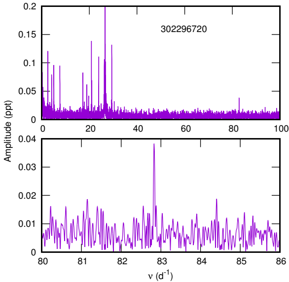
Figure 24. Periodogram of TIC 302296720 which appears to be a \delta Scuti star with a single high frequency (bottom panel).
