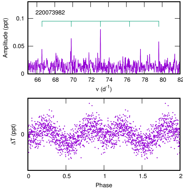
Figure 16. Periodogram of TIC 220073982 showing peaks spaced by 3.260 \text{ d}^{-1} . The light curve phased with 3.260 \text{ d}^{-1} is shown in the bottom panel.
