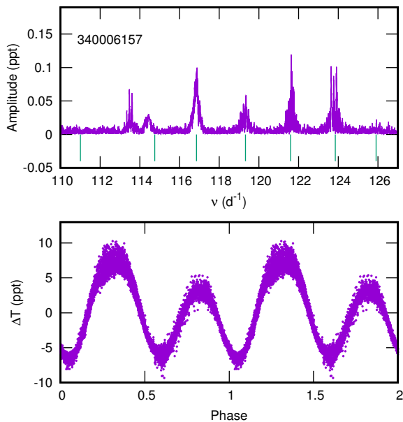
Figure 7. Periodogram for TIC 340006157 and the light curve phased with \nu_{\text{rot}} = 0.13015 \text{ d}^{-1} . The vertical lines below the periodogram show the frequencies listed in Matthews et al. (1987).
