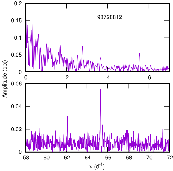
Figure 23. Periodogram of TIC 98728812 with some barely significant low-frequency peaks suggestive of a \gamma Dor variable and two high-frequency peaks (bottom panel).
