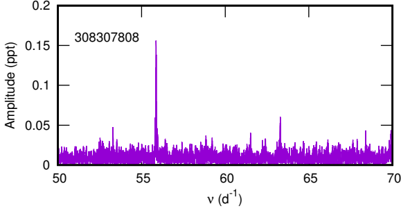
Figure 20. Periodogram of TIC 308307808.
