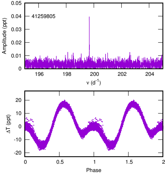
Figure 2. Periodogram of TIC41259805 and the light curve phased with \nu_{\text{rot}} = 0.58326 \text{ d}^{-1} .
