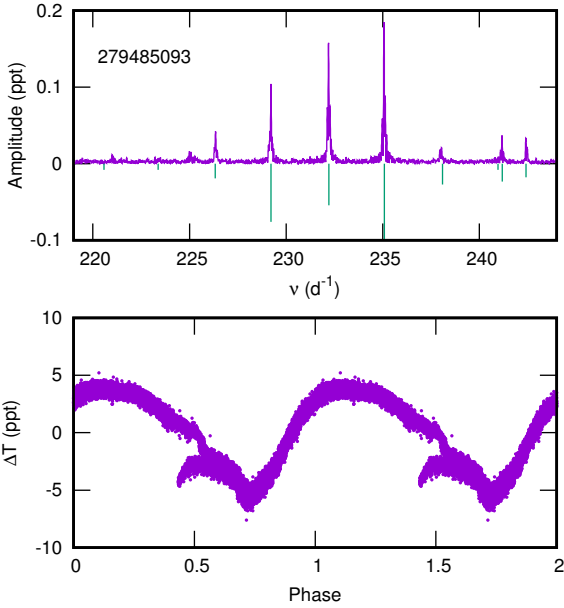
Figure 5. Periodogram for TIC 279485093 and the light curve phased with \nu_{\text{rot}} = 0.080274 \text{ d}^{-1} . The vertical lines indicate frequencies in the literature.
