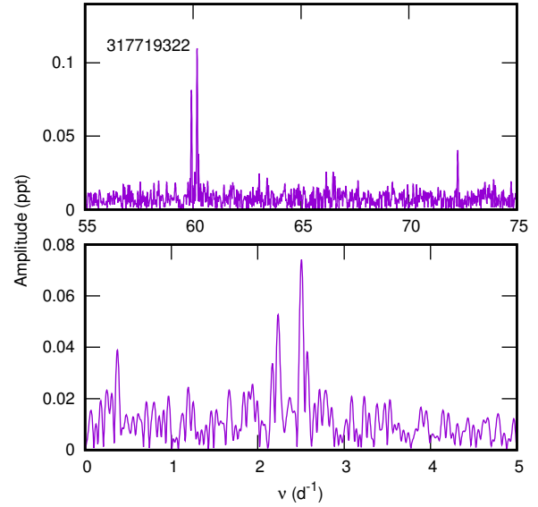
Figure 25. Periodograms of TIC 317719322 showing the high-frequency and the low-frequency regions.
