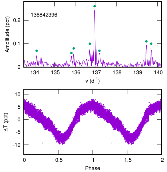
Figure 3. Periodogram of TIC136842396 and the light curve phased with \nu_{\text{rot}} = 0.1169 \text{ d}^{-1} . The dots in the periodogram indicate the extracted frequencies.
