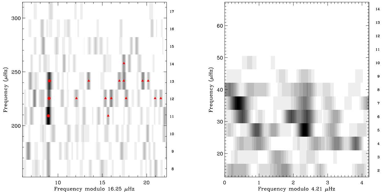
Figure 3. Grayscale échelle diagram of the smoothed PSD of HD 212771 (left panel) and HD 203949 (right panel). The pressure radial order, n_p , is indicated along the right y -axis. Identified individual modes for HD 212771 (see Fig. 4 and Table 3) are marked with red circles ( \ell = 0 , radial modes) and red triangles ( \ell = 1 , dipole modes). A proxy for \Delta\nu of 4.21 \mu\text{Hz} (within errors of the quoted value in Table 2) is used in the right panel to enhance the vertical alignment of the ridges.
