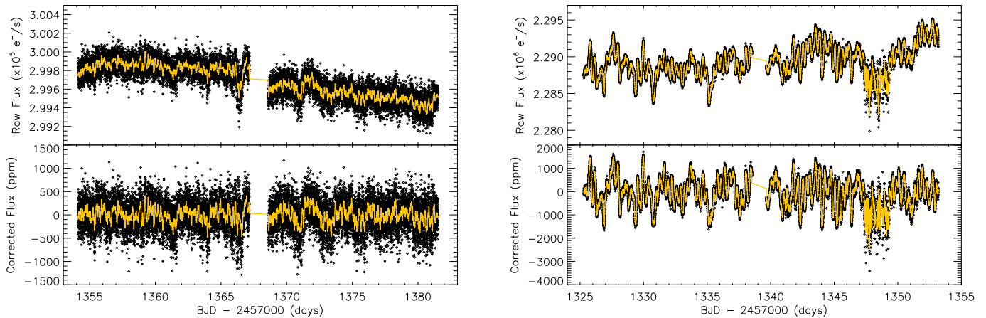
Figure 1. Light curves of HD 212771 (left panel) and HD 203949 (right panel) produced by the TASOC photometry pipeline. In each panel, raw (top) and corrected (bottom) 2-minute cadence light curves are displayed. A smoothed — using a 1-hour (HD 212771) and 10-minute (HD 203949) boxcar filters — version of the light curve is depicted by a yellow curve in each subpanel.
