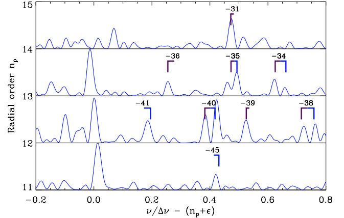
Figure 4. Mixed-mode pattern of HD 212771. The PSD along each pressure radial order, n_p , is shown as a function of reduced frequency, \nu/\Delta\nu - (n_p + \epsilon) , where \epsilon is a phase shift sensitive to the properties of the near-surface layers of the star. The three prominent radial modes have a reduced frequency close to 0 (modulated by acoustic glitches). The mixed-mode orders, n_m , are indicated, with color coding the azimuthal order ( m = -1 in dark purple and m = 1 in blue; see Table 3).
