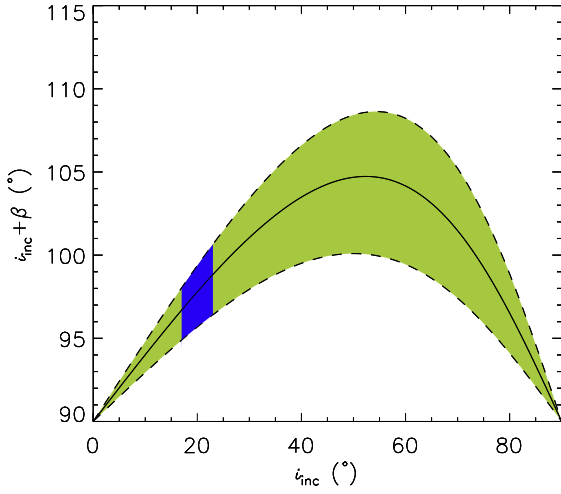
Figure 6. Visualisation of the values of i_{\text{inc}} and \beta that satisfy equation (1). The green shaded region bound by the dashed lines represents the 1\sigma error range. As can be seen i_{\text{inc}} + \beta is always greater than 90^\circ , suggesting we see both pulsation poles. The blue shaded region represents the values of i_{\text{inc}} , which are estimated from spectroscopy. See the discussion for details.
