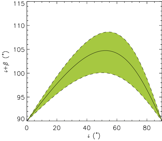
Figure 6. Visualisation of the values of i and \beta that satisfy equation (1). The shaded region bound by the dashed lines represents the 1\sigma error range. As can be seen i+\beta is always greater than 90^\circ , suggesting we see both pulsation poles.
