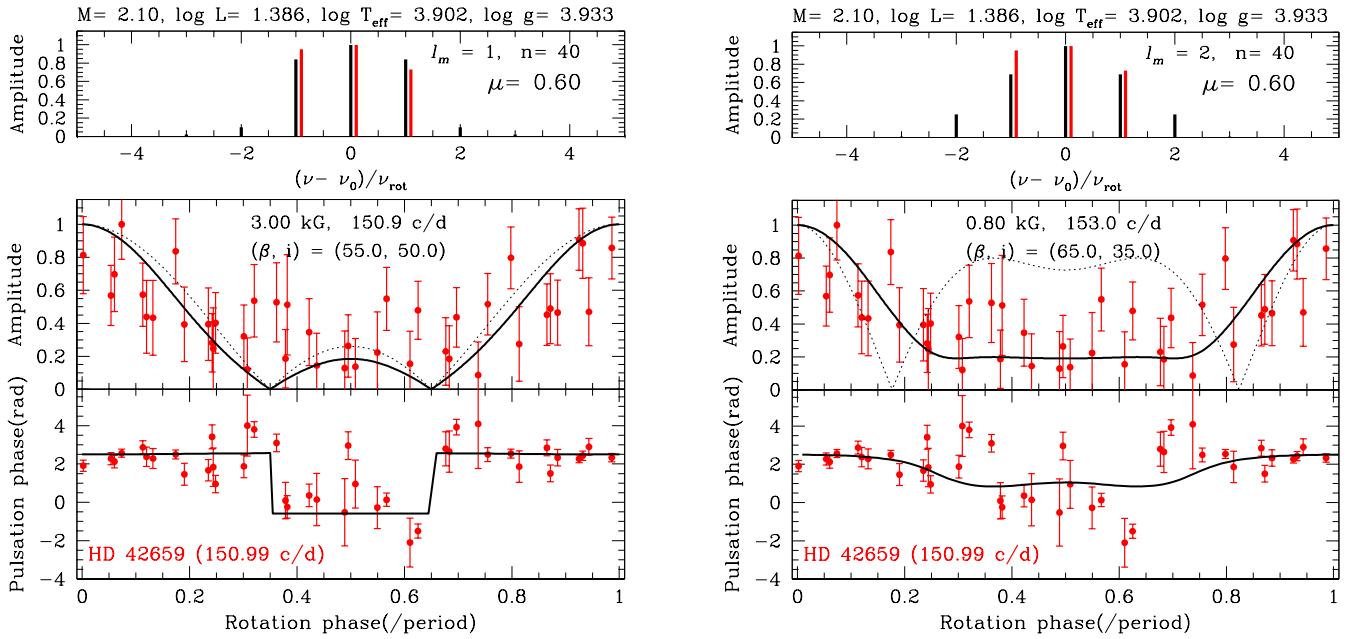
Figure 9. Left: best fitting distorted dipole model to the observed amplitude and phase variations. We show a representative model, as any values of i , and \beta which satisfy equation 1 and Fig. 6 provide good fits to the observations. Right: the best fitting distorted quadrupole model. In this case, only a narrow range of parameters allow us to obtain a good fit. In both cases, the red colour represents the observations, with the black being the models. The dotted lines represent the non-distorted case in each model.
