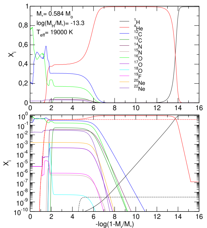
Fig. 1. Upper panel: fractional abundance by mass of selected nuclear species in terms of the outer mass fraction, corresponding to a DA WD model characterized by M_{\star} = 0.584 M_{\odot} , T_{\text{eff}} = 19000 \text{ K} and \log(M_{\text{H}}/M_{\star}) = -13.3 . Lower panel: same as in the upper panel, but with a logarithmic scale for the chemical abundances. In this panel, the black and red dashed lines correspond to initial fractional abundances of H and He, respectively.
