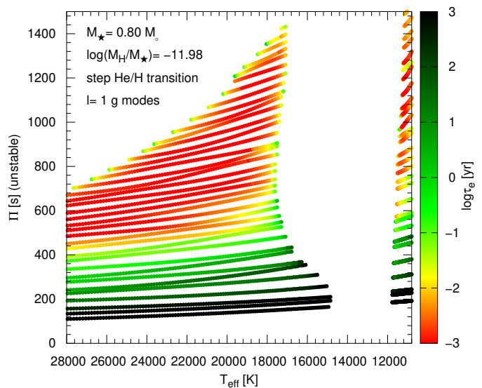
Fig. 9. Same as Fig. 5, but for M_{\star} = 0.80M_{\odot} . Also for these high-mass WD models, many g modes are excited at high effective temperature.
