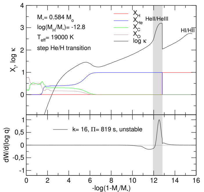
Fig. 6. Upper panel: same as in Fig. 4, but for the case in which \log(M_{\text{H}}/M_{\star}) = -12.8 . Lower panel: the normalized differential work function corresponding to an unstable g mode with k = 16 and period \Pi = 819 s.
