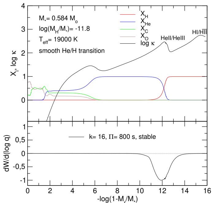
Fig. 2. Upper panel: inner chemical profiles of ^{16}\text{O} , ^{12}\text{C} , ^4\text{He} and H, and the logarithm of the Rosseland opacity ( \kappa ) versus the outer mass fraction coordinate, corresponding to a DA WD model with M_* = 0.584M_\odot , \log(M_{\text{H}}/M_*) = -11.8 , and T_{\text{eff}} = 19000 K. The H/He interface is shaped by element diffusion. The bumps in \kappa due to the second ionization of He and the ionization of H are evident. Lower panel: the normalized differential work function corresponding to a stable g mode with k = 16 and period \Pi = 800 s.
