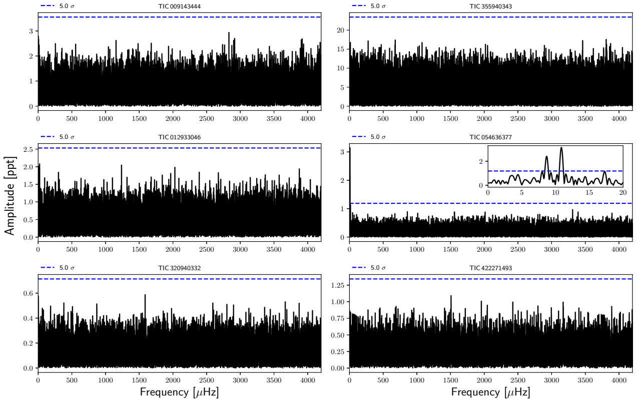
Fig. A.1. The amplitude spectra of warm DA WDs. The blue dashed horizontal line indicates the threshold ( 5\sigma ). The inset is a blow-up of the amplitude spectra at the low-frequency regime for the few stars where some frequencies are above 5\sigma , as discussed in the text.
