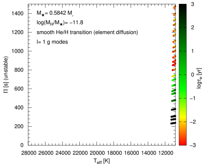
Fig. 3. Unstable \ell = 1 g -mode periods ( \Pi ) in terms of the effective temperature for the sequence of DA WD models with M_* = 0.584M_\odot and \log(M_{\text{H}}/M_*) = -11.8 . Color coding indicates the value of the logarithm of the e -folding time ( \tau_e ) of each unstable mode (right scale). Only unstable modes for effective temperatures characteristic of the ZZ Ceti stage ( T_{\text{eff}} \lesssim 11500 K) are found.
