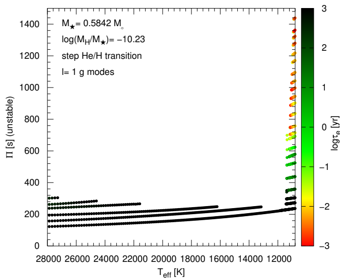
Fig. 8. Same as Fig. 5 but for \log(M_{\text{H}}/M_{\star}) = -10.23 . Here, a few low-order modes ( k = 1, \dots, 6 ) are marginally unstable apart from the unstable g modes at the ZZ Ceti’s effective temperatures.
