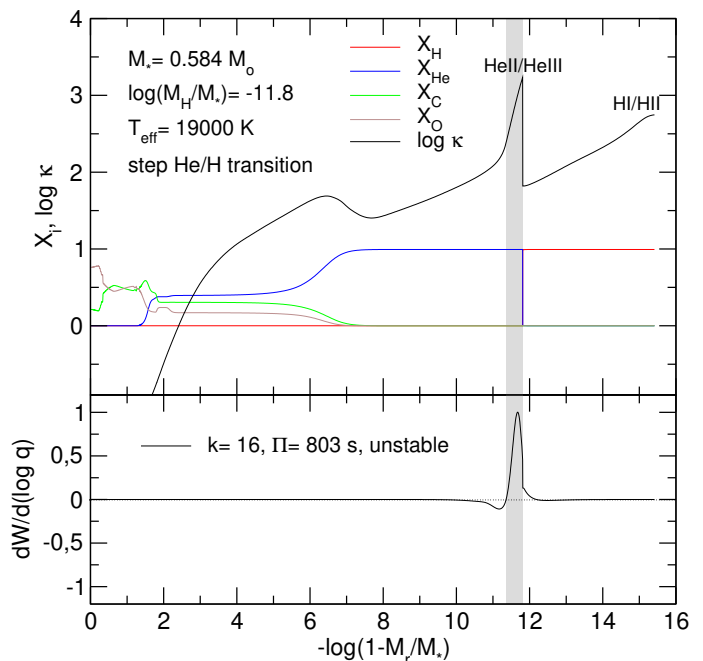
Fig. 4. Upper panel: same as in Fig. 2, but for the extreme case in which the H/He interface is assumed to be discontinuous (step-like shape). The vertical gray strip marks the convection zone driven by the 2 nd ionization of He. Lower panel: the differential work function for an unstable g mode with k = 16 and period \Pi = 803 s.
