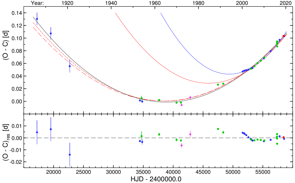
Figure 4. Top: O – C diagram for the light (green dots) and radial velocity (blue dots) times of maximum given in Tables 3 and 4. A constant shift of +0.070 d was applied to the times of maximum radial velocity. Two violet dots correspond to T_{\max} derived from TD-1A and ANS UV observations, while the red dot corresponds to T_{\max} derived from the TESS data. These three values of O – C are not considered in the fits. The four parabolas are four fits with different weighting schemes: weights proportional to \sigma^{-2} (red continuous line), \sigma^{-1} (red long-dashed line), \sqrt{\sigma} (red short-dashed line) and with equal weights (black line). The blue line shows the fit to the recent (2000 – 2019) RV data only ( \dot{P} = 0.97 \pm 0.13 s/cen with equal weights). Bottom: residuals from the fit with equal weights.
