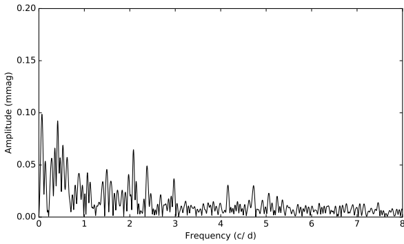
Figure 2. Fourier amplitude spectra of TESS sectors XX and YY photometry showing weak peaks at low frequencies.
