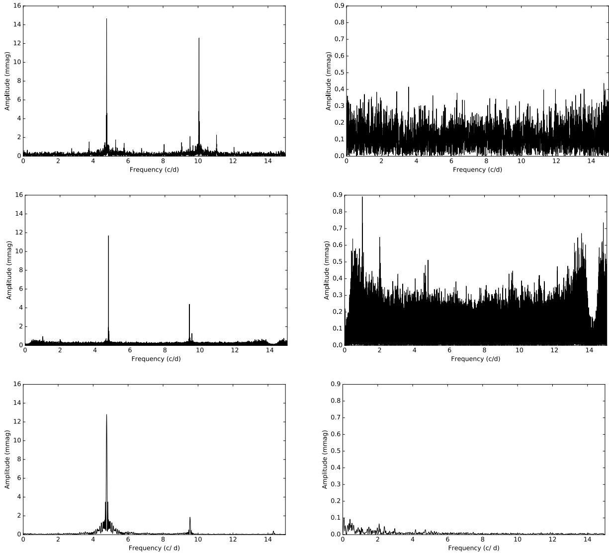
Figure 1. Fourier amplitude spectra of BTr+BHr data (upper frames) and SMEI data (lower frames) in mmag. Upper left: BTr+BHr data. Upper right: Spectrum of residuals following prewhitening with the fundamental frequency of 4.771491 \text{ d}^{-1} and the first two harmonics. Middle left: Orbit-averaged SMEI data. Middle right: Spectrum of residuals following prewhitening with the fundamental frequency of 4.771517 \text{ d}^{-1} and its first two harmonics. Bottom left: TESS data. Lower right: Spectrum of residuals following prewhitening with the fundamental frequency of 4.771483(6) \text{ d}^{-1} and its first four harmonics. In the BRITe and SMEI residuals, the peaks at 1 and 2 \text{d}^{-1} are instrumental, as are peaks between 3 and 5 \text{d}^{-1} .
