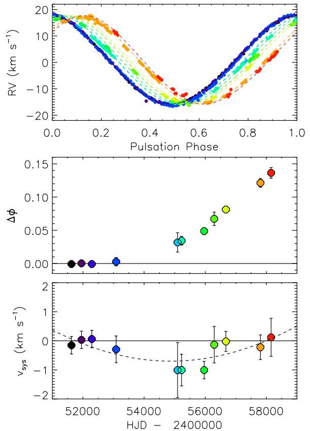
Figure 6. Top: CORALIE and ESPaDOnS RVs phased with the pulsation period determined from the first epoch of CORALIE data. Colours indicate epochs. Dashed lines show 3 rd -order harmonic fits to the CORALIE data, shifted to minimize the standard deviation of the residuals. Middle: phase shift \Delta\phi of the RV curve in each epoch. Bottom: systemic velocity v_{\text{sys}} determined from the mean residual RV after subtraction of the phase-shifted curves in the top panel. The dashed curve in the bottom panel relates to the most conservative scenario for the light-time hypothesis (see text).
