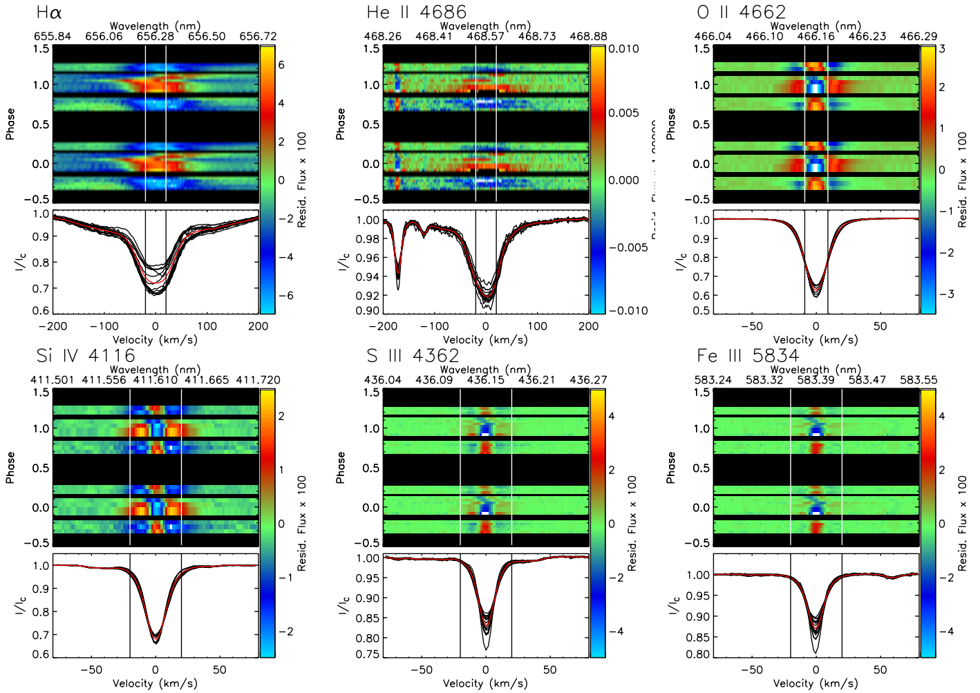
Figure 8. Dynamic spectra displaying line profile variations coherent with the rotational ephemeris of Shultz et al. (2017, 2018). Top panels show residual intensity mapped to colour as a function of rotational phase; bottom panels show phase-binned intensity spectra (black) and the mean reference spectrum (red).
