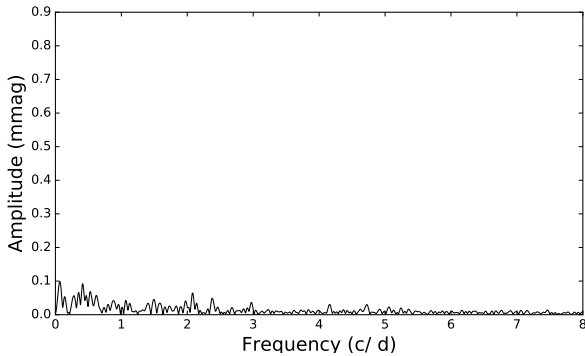
Figure 2. Fourier amplitude spectra of TESS sector 6 photometry showing weak peaks at low frequencies.
