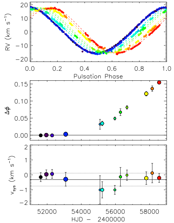
Figure 6. Top: CORALIE and ESPaDOnS RVs phased with the pulsation period determined from the first epoch of CORALIE data. Colours indicate time bins . Dashed lines show 3 rd -order harmonic fits to the CORALIE data, shifted to minimize the standard deviation of the residuals. Middle: phase shift \Delta\phi of the RV curve in each epoch. Bottom: systemic velocity v_{\text{sys}} determined from the mean residual RV after subtraction of the phase-shifted curves in the top panel. The solid line shows the mean v_{\text{sys}} , the dotted lines the standard deviations. The dashed curve relates to the most conservative scenario for the light-time hypothesis (see text). In the middle and bottom panels, symbol size is proportional to the log of the number of points in each bin.
