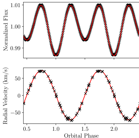
Figure 14. The model phoebe2 light curve (top) and radial velocity curve (bottom) overlaid on the observations.
