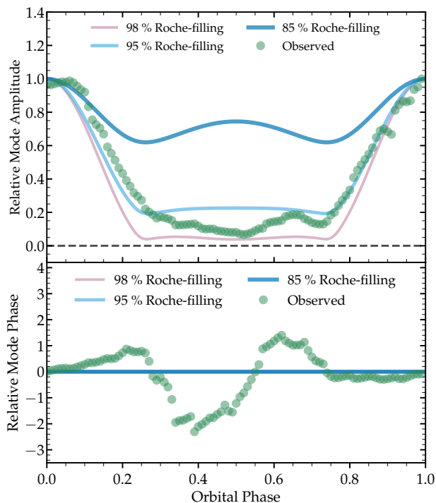
Figure 19. : Top: As a function of orbital phase, amplitude (top) and phase (bottom) modulation of a radial mode with latitudinal flux perturbation given by Fig. 18, viewed at an inclination angle of i = 50^\circ to the orbital axis. Green dots are the (smoothed) observed phase variation of mode \nu_2 . Bottom: Corresponding mode phase variations.
