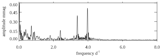
Figure 9. Amplitude spectrum after pre-whitening the orbital harmonic series, showing peaks for at least 3 g modes. The lowest frequency peaks are probably instrumental artefacts.
