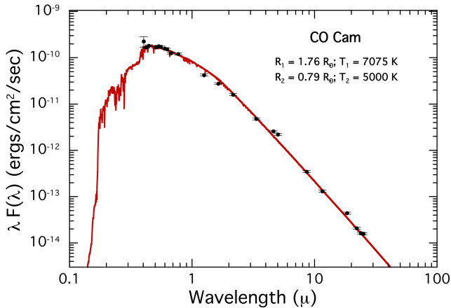
Figure 10. Spectral fit to the available SED data using the combined flux from the two stars. This emerges directly from the MCMC analysis where the SED is fitted during each link of the MCMC.
