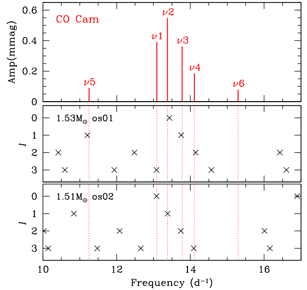
Figure 15. Central pulsation frequencies of the multiplets in the p-mode range of CO Cam (top panel) are compared with pulsation frequencies (crosses) of two models of 1.53 M_{\odot} and 1.51 M_{\odot} . The vertical axes of the middle and bottom panels represent latitudinal degree, \ell . Each model is the best model for a given overshooting parameter, where os01 and os02 mean that h_{\text{os}} = 0.01 and 0.02, respectively.
