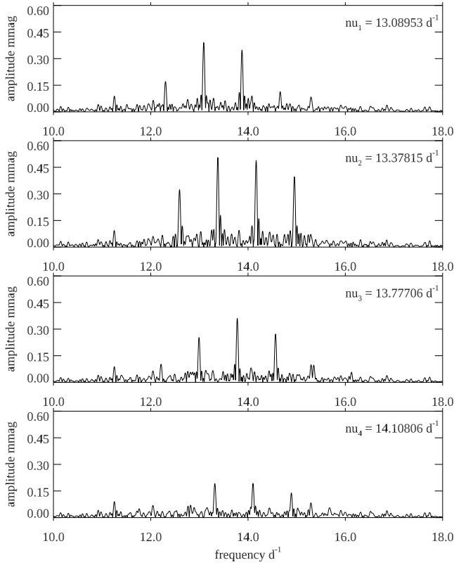
Figure 7. The four mode frequency septuplets isolated.
