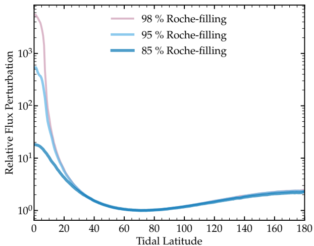
Figure 18. Flux perturbations as a function of angle away from the line of apsides, for the p mode in HD 74423 (Fuller et al., in prep). While we do not expect these models to apply to CO Cam, which is far less Roche lobe filling than HD 74423, they match the observed amplitude variation fairly well, as shown in Fig. 19.
