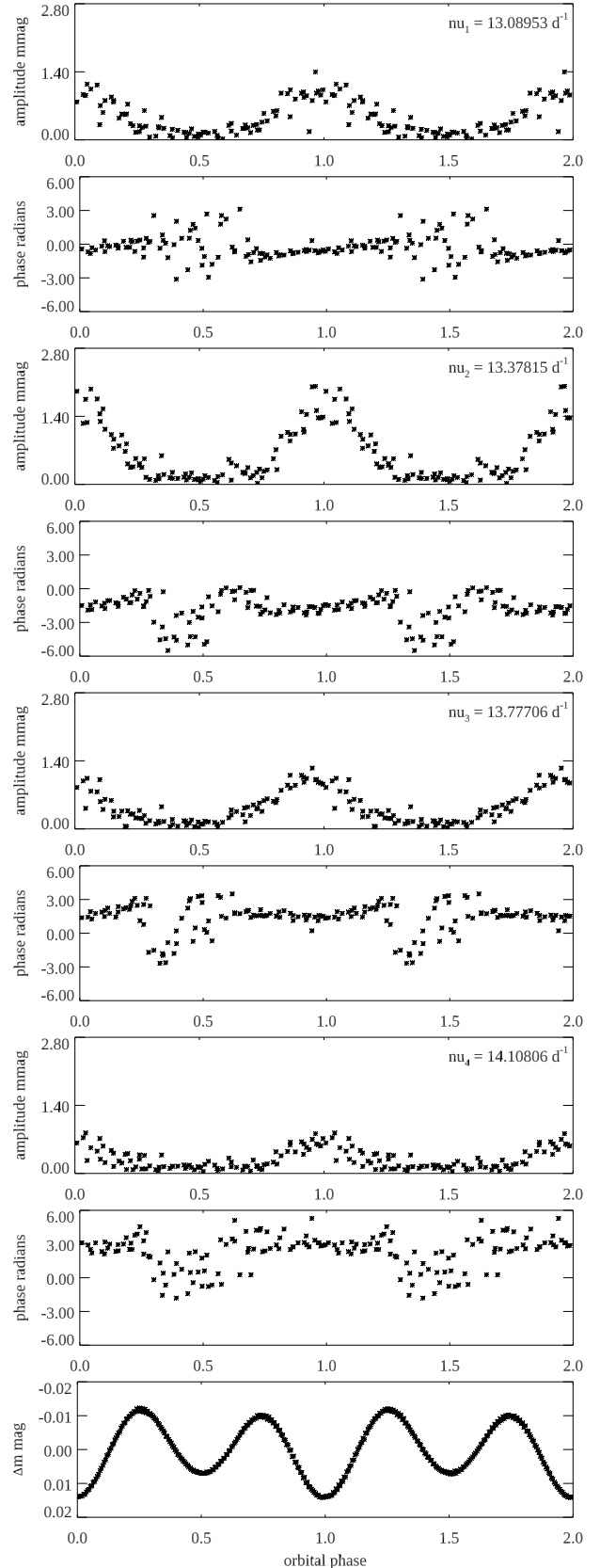
Figure 8. Each pair of panels shows the pulsation amplitude and phase variation as a function of orbital phase for the isolated data (cf. Fig. 7). The bottom panel shows the orbital light variations as a function of orbital phase. It can be seen that pulsation maximum and orbital light minimum coincide, as required by the oblique pulsator model.
