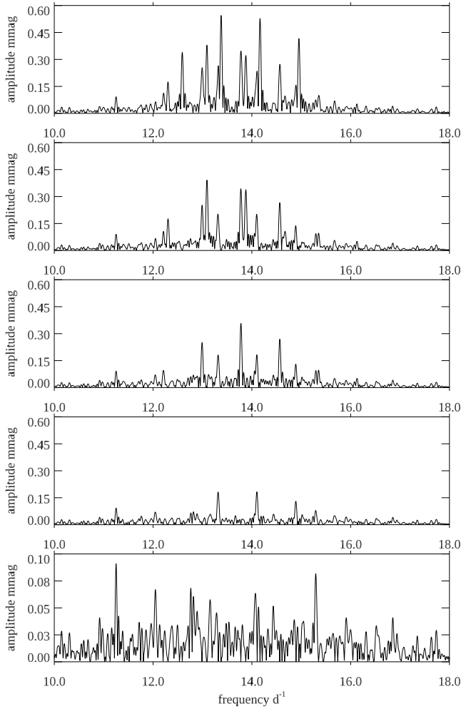
Figure 5. Top: The amplitude spectrum of the high-pass data, showing the pulsation frequencies and their orbital sidelobes. Sequential pre-whitening of multiplets based on the highest peaks is shown in the 5 panels. The last of those, the bottom panel, shows that there is significant amplitude left after pre-whitening the highest amplitude four multiplets. The two highest peaks, \nu_5 = 11.252 \text{ d}^{-1} and \nu_6 = 15.293 \text{ d}^{-1} , show some orbital sidelobes, but these are too close to the noise level to find the full multiplet, thus we stopped the analysis with four secure oblique pulsator multiplets. Note the change of ordinate scale in the bottom panel.
