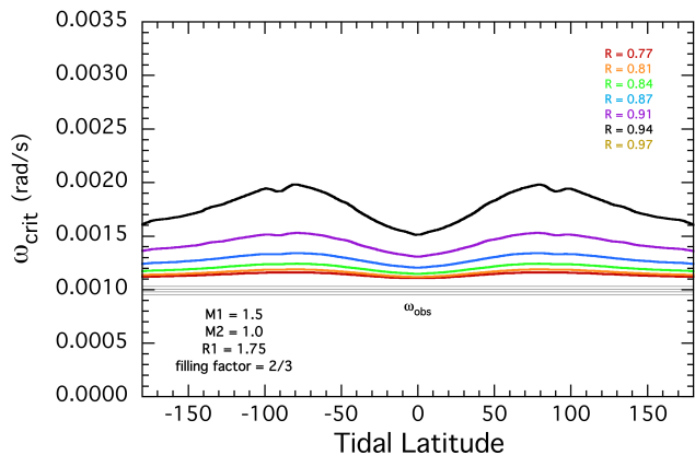
Figure 16. The acoustic cutoff frequency as a function of tidal latitude (measured in the orbital plane) of a tidally distorted polytropic model with the same Roche geometry as CO Cam. Different colours correspond to different radial coordinates within the star, and the horizontal black lines are the observed pulsation frequencies ( \omega_1 through \omega_4 ) of CO Cam.
