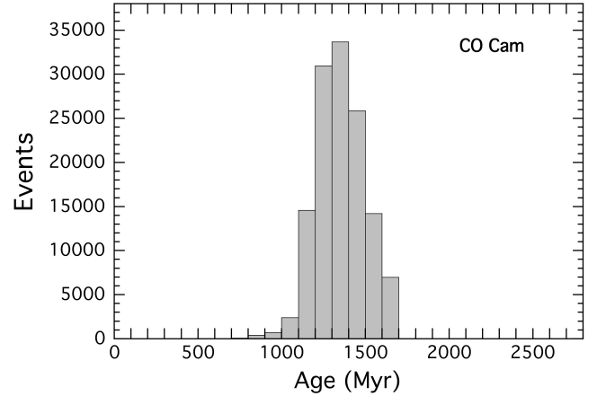
Figure 11. The age probability distribution for the system deduced from the MCMC analysis of the system parameters and the MIST evolution tracks (see Sect. 6.2 for references).
