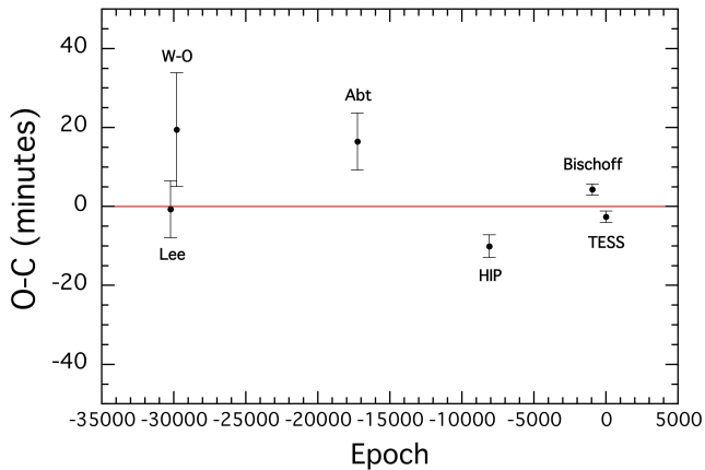
Figure 2. The O - C diagram for CO Cam based on the data points given in Table 2. The reference epoch and period were found to be t_0 = \text{JD } 2458693.3449 \pm 0.0035 and P = 1.2709927 \pm 0.0000007 d. References to the labeled points can be found in Table 2. The red line is a linear \chi^2 fit to the O - C curve.
