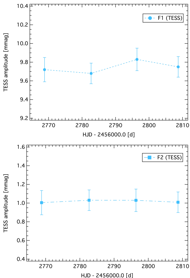
Fig. 14. Amplitude behaviour of the two main pulsation frequencies, F_1 (filled circles, top panel) and F_2 (filled squares, bottom panel) based on four subsets of TESS data. The error bars display the one-sigma error derived using SMURFS .
