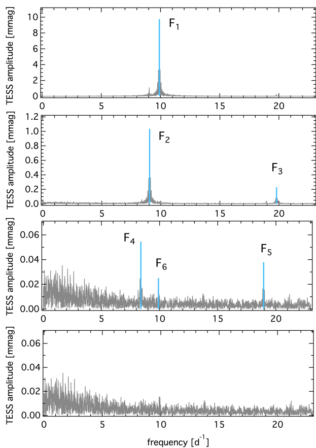
Fig. 5. Fourier analysis of the TESS data: The amplitude spectrum of the original data with F_1 identified (top panel), amplitude spectrum after prewhitening F_1 (second panel from the top), amplitude spectrum after prewhitening F_1 , F_2 , and F_3 (third panel from the top), and residual amplitude spectrum after prewhitening all significant frequencies (bottom panel).
