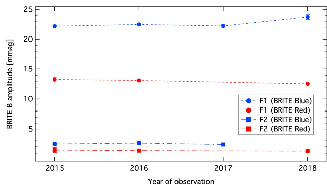
Fig. 12. Annual behaviour of the amplitudes of the two main pulsation frequencies, F_1 (filled circles) and F_2 (filled squares) based on the BRITE-Constellation observations in the B (blue) and R (red) filter conducted every year from 2015 to early 2019. The one-sigma error bars in the figure are mostly smaller than the symbol size.
