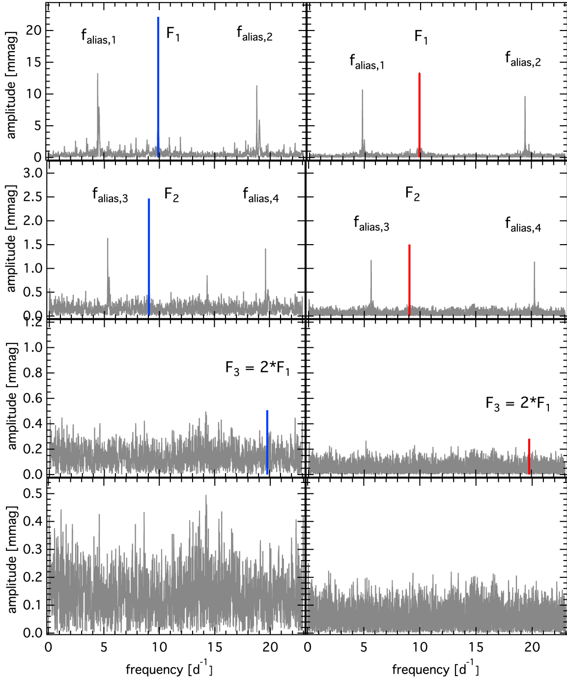
Fig. B.2. Amplitude spectra of the BRITe-Constellation data obtained in 2015: Combined blue filter data are shown on the left side, combined red filter data on the right side. Top panels show the amplitude spectra of the original data with F_1 identified, the second panels illustrate the amplitude spectra after prewhitening F_1 , the third panels those after prewhitening F_1 and F_2 , and the bottom panel displays the residual amplitude spectra after prewhitening all significant frequencies. An explanation for the identified alias frequencies is given in the text.
