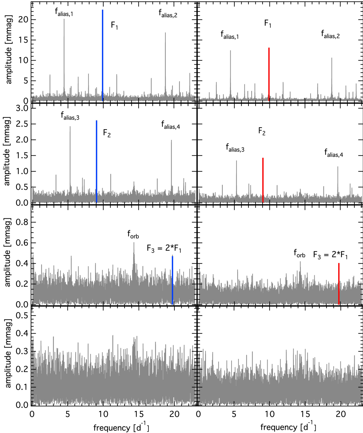
Fig. 3. Amplitude spectra of the BRITE-Constellation data obtained in 2016: BAb blue filter data are shown on the left side, UBr red filter data on the right side. Top panels show the amplitude spectra of the original data with F_1 identified, the second panels illustrate the amplitude spectra after prewhitening F_1 , the third panels those after prewhitening F_1 and F_2 , and the bottom panel displays the residual amplitude spectra after prewhitening all significant frequencies. An explanation for the identified alias frequencies is given in the text.
