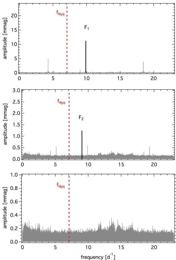
Fig. 4. Amplitude spectra of the SMEI data: original data with F_1 identified (top panel), amplitude spectra after prewhitening with F_1 and showing F_2 (middle panel), and residuals after prewhitening F_1 and F_2 (bottom panel). The position of the Nyquist frequency is marked in red.
