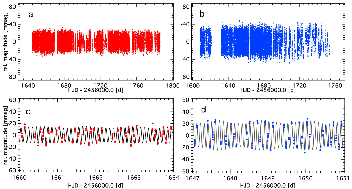
Fig. 1. BRITE photometric time series obtained by UBr (panel a) and BAb in 2016 (panel b) to the same Y-axis scale and with a time base of 170 days on both X axes. Panels c and d show 4-days subsets of the UBr and BAb 2016 light curves binned to 5-minute intervals and the corresponding multi-sine fit with the two identified pulsation frequencies again to the same Y-axis scale and with a time base of 4 days on both X axes.
