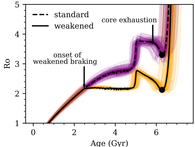
Figure 7. Predictions from a standard spin-down model (purple/dashed) and weakened braking model (orange/solid) for the evolution of the Rossby number in 94 Aqr Aa. For each model, the best-fit combination of mass and composition is shown as a dark line and the best fit age is marked with a solid point. In addition, 250 randomly drawn posterior samples of mass and composition are shown, truncated at the end of the subgiant branch.
