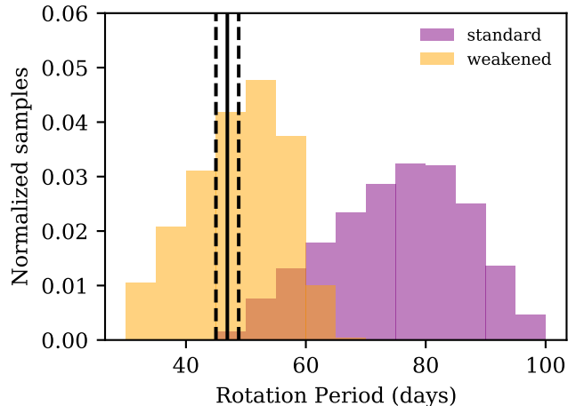
Figure 6. Predictions from a standard spin-down model (purple) and weakened braking model (orange) for the rotation period of 94 Aqr Aa. The observed rotation period from Mount Wilson data is shown with black vertical lines.
