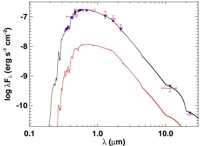
Figure 4. Spectral energy distribution (SED) fit to the broadband photometry of 94 Aqr A. The fit to 94 Aqr Aa is shown in black, with observed fluxes as red symbols and bandpass integrated model fluxes as blue symbols. The red curve shows the SED of the companion (Ab), which is used to correct for light contamination in the SED of 94 Aqr Aa.
