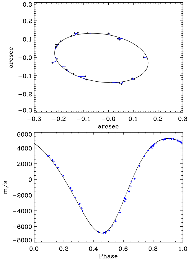
Figure 5. Results of a simultaneous fit to the astrometry (top) and spectroscopy (bottom) of 94 Aqr A. Data are shown with blue points, and the fit is shown in black.
