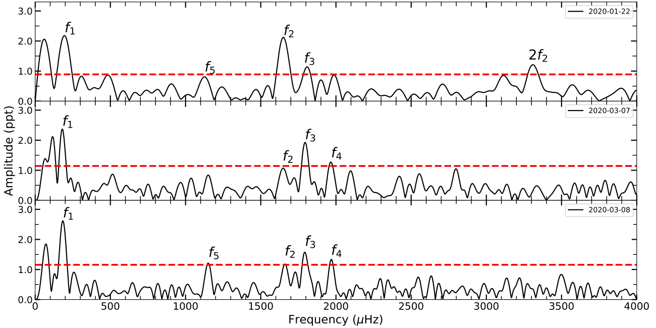
Figure 2. Fourier Transform for HE 1017–1352 for the SOAR observations for each of the three nights listed in Table 1. The 1/1000 False Alarm Probability detection limit was computed using random shuffling of the data. The identification for each peak is indicated (see Table 2). The FT corresponding to the concatenation of the three nights is depicted in the middle panel of Fig. 3.
