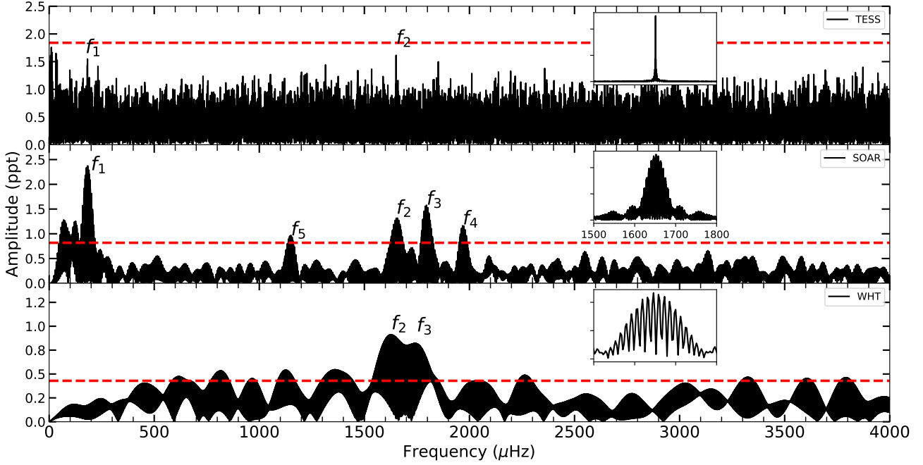
Figure 3. Fourier Transform for HE 1017–1352 based on observations with three different instruments. Observations from TESS satellite (top) span for 24 d in sector 9. The FT for SOAR telescope (middle) is computed from the concatenation of the three nights presented in the previous section. The FT for the WHT (bottom) was computed from the original data considering the concatenation of the two nights. The FAP (1/1000) detection limit (dashed line) was computed using random shuffling of the data. The identification for each peak is indicated (see Table 3 for details). The spectral window for each case is depicted as an inset plot, with a full-width at half maximum (FWHM) of 1 \mu\text{Hz} for TESS, 68 \mu\text{Hz} for SOAR and 280 \mu\text{Hz} for WHT. The x-axis is in \mu\text{Hz} and all inset plots are in the same scale as in the middle inset plot.
