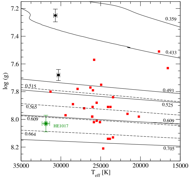
Figure 1. The position of the three hot DAV candidates and DBV white dwarf stars in the T_{\text{eff}} - \log g plane. Hot DAV candidates from Kurtz et al. (2008) are depicted with black circles, while HE 1017–1352 is depicted with a green circle. Known DBV stars are depicted with red squares. Some cooling tracks with thin hydrogen envelope (full line, Romero et al. 2019a) and helium pure atmospheres (dashed line, Althaus et al. 2009) are included for masses from 0.493 M_{\odot} to 0.705 M_{\odot} . Two low mass sequences with thick hydrogen envelopes, with stellar masses of 0.359 M_{\odot} and 0.433 M_{\odot} , are also included (Romero & Istrate 2019). Atmospheric parameters for HE 1017–1352 are taken from Gianninas et al. (2011), and for the other two hot DAV candidates are taken from Kepler et al. (2016).
