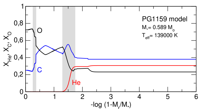
Fig. 24. Internal chemical profile of a template PG 1159 model ( M_{\star} = 0.589 M_{\odot} , T_{\text{eff}} = 139\,000 K) in terms of the outer fractional mass. The locations of the O/C and O/C/He chemical interfaces are indicated with gray regions.
