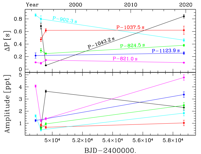
Fig. 11. Period variations (upper panels) and amplitudes (lower panels) of the six periods of RX J2117 that are common to the Vauclair et al. (2002) and TESS datasets. In the upper panel we have subtracted a constant value from each period in order to fit all periods within a narrow range.
