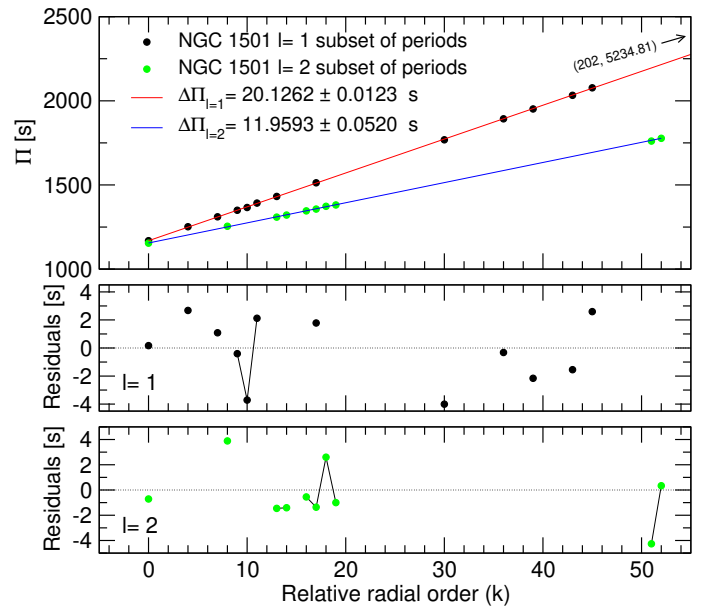
Fig. 20. Upper panel: Linear least-squares fits to the 14 dipole periods of NGC 1501 marked with an asterisk and the 9 quadrupole periods marked with two asterisks in Table 6. The derived period spacings from these fits are \Delta\Pi_{\ell=1} = 20.1262 \pm 0.0123 s and \Delta\Pi_{\ell=2} = 11.9593 \pm 0.0520 s, respectively. Middle panel: Residuals of the \ell = 1 period distribution relative to the dipole mean period spacing. Lower panel: Residuals of the \ell = 2 period distribution relative to the quadrupole mean period spacing. Modes with consecutive radial order are connected with a thin black line.
