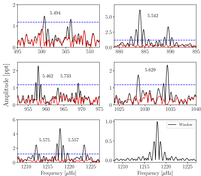
Fig. 4. Amplitude spectra of RX J2117 showing rotational multiplets. The panels present rotational splittings in different regions in the amplitude spectra with an average splitting \delta\nu = 5.570 \mu\text{Hz} . The last panel (bottom right) presents the window function of RX J2117 for the frequency 1217.872 \mu\text{Hz} . The horizontal dashed blue line shows the confidence level of 0.1% FAP. The red lines are residuals after extraction of the signals.
