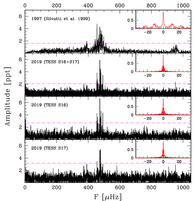
Fig. 5. Comparison between the amplitude spectrum of HS 2324 in 1997 (Silvotti et al. 1999) and 2019 ( TESS data). The detection threshold (dash-dotted magenta line) in 2019 is slightly higher (2.07 ppt with sector 16 and 17 together vs. 1.62 ppt in 1997), but the spectral window (red, upper right panels) is much cleaner. This partially explains the higher density of the peaks in 1997. The low level of noise below \sim 100 \mu\text{Hz} in 1997 is due to artificial filtering.
