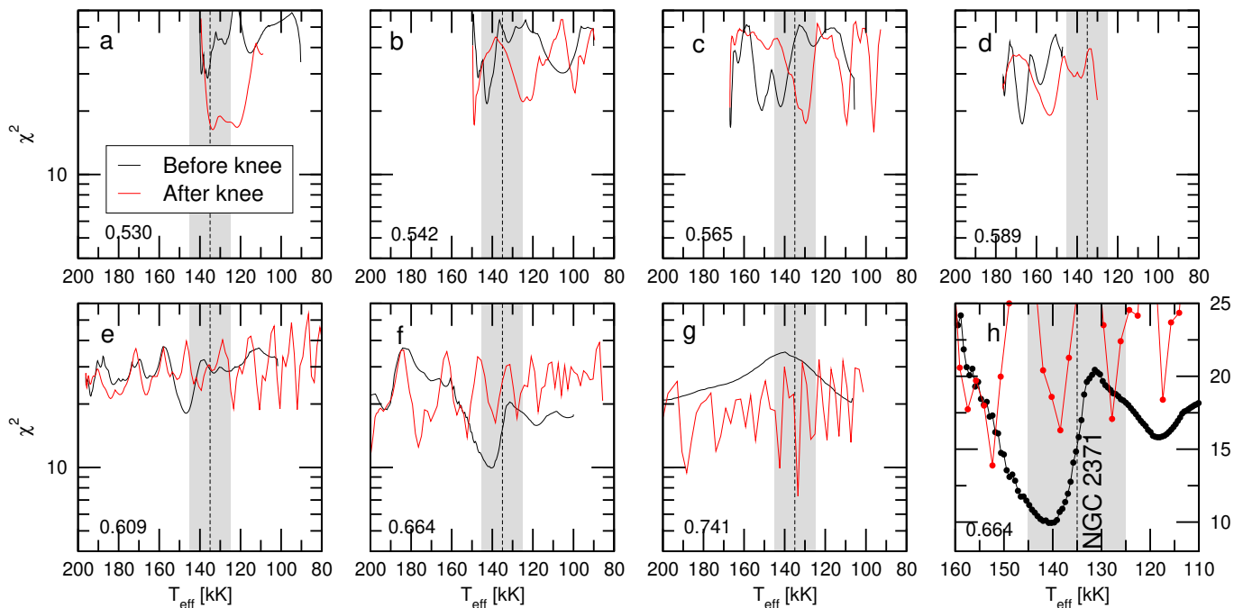
Fig. 33. Same as Fig. 26, but for NGC 2371. The minimum in panel f before the evolutionary knee (black curve) corresponds to M_{\star} = 0.664M_{\odot} . Panel h is a zoom of the region with the strong minimum seen in panel f; the y-axis scale is linear in this case. The vertical dashed line is the spectroscopic T_{\text{eff}} of NGC 2371 (135 kK), and the gray zone depicts its uncertainties ( \pm 10 kK).
