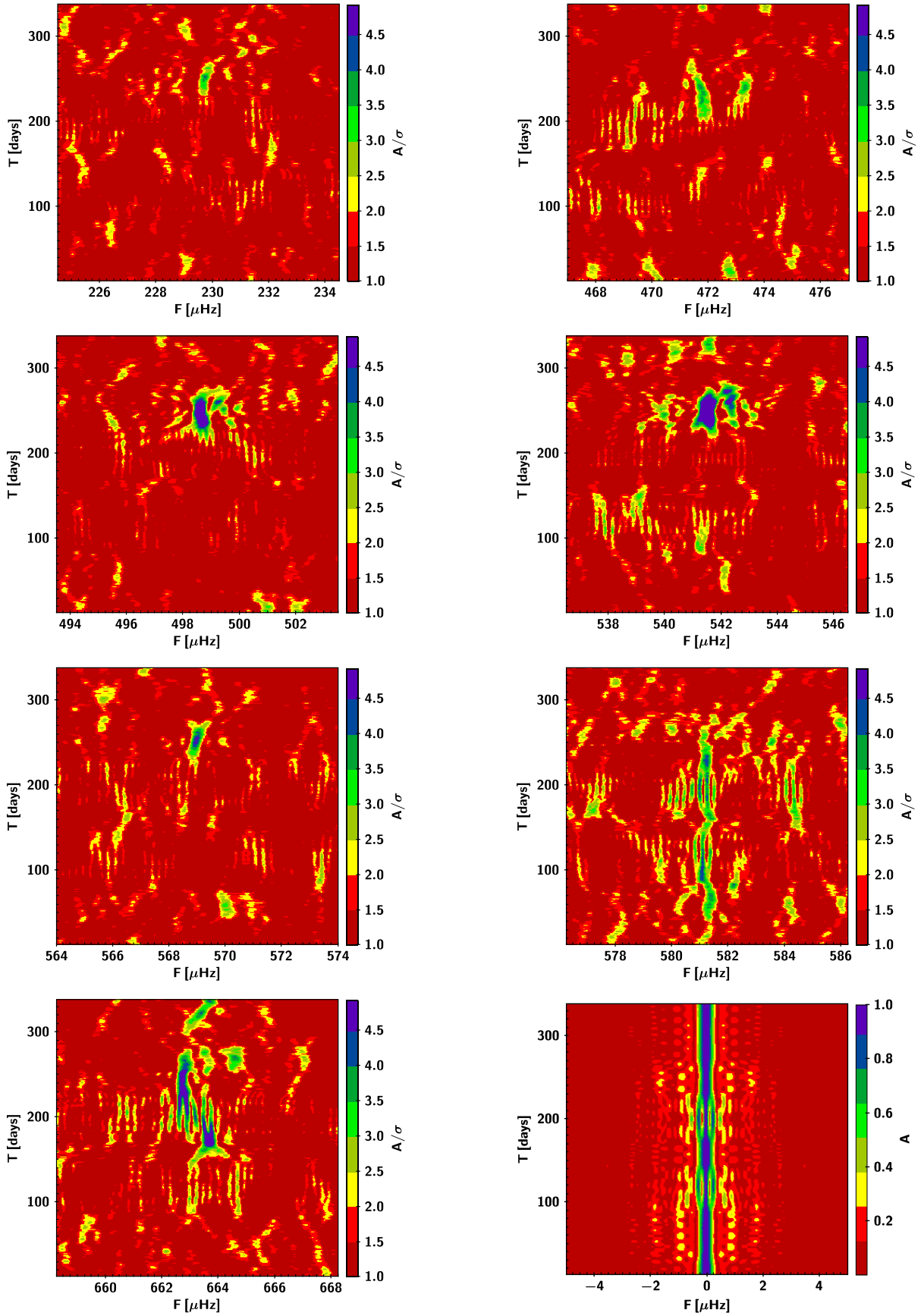
Fig. 7. Panels 1-7: Sliding FT of K 1–16 centered on the peaks at \sim 229.7 , \sim 471.7 , \sim 498.7 , \sim 541.6 , \sim 569.0 , \sim 581.3 , and \sim 663.0 \mu\text{Hz} . The color-coded amplitudes are given in \sigma units, i.e., amplitude divided by the mean noise of each FT. The oscillations are not stable over the course of the TESS observations, and in the first \approx 200 days (up to Sector 22) some of the modes are absent. Panel 8: Sliding WF obtained using a single sinusoid of constant frequency and constant amplitude of one, without any noise. The frequency scale is the same in all panels. See text for more details on sFT and sWF computations.
