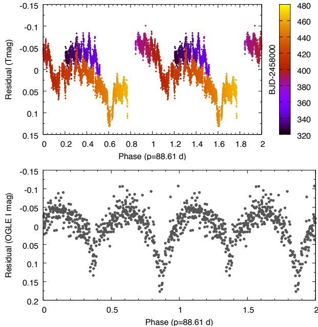
Figure 10. Residual light curves of OGLE LMC-T2CEP-023 folded with the orbital period of the companion star. Upper panel: TESS data. Lower panel: OGLE I-band data.
