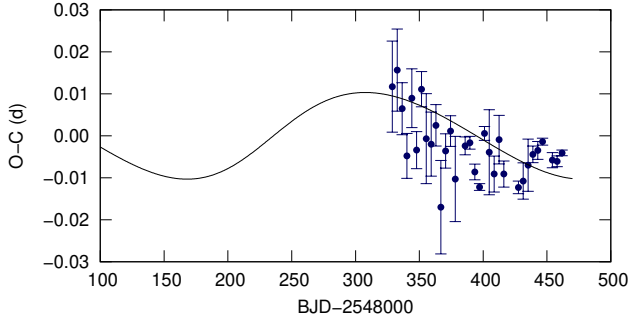
Figure 11. The O–C diagram of OGLE LMC-CEP-227 plotted on the expected LiTE variation caused by the known companion star.
