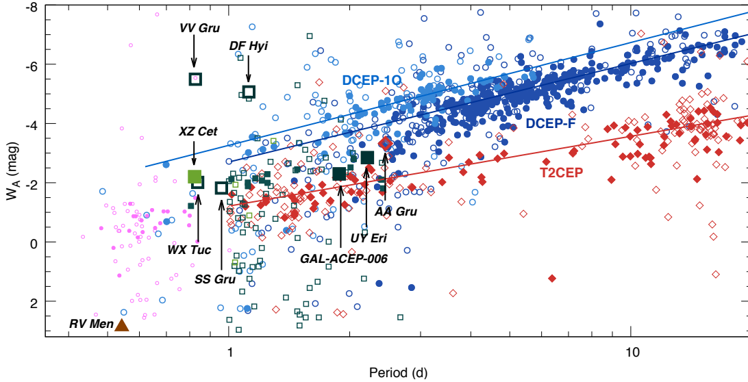
Figure 15. P-L relation of Milky Way Cepheids using absolute Wesenheit magnitudes (Ripepi et al. 2019). Filled symbols indicate stars with parallax errors below 20%. Our target stars are indicated with large symbols. Colours are the same as in Fig. 9. Pink: stars reclassified as RRAB. Lines: P-L relations calculated by Ripepi et al. (2019) for each class, slopes have been fixed to LMC Cepheids.
