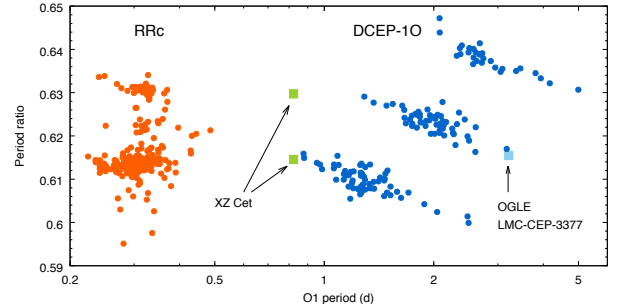
Figure 6. The Petersen diagram of non-radial modes in overtone RR Lyrae (orange) stars and Cepheids (blue). (Sources: Netzel et al. (2015a,b); Netzel & Smolec (2019); Moskalik et al. (2015); Jurcsik et al. (2015); Smolec & Śniegowska (2016); Moskalik & Kołaczowski (2009)). The new discoveries, XZ Cet and OGLE LMC-CEP-3377 (see Sect. 3.3.4) are marked with squares.
