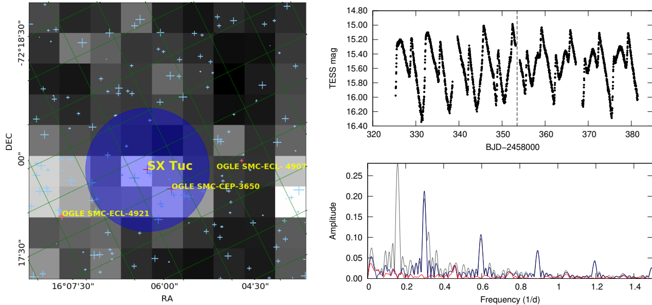
Figure 13. Left: image cutout of SX Tuc and OGLE SMC-CEP-3650 within the aperture. Upper right: composite light curve. Lower right: composite Fourier spectrum (SX Tuc in blue, OGLE SMC-CEP-3650 in grey, residual in red.)
