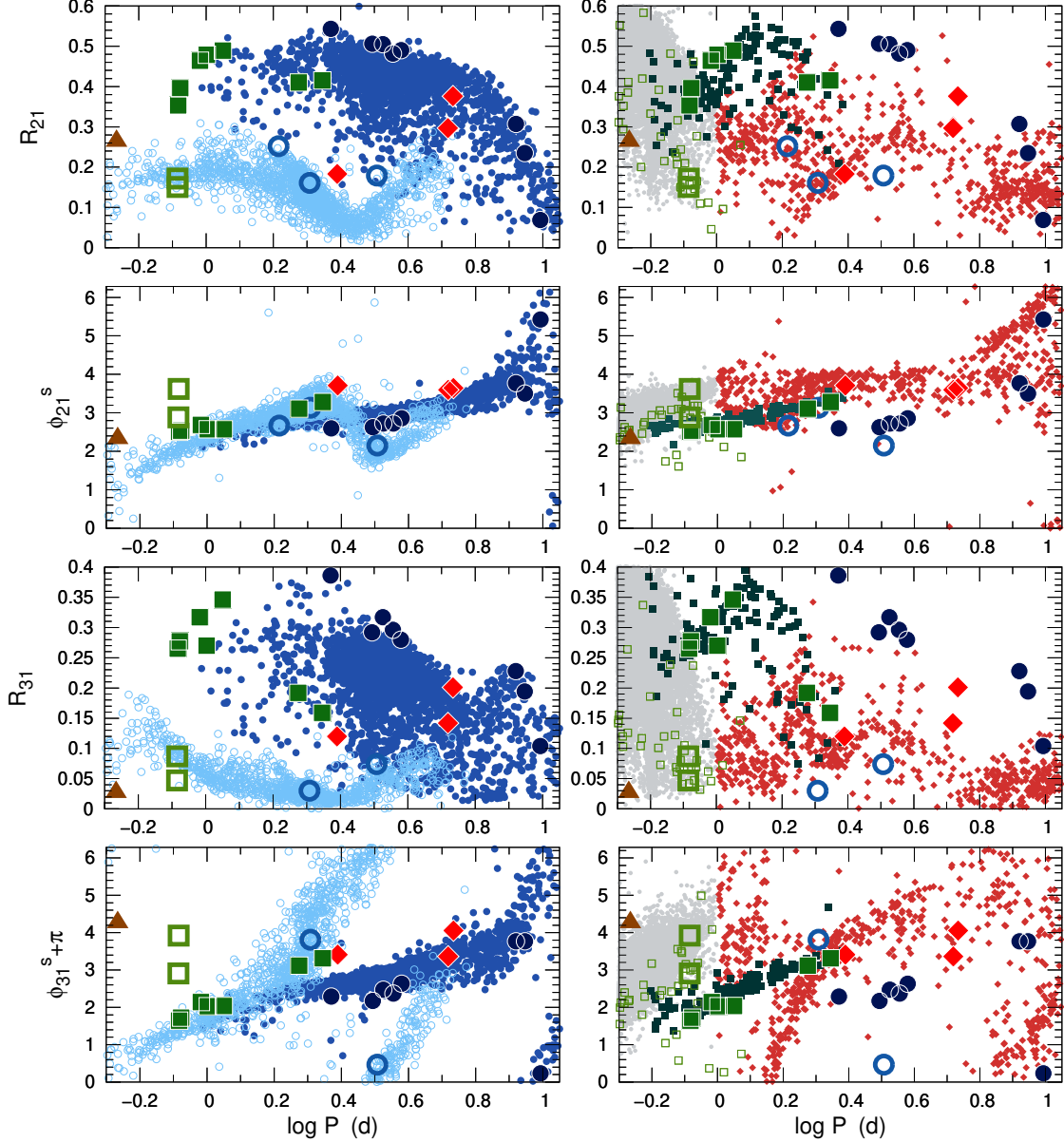
Figure 14. Relative Fourier parameters R_{21} , \phi_{21}^s , R_{31} and \phi_{31}^s + \pi against the pulsation periods. Large symbols are our targets with colours corresponding to the most likely classes (blue dots: DCEP-F, light blue circles: DCEP-10, green filled squares: ACEP-F, light green open squares: ACEP-10, red diamonds: T2CEP). Small symbols are the OGLE-IV Fourier parameters for Classical Cepheids (left panels), and Type II and anomalous Cepheids (right panels). We also included RRab stars with grey dots in the latter. RV Men is the brown triangle at the short-period end, at the edge of the RRab locus.
