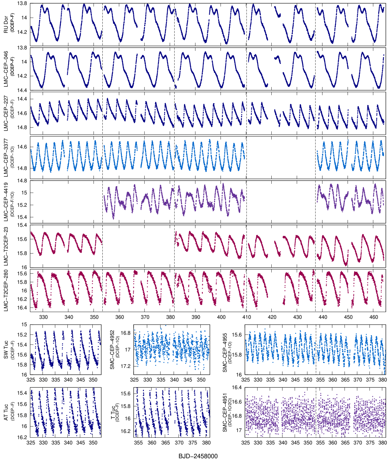
Figure 9. FITSH light curves of Cepheids in the Magellanic System. Subtypes are marked in different colours: DCEP-F (dark blue), DCEP-10 (light blue), double-mode stars (purple), T2CEP (dark red). Dashed vertical lines divide the different Sectors.
