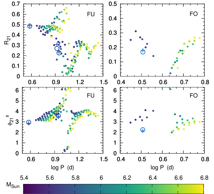
Figure 16. Theoretical Fourier parameters for LMC Cepheids at different masses, for LMC-like chemical composition ( Y=0.25 , Z=0.008 ). Observed TESS (plus) and OGLE I -band (circle) Fourier parameters of OGLE LMC-CEP-227, RU Dor, OGLE LMC-CEP-046 and OGLE LMC-CEP-3377 are indicated.
