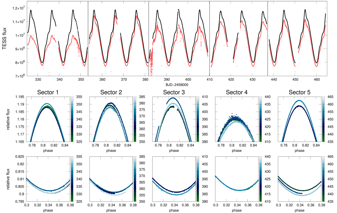
Figure 3. Short cadence photometry of \beta Dor from the SPOC pixel mask (red) and our custom pixel mask (black). Lower panels show the differences in the maxima and minima of the custom light curves when folded with the pulsation period, for each Sector. Colours indicate the progress of time (BJD-2458000) in days.
