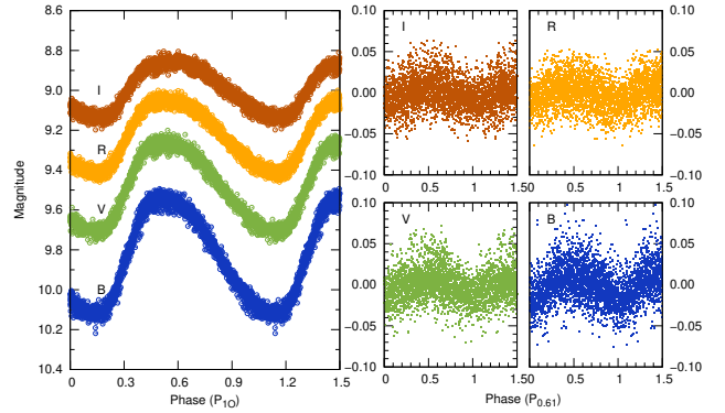
Figure 7. Ground-based measurements of XZ Cet in BVRI bands. Left: phase curves folded with P_{1\text{O}}=0.82315 days. Right: residual phase curves folded with P_{0.61}=0.50479 days.
