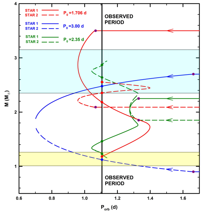
Figure 11. The evolution of the masses of the two components of the primordial binary as a function of orbital period is illustrated. Arrows superposed on the curves denote the direction of increasing age (i.e., the direction in which the component is evolving). Star 1 is always losing mass while Star 2 is accreting mass. The colour scheme for the three cases shown in Fig. 10 is repeated here. The initial orbital period for each case is also labeled (upper left) and the observed orbital period ( 1.1057 d) is denoted by a vertical black bar. The solid dots of the same colour as the curves indicate the points that could be possible solutions for the properties of TIC 63328020. The cyan-shaded region represents the approximate range of possible masses of the current primary based on the analysis presented in Table 6 (columns 3 and 4). The yellow-shaded region corresponds to the possible range of masses for the current secondary. All of the curves terminate when both stars have simultaneously filled their Roche lobes.
