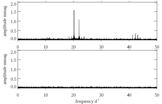
Figure 2. Top: The amplitude spectrum of the high pass data. There is a frequency septuplet centred on \nu_1 = 21.09533 \text{ c/d} , and a quintuplet centred on 2\nu_1 . The reason there are two high amplitude first sidelobes about an almost zero amplitude mode pulsation frequency is that we are seeing this pulsation inclined by 90^\circ to the orbital axis, which itself is near to i = 90^\circ , thus giving two pulsation amplitude maxima per orbit.
