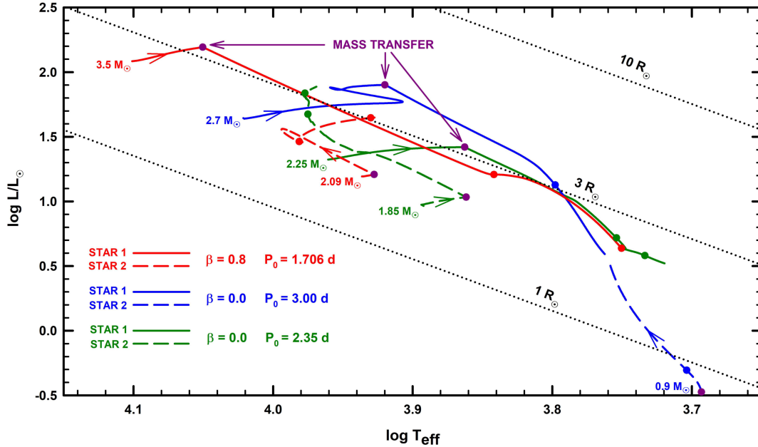
Figure 10. Representative tracks of three distinctly different primordial binary evolutions leading to the formation of TIC 63328020 are shown in the HR diagram. The evolution of the more massive component of the primordial binary (Star 1) is denoted by a solid curve and the evolution of its less massive companion (Star 2) is represented by a dashed curve. Arrows superposed on the curves denote the direction of increasing age (i.e., the direction in which the component is evolving). Different colours are used to denote each pair of the components of the primordial binary. Each component initially starts evolving from the ZAMS and those masses for all three cases are labelled. The red tracks correspond to a binary that experiences highly non-conservative mass-transfer ( \beta = 0.8 ), while the blue and green tracks assume fully conservative mass-transfer. The solid dots of the same colour as the track indicate the points in the evolution when the orbital period matches the observed value (1.1057 d). The purple dots indicate the points for which (rapid) thermal-timescale mass-transfer is first initiated. All of the tracks terminate when both stars have simultaneously fill their Roche lobes.
