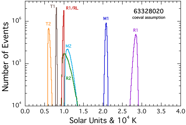
Figure 7. Posterior distributions from the MCMC analysis for the case where the stars are assumed to be coeval and without any prior mass exchange. For M_1 , M_2 , R_1 , and R_2 , the x axis is labeled in solar units, while T_1 and T_2 are in units of 10^4 K, and R_1/R_L is dimensionless. Note, in particular, that R_2 is small compared to R_1 .
