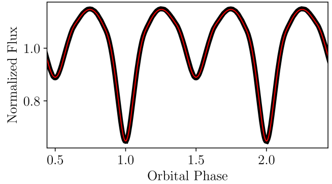
Figure 9. The model phoebe2 light curve (red) on the observations (black). A sinusoidal component of amplitude 0.4 per cent was removed from the TESS light curve to equalize the two ELV maxima before performing the fit (see text for details).
