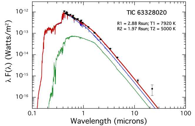
Figure 4. SED data and model for TIC 63328020 spanning the blue to 20 micron region for the non-coeval case described in Section 3.3.2. The continuous green, blue and red curves represent the contributions of the secondary, the primary, and the total system flux, respectively.
