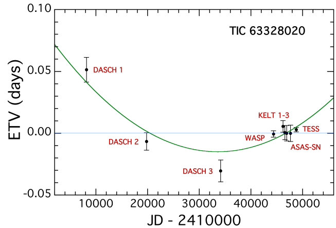
Figure 5. Long-term eclipse timing variations for TIC 63328020. The data sets used are marked in red labels and include TESS , ASAS-SN , WASP , KELT , and DASCH (see Table 3 for references). The latter two data sets have each been divided into three subsets of 30 years and \sim 10 months, respectively. The time intervals covered by each data set and the references are given in Table 3. The error bars plotted here and used in the long-term fit are scaled from the actual uncertainties in Table 3, \sigma_0 , to be \sigma \equiv 0.1\sqrt{\sigma_0} . We did this so as not to allow the tiny error bars of the modern-epoch points to totally dominate the determination of the long-term period or its derivative. The green curve is a fit to linear and quadratic terms. See Table 4 for results.
