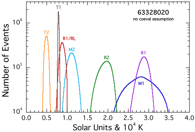
Figure 8. Posterior distributions from the MCMC analysis for the case where the stars are not assumed to be coeval and without any prior mass exchange. The axis labeling is the same as in Fig. 8. Note, that the distributions are broader than in Fig. 7, and M_1 has gotten larger, as has R_2 .
