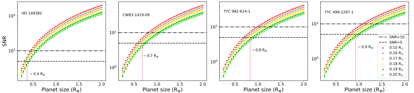
Fig. 6. Performances of CHEOPS on hot subdwarfs. From left to right panel: HD 149382 ( G=8.9 ), CW83-1419-09 ( G=12.0 ), TYC 982-614-1 ( G=12.2 ), and TYC 499-2297-1 ( G=12.6 ). The minimum planet size for \text{SNR}=5 and a 0.18 R_{\odot} host is indicated next to the red vertical line.
