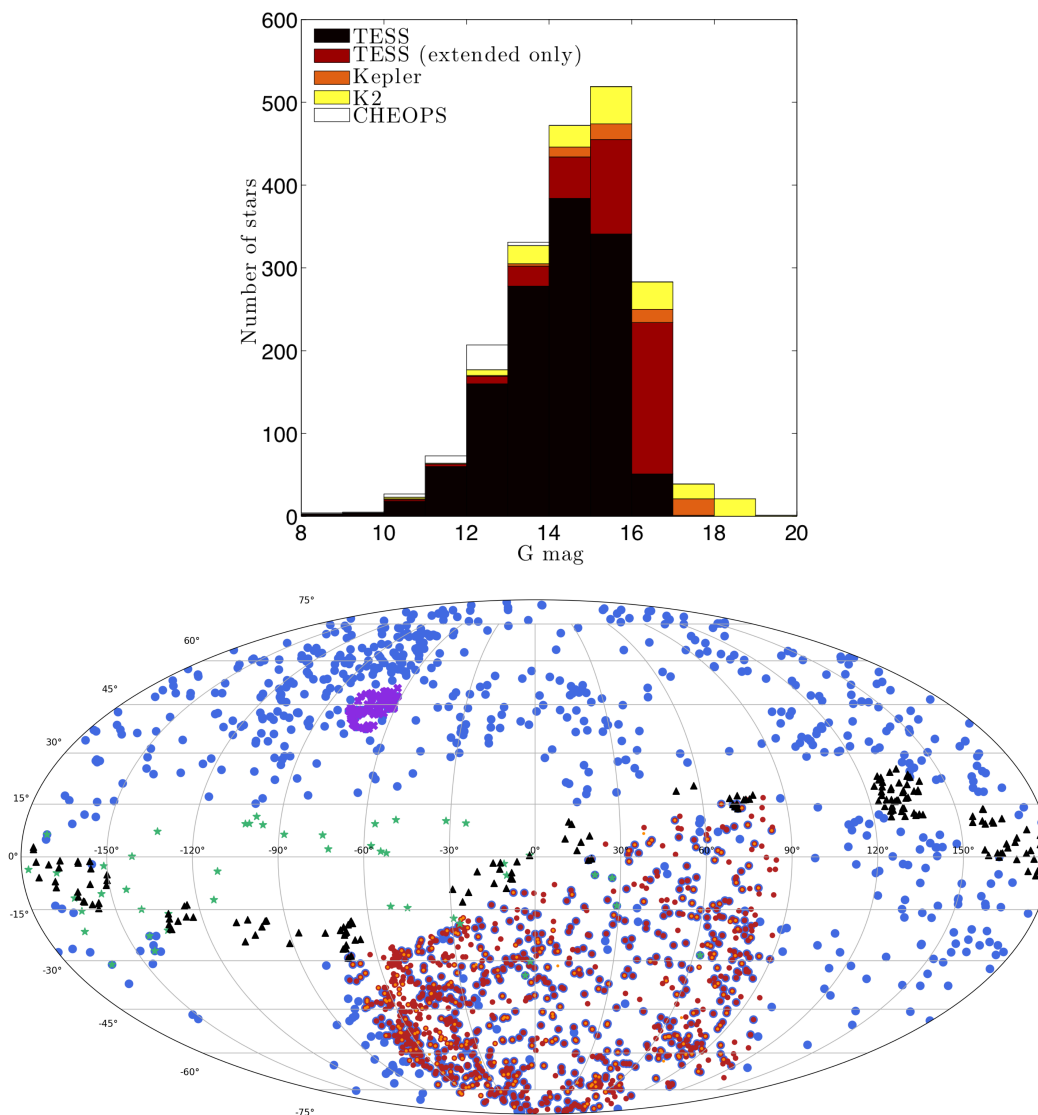
Fig. 1. Top: Number of hot subdwarfs observed by Kepler, K2, TESS (hot subdwarfs observed in primary mission, which are all reobserved in the extended mission), TESS extended only (new hot subdwarfs observed only in the extended mission), and CHEOPS (as of December 19, 2020) per G magnitude bin. Bottom: Celestial distribution of these hot subdwarfs: TESS primary mission (blue dots), TESS extended mission 2-min and 20 s (red and dark orange dots), Kepler (purple crosses), K2 (black triangles), and CHEOPS (green stars).
