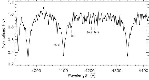
Figure B2. SAAO spectrum of TIC 294266638. Lines of Sr and Eu are noted as being pronounced in this star, leading to the classification of Ap SrEu.
