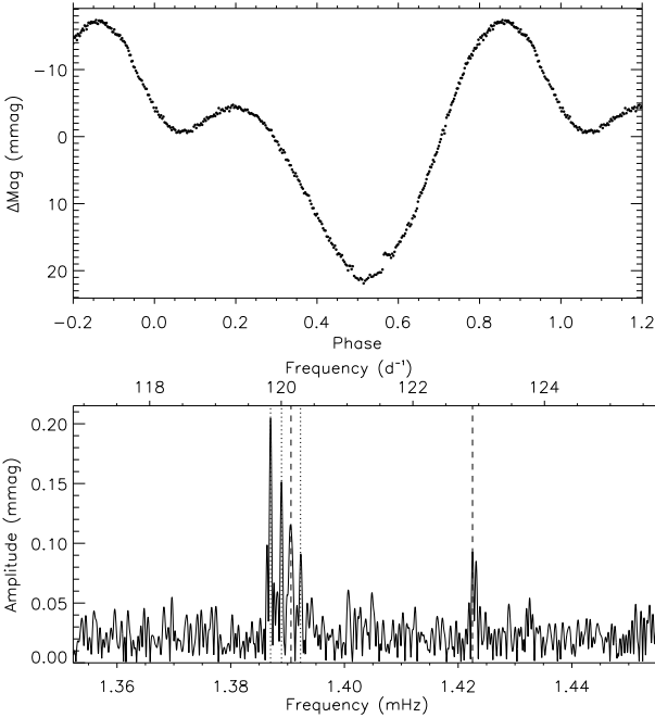
Figure 40. Top: light curve of TIC 363716787 phased on its rotation period of 5.9660 d. Bottom: amplitude spectrum of the light curve of TIC 363716787. The dashed lines represents the two extracted modes, while the dotted lines show the multiplet components.
