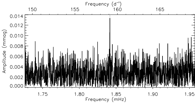
Figure 31. The amplitude spectrum of TIC 189996908. The low S/N peak detection agrees with that found in spectroscopic observations.
