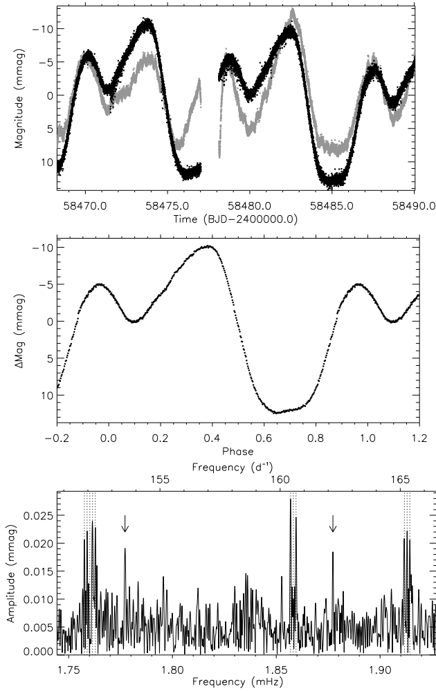
Figure 4. Top: comparison of the PDC_SAP (grey) and SAP (black) light curves for TIC 176516923. Middle: SAP light curve phase folded on the derived rotation period of 8.7821 d. Bottom: amplitude spectrum of the PDC_SAP light curve showing the pulsational variability. The vertical dotted lines indicate the multiplet components, with the arrows indicating possible further modes.
