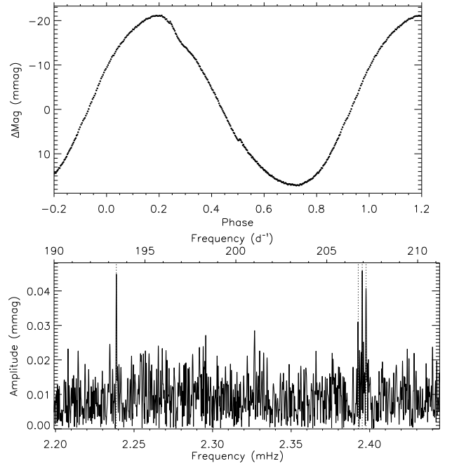
Figure 5. Top: the light curve of TIC 178575480 phase folded on the derived rotation period of 8.7821 d. Bottom: amplitude spectrum of the light curve showing the pulsational variability. The vertical dotted lines indicate the pulsation modes and the multiplet components of the high-frequency triplet.
