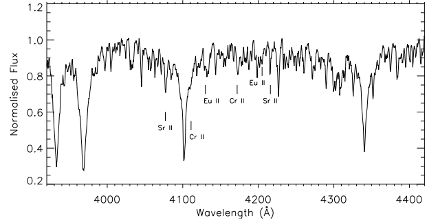
Figure B7. The SAAO spectrum of TIC 49818005 with lines of Sr, Eu and Cr identified. We provide a spectral classification of Fp SrEu(Cr).
