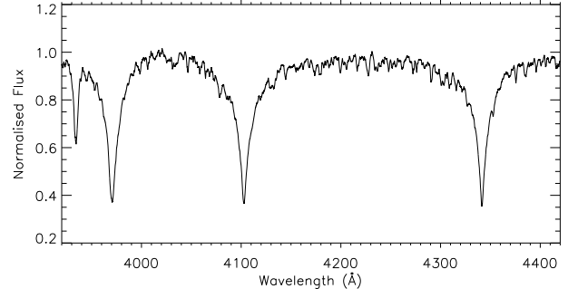
Figure B11. The SAAO spectrum of TIC 3814749 showing the lack of strong chemical peculiarities in this star.
