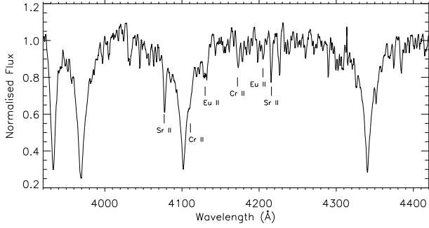
Figure B3. The SAAO spectrum of TIC 356088697 with lines of Sr, Eu and Cr identified. We refine the spectral classification to Ap SrEuCr.
