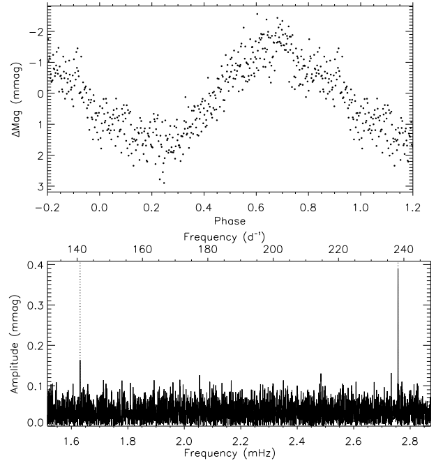
Figure 47. Top: phase folded light curve of TIC 3814749, phased on a period of 1.689 d. Bottom: the two high frequency pulsation modes found in this star, as marked by dotted lines.
