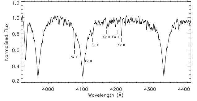
Figure B5. The SAAO spectrum of TIC 17676722 with lines of Sr, Eu and Cr identified. We refine the spectral classification to Ap SrEuCr.
