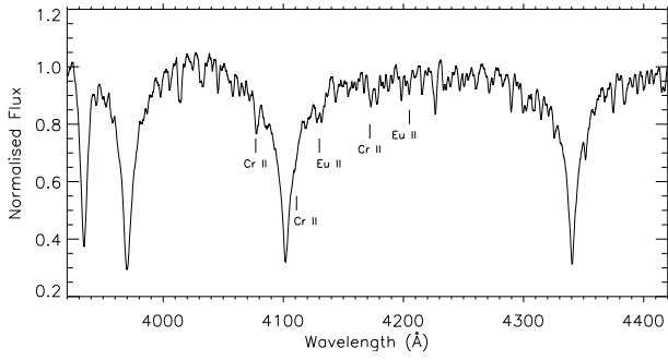
Figure B10. The SAAO spectrum of TIC 350146296 with which we deduce a classification of F0p EuCr.
