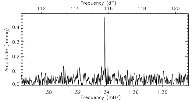
Figure 12. Amplitude spectrum showing the pulsation mode in TIC 466260580.
