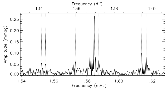
Figure 25. The pulsation signatures seen in TIC 136842396. The vertical dotted lines represent the extracted peaks, all of which are, in their groups, separated by integer values of the rotation frequency.
