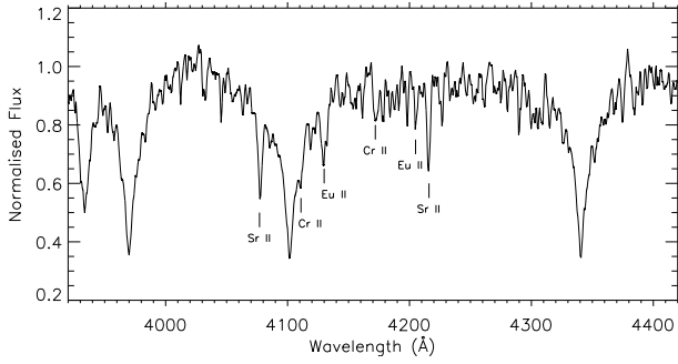
Figure B9. The SAAO spectrum of TIC 156886111 with which we deduce a classification of Ap SrEuCr.
