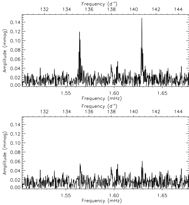
Figure 6. Pulsation modes in TIC 294266638. After removing the obvious pulsations, excess power is remaining which is suggestive of frequency variability.
