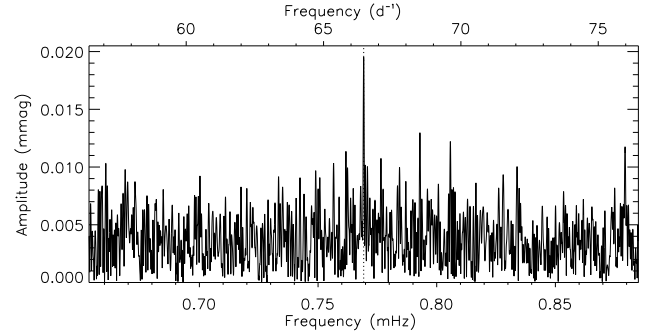
Figure 19. Amplitude spectrum of TIC 6118924.
