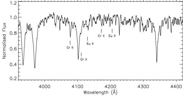
Figure B8. The SAAO spectrum of TIC 152808505. We provide a spectral classification of Fp EuCr.
