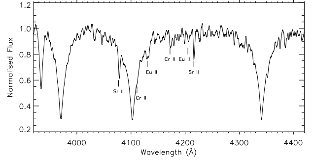
Figure B6. The SAAO spectrum of TIC 41259805 with lines of Sr, Eu and Cr identified. We refine the spectral classification to Ap SrEu(Cr).
