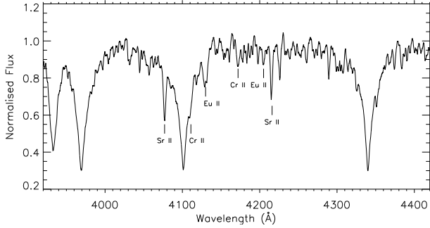
Figure B4. The SAAO spectrum of TIC 12968953 with lines of Sr, Eu and Cr identified. We refine the spectral classification to Ap SrEuCr.
