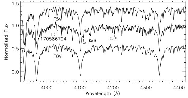
Figure B1. SAAO spectrum of TIC 170586794 (centre), with stars of spectral class F5V (above) and F0V (below) for comparison. Lines of Eu and Cr are enhanced in this star, leading to the classification of F5VpEuCr.
