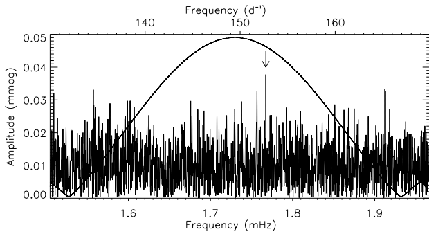
Figure 23. The amplitude spectrum of TIC 93522454 in the frequency region of interest. We see no clear indication of pulsation, but mark with an arrow a possible signature. The smooth solid curve represents the shape of the peak used by Kochukhov et al. (2013) to provide a pulsation frequency of 1.73 mHz ( 149.47 \text{ d}^{-1} ), demonstrating the broad frequency range where the mode may be found.
