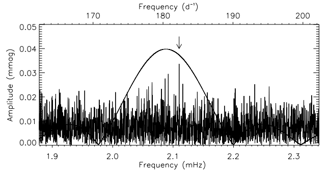
Figure 30. The amplitude spectrum of TIC 173372645. The arrow indicated a potential peak, whereas the broad smooth curve represents the shape of the peak used by Kurtz et al. (2006b) to identify the pulsation mode in this star.
