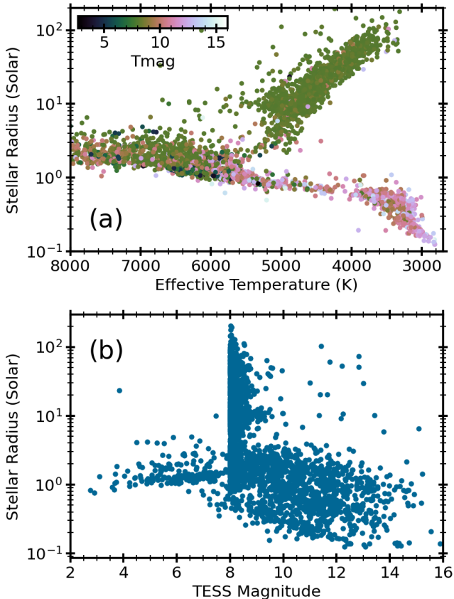
Figure 1. Panel (a): Stellar radius versus effective temperature of the \approx 4400 unique stars with T_{\text{eff}} < 8000 K observed with TESS 20-second cadence observations during the first 10 sectors of the extended mission, color-coded by TESS magnitude T (capped at T < 16 mag). Panel (b): Stellar radius versus TESS magnitude for the sample shown in panel (a). Compact stars (such as hot subdwarfs and white dwarfs) are excluded from both panels.
