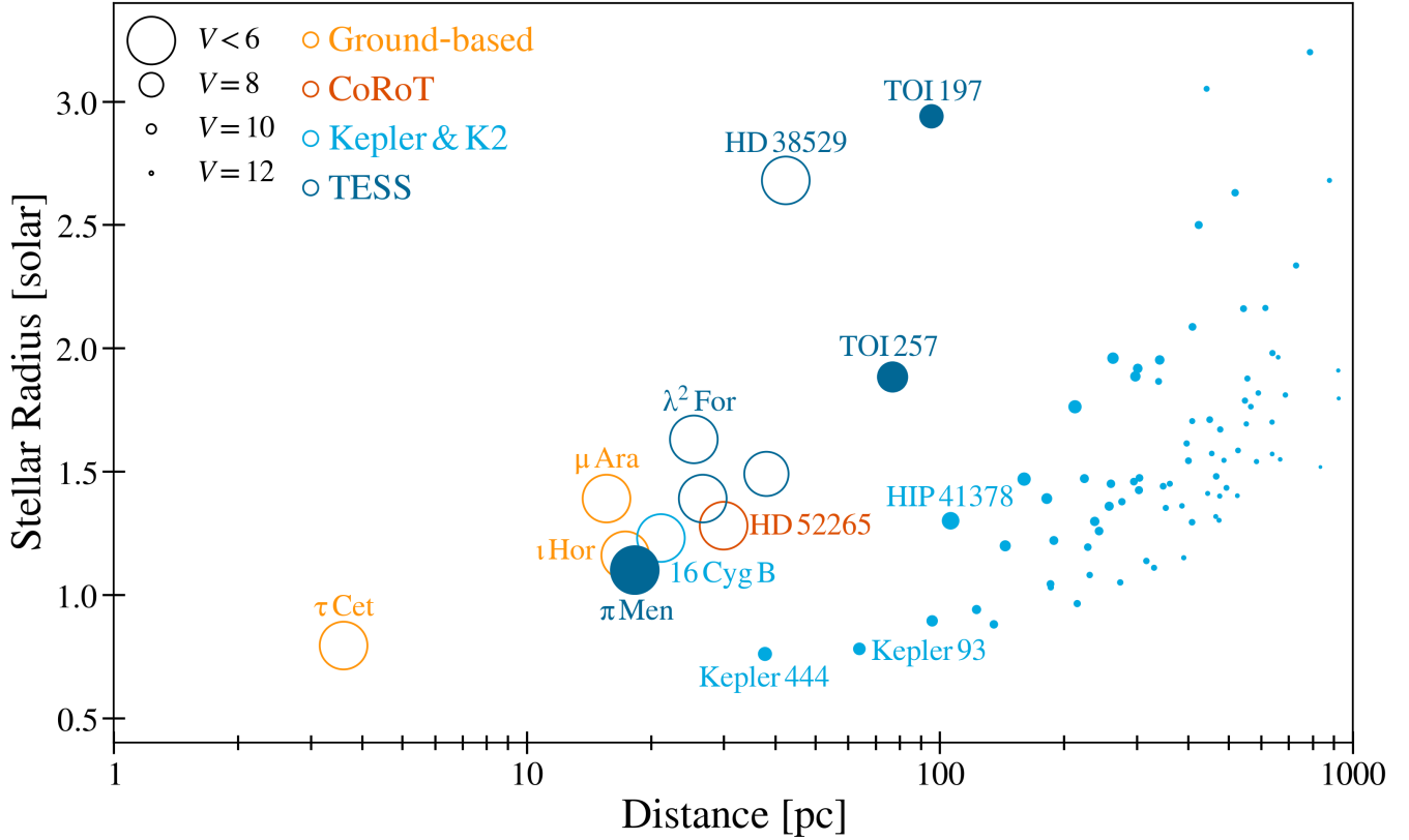
Figure 9. Stellar radius versus distance for the current population of asteroseismic host stars (excluding evolved stars with R > 3.5R_{\odot} ) with confirmed \Delta\nu measurements from ground-based radial velocity observations (orange), CoRoT (red), Kepler/K2 (light blue) and TESS (dark blue). Markers are sized by their visual magnitude and filled symbols show systems with known transiting planets. \pi Men is now the closest and brightest star with a transiting planet for which detailed asteroseismic modeling is possible. Label references (in order of proximity) – \tau Cet (Teixeira et al. 2009), \mu Ara (Bouchy et al. 2005), \iota Hor (Vauclair et al. 2008), \pi Men (this work), 16 Cyg B (Metcalfe et al. 2012), \lambda^2 For (Nielsen et al. 2020), HD 52265 (Lebreton 2012; Escobar et al. 2012; Lebreton & Goupil 2014), Kepler-444 (Campante et al. 2015), HD 38529 (Ball et al. 2020), Kepler-93 (Ballard et al. 2014), TOI-257 (Addison et al. 2021), TOI-197 (Huber et al. 2019) and HIP 41378 (Vanderburg et al. 2016; Becker et al. 2019; Lund et al. 2019).
