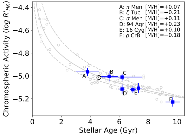
Figure 8. Chromospheric activity versus stellar age for a sample of spectroscopic solar twins from Lorenzo-Oliveira et al. (2018) with ages determined from isochrone fitting (grey circles) and bright stars with asteroseismic ages from TESS and Kepler (blue symbols).
