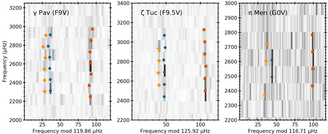
Figure 7. Échelle diagrams for \gamma Pav (left), \zeta Tuc (middle) and \pi Men (right) using granulation-background corrected power spectra. Different symbols denote radial modes (circles), dipole modes (squares) and quadrupole modes (diamonds). Error bars are smaller than symbol sizes in all cases.
