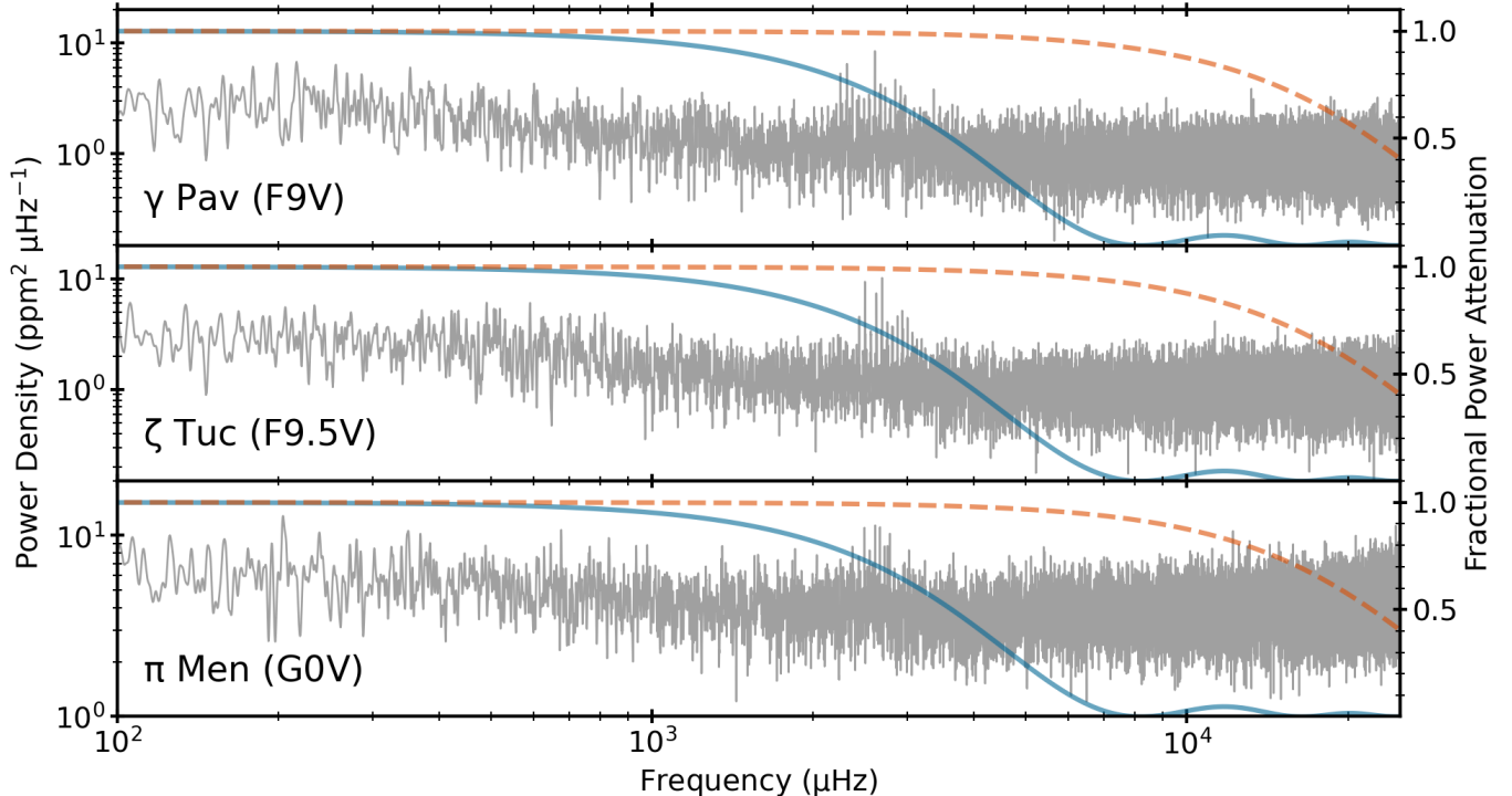
Figure 6. Power density spectra on a log-log scale using the 20-second cadence light curves for \gamma Pav (top), \zeta Tuc (middle) and \pi Men (bottom). Each power spectrum was smoothed with a Gaussian with a FWHM of 1 \mu\text{Hz} . Lines show the fractional power attenuation as given on the right-hand y-axis for 2-minute cadence sampling (solid lines) and 20-second cadence sampling (dashed lines) in each panel.
