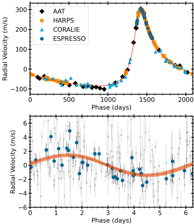
Figure 11. Radial velocity data phase-folded to the orbital periods of \pi Men b (top panel) and \pi Men c (bottom panel). The bottom panel shows all instruments except for ESPRESSO in grey. Each panel shows the RV data with contribution from the other planet removed.
