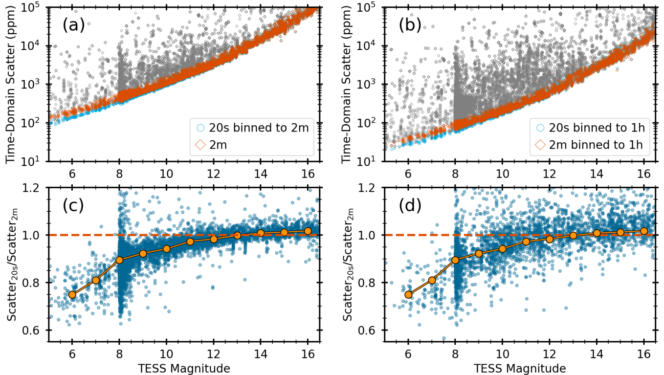
Figure 2. Panel (a): Time-domain scatter as a function of TESS magnitude for stars observed in 20-second cadence between Sectors 27 to 36. Symbols show 20-second light curves binned to 2-minute cadence (cyan circles) and original 2-minute light curves (red diamonds) for each sector. Grey points mark stars likely dominated by stellar variability (see text). Panel (b): Same as panel (a) but binning light curves to 1-hour cadence. Panel (c): Ratio of the time-domain scatter for the two datasets shown in panel (a), retaining only stars not dominated by stellar variability (i.e. each point in panel c is the ratio of a cyan and red point in panel a). The dashed line marks unity and orange circles show median bins. Panel (d): Same as panel (c) but for the binned light curves shown in panel (b).
