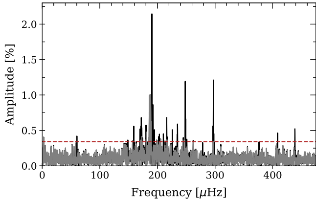
Figure 3. Periodogram of the GD 278 TESS dataset in black. In grey is the periodogram of the same data after being prewhitened by the frequencies in Table 1. The red dashed line represents the 99.9% False Alarm Probability threshold, which we estimate to be 0.34%. Peaks above this line have a <0.1\% chance of being caused by random noise, and thus represent intrinsic signals from the star.
