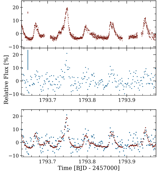
Figure 4. Top: Simultaneous McDonald (15-s exposures) and TESS (120-s exposures) observations of GD 278, captured on 2019 November 8. A representative error bar is shown in the top left corner of each plot. Bottom: Both data sets overplotted. The McDonald data (red) have been resampled to the same 2-min cadence as the TESS data (blue) in the bottom plot.
