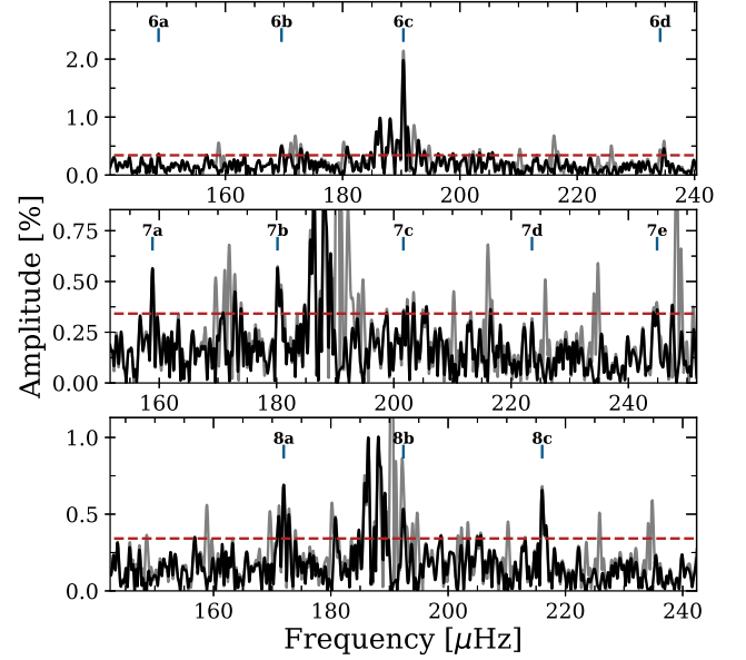
Figure 6. Similar to Figure 5, except for the three \ell = 2 mode splittings identified within the GD 278 TESS periodogram and listed in Table 2. Blue tick marks indicate the frequencies that we propose form the rotationally split multiplets, also consistent with 0.5-d rotation.
