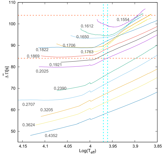
Figure 10. Evolution of the mean period spacing for \ell = 1 modes as a function of effective temperature for various cooling models of ELM white dwarfs (Calcaferro et al. 2018) with masses between 0.15 - 0.44 M_{\odot} and canonically thick hydrogen envelopes. Plotted over these models are the two possible values of the constant period spacing for GD 278 found from our analysis (roughly 84 s and 104 s, horizontal lines), as well as bounds from the spectroscopic effective temperature and uncertainties (vertical cyan lines). For white dwarfs < 0.2 M_{\odot} we expect mean period spacings \Delta\Pi > 80 s.
