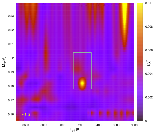
Figure 7. Map of the inverse of the quality function ( 1/\chi^2 ) as a function of the stellar mass ( M_\star ) and effective temperature ( T_{\text{eff}} ), considering the eight m = 0 modes identified in bold in Table 2. Each point on the map corresponds to a hydrogen envelope mass ( M_H ) that maximizes the value of 1/\chi^2 . The green box represents the GD 278 spectroscopic mass and effective temperature, and the corresponding 1\sigma uncertainties, from Brown et al. (2020).
