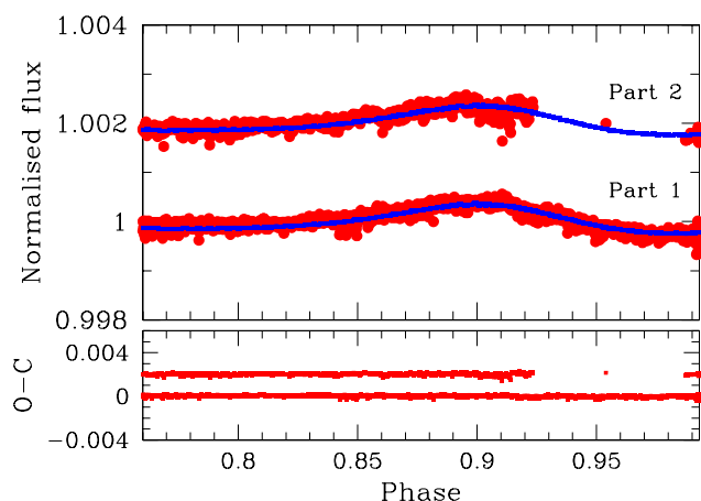
Fig. 11: Same as Fig. 10, but in the portion of the light curve preceding the primary minimum. Brightening due to the proximity effect (reflection) is well below 1 milli-mag level, and is detected only thanks to the superb high-precision space photometry acquired by the TESS mission. The light curves and best fit for the Part 2 are arbitrary shifted upwards for better visibility.
