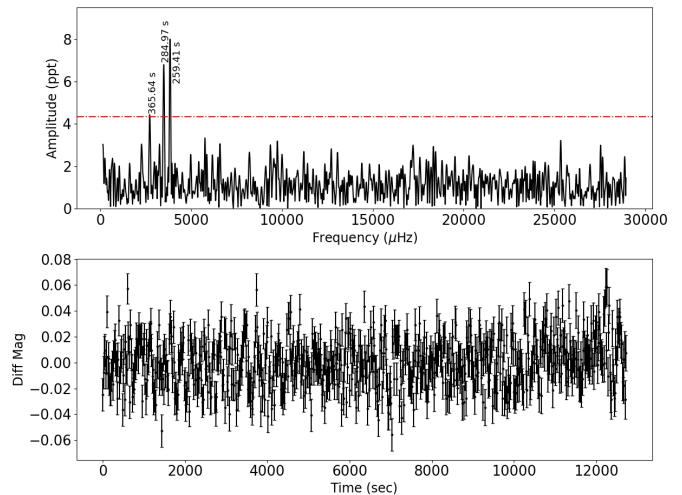
Figure 5. FT and light curve, top and bottom panel respectively, for TIC 20976653 based on data obtained from the Pico dos Dias observatory on 2020-06-14. The data spans for 3.4 h, with an integration time of 17 s.
