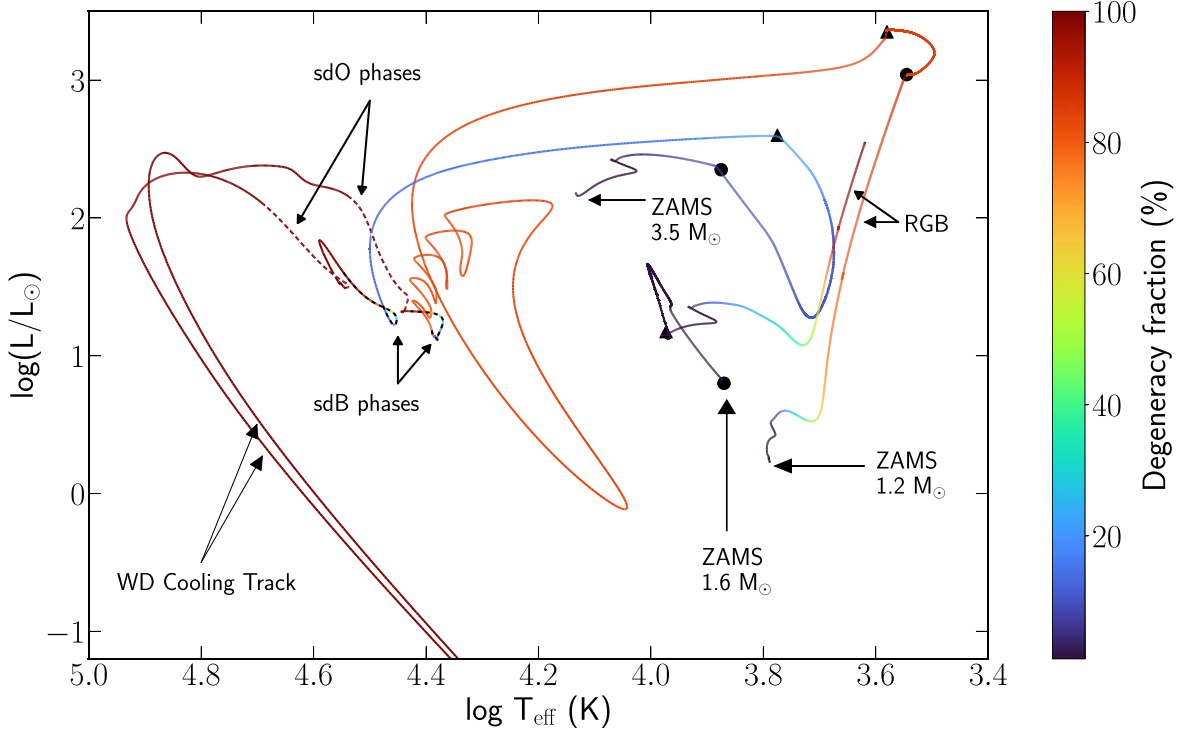
Figure 9. Formation and evolution of representative intermediate-period and long-period sdBs from the zero-age main sequence (ZAMS) to the final WD cooling stage in the H-R diagram. The solid lines denote the evolutionary tracks and the corresponding colors (as given by the color bar) indicate the percentage of the combined ideal gas and electron degeneracy pressures that is solely due to degeneracy (evaluated at the center). A filled circle denotes the start of a mass-transfer phase and a triangle denotes the end of that phase. The ZAMS progenitor star for the intermediate-period case has a mass of 3.5 M_{\odot} and an approximately solar metallicity ( Z = 0.02 ). Mass transfer is initiated in the Hertzsprung gap and continues as the progenitor ascends the red giant branch (denoted as RGB). Mass transfer ceases once its mass is reduced to 0.47 M_{\odot} , and this stripped core evolves along the horizontal branch until it reaches the sdB phase. This phase (annotated and denoted by the black dashed lines overlaid on the evolution curves) persists for almost 80 Myr before the hot subdwarf subsequently evolves through the sdO phase (distinguished by the brown dashed lines) for an additional 40 Myr. The evolution of the companion star is also shown; its initial mass is 1.6 M_{\odot} , and it undergoes a phase of rapid accretion before it reaches thermal equilibrium (after mass transfer has ceased) and evolves normally as a 1.9 M_{\odot} star. The star ascends the RGB, and the evolution is halted once the star is large enough to fill its Roche lobe. The progenitor star of the long-period sdB binary has a primordial mass of 1.2 M_{\odot} and evolves up the RGB until it is close to its tip, at which point it starts to lose mass rapidly. After a series of thermal adjustments, it enters the sdB phase, which persists for \approx 75 Myr (annotated); for reasons of clarity, the evolution of its companion is not shown. Note that the observable properties of the sdBs in both the intermediate- and long-period scenarios are quite similar, as are the fractions of electron degeneracy pressure in both stars during most of their sdB and sdO phases.
