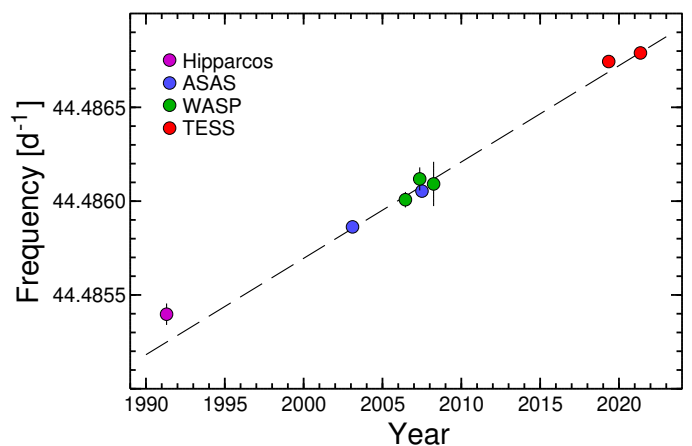
Fig. 2. Pulsation frequencies of the BLAP in HD 133729 system derived from the Hipparcos, ASAS, WASP, and TESS data. Dashed line corresponds to the derived constant rate of frequency change, d f_p / dt = (1.41 \pm 0.07) \times 10^{-7} \text{ d}^{-2} .
