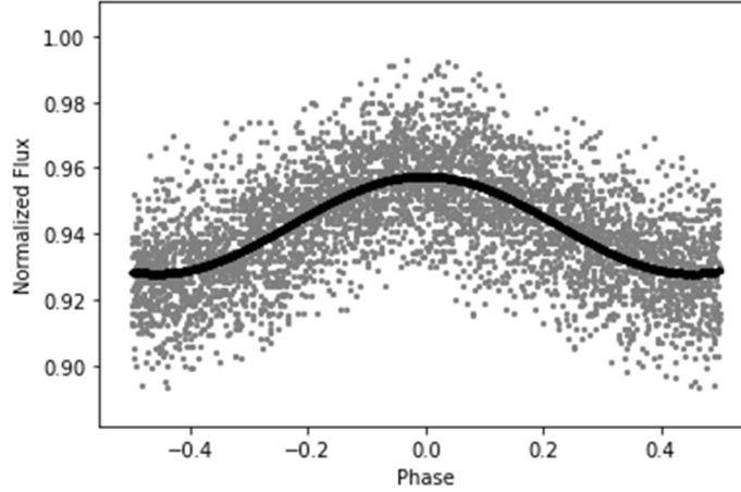
Figure 2. The phase-normalized flux curve for 2MASS 20250468+5026580.
