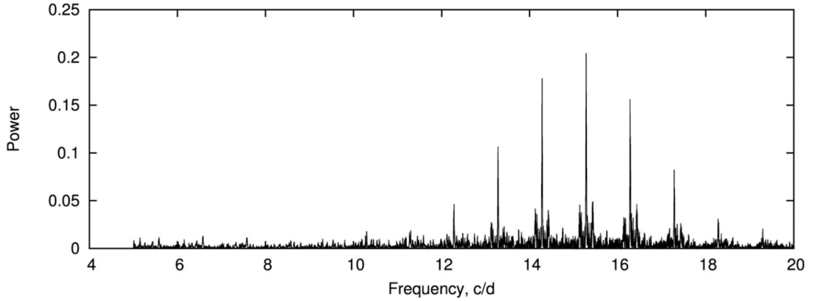
Figure 3. Periodogram of 2MASS 20250468+5026580 during the 2012-2013 observations.
