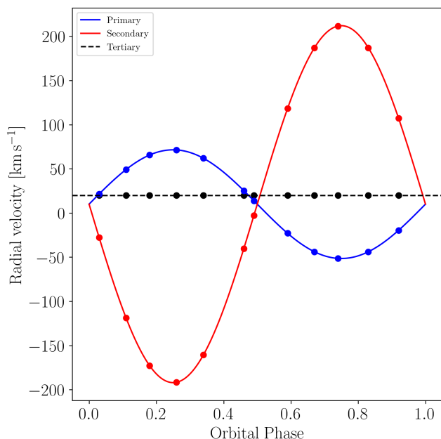
Fig. 3. Orbital solution for the primary (blue), secondary (red), and tertiary (black) components of U Gru obtained with the method of spectral disentangling. Note that the filled circles do not represent actual RV measurements. Instead, they indicate the distribution of the observed spectra over the orbital cycle of the inner binary system, while the orbital RV curve itself is computed from the best fit orbital elements.
