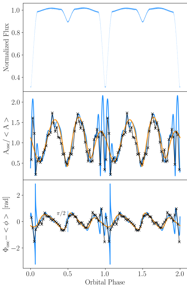
Fig. 10. (Top): Phase folded light curve of U Gru for sector 1. (Middle): Amplitude modulation of f_{14} = 33.046 \text{ d}^{-1} as reconstructed according to the fitting method developed by Jayaraman et al. (2022). The blue considers all 14 frequencies split from f_{14} and the orange lines consider those frequencies with f = f_{14} \pm N f_{\text{orb}} , where -3 \leq N \leq 3 . Tracked mode amplitudes from Section 4 shown as black x's. (Bottom): Same as the middle panel but for the phase modulation.
