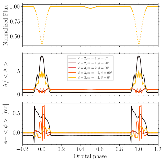
Fig. 8. (Top): Simulated light curves with different pulsation configurations (\ell, m, \beta) phase folded over the binary period. (Middle): Mode amplitude variations for different pulsation configurations as seen by an observer because of changing partial cancellation effects. (Bottom): Mode phase variations for different pulsation configurations as seen by an observer.
