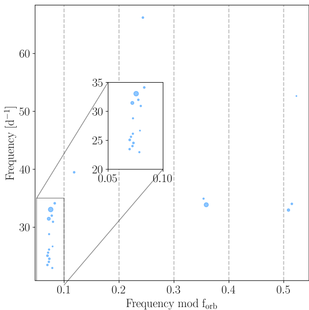
Fig. 6. Échelle diagram of the significant frequencies extracted from the residuals of sector 1 folded over the orbital period. The marker size scales with amplitude.
