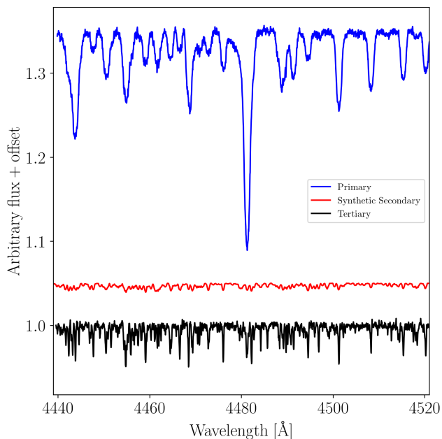
Fig. 2. Disentangled spectra of the primary (blue) and tertiary (black) components of the U Gru system. A representative synthetic spectrum corresponding to T_{\text{eff}} = 5500 K and \log g = 3.5 dex and diluted to the level of 2% (in continuum units) is shown for comparison to the secondary component (red). Note that a constant vertical shift have been applied to all the spectra for visibility purpose.
