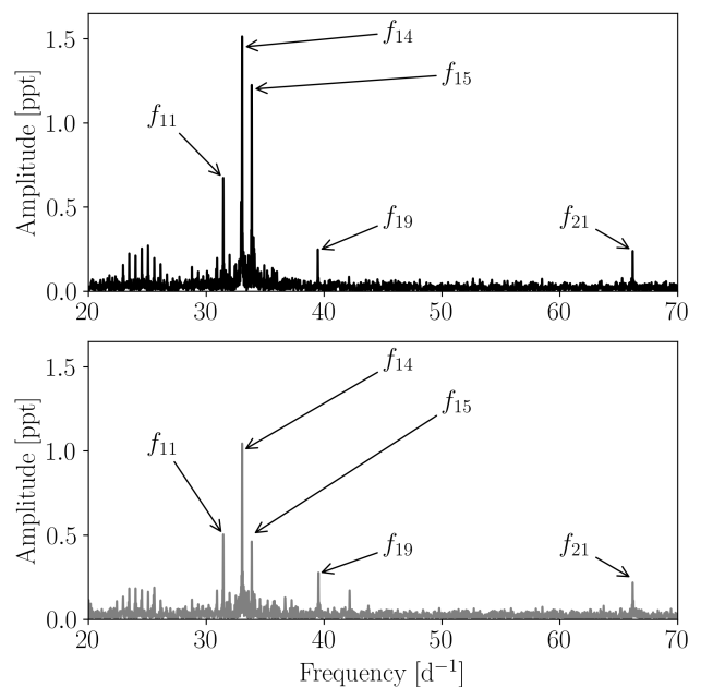
Fig. 5. (Top): Lomb-Scargle periodogram of binary subtracted residuals for sector 1. (Bottom): Lomb-Scargle periodogram of binary subtracted residuals for sector 28.
