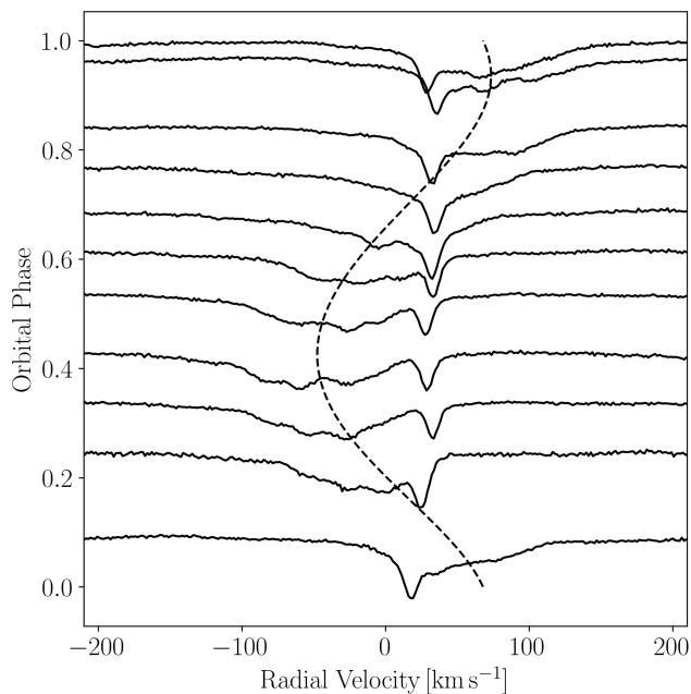
Fig. 1. The least-squares deconvolution profiles of U Gru computed from 11 blue arm UVES spectra. The orbital phase resolved spectral contribution of the broad-lined primary component is indicated with the dashed line.
