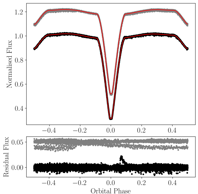
Fig. 4. (Top): Phase folded light curve of U Gru for sectors 1 (black) and 28 (grey) with the interpolated binary model in red. (Bottom): Residuals after subtraction of interpolation binary model for sectors 1 (black) and 28 (grey).
