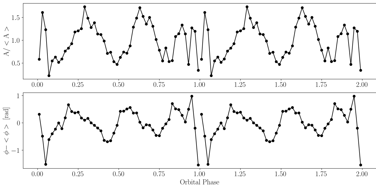
Fig. 7. (Top): Tracked mode amplitude for f_{14} = 33.046 \text{ d}^{-1} as a function of orbital phase. (Bottom): Tracked relative mode phase for f_{14} = 33.046 \text{ d}^{-1} as a function of orbital phase. Phase values of 0, 1 and 2 correspond to primary eclipse, and phase values of 0.5 and 1.5 correspond to secondary eclipse.
