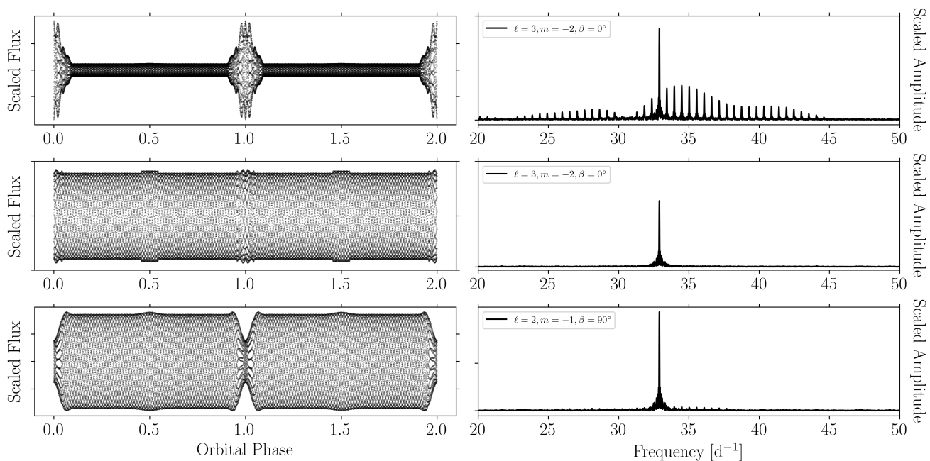
Fig. 9. Left column display simulated light curves of the pulsation mode only. Right column displays periodogram of the accompanying light curve. These light curves do not consider the light variations caused by the binary itself.
