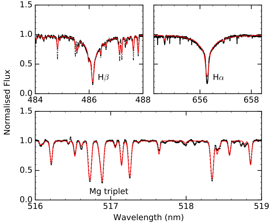
Figure 6. The H\beta (top left), Mg_1 triplet (bottom), and H\alpha (top right) line regions for the target star. The observed (black) and synthetic spectra (red) are shown. The synthetic spectrum was obtained with LTE consideration. The majority of the narrow features in the observed spectrum that the models do not fit are telluric lines.
