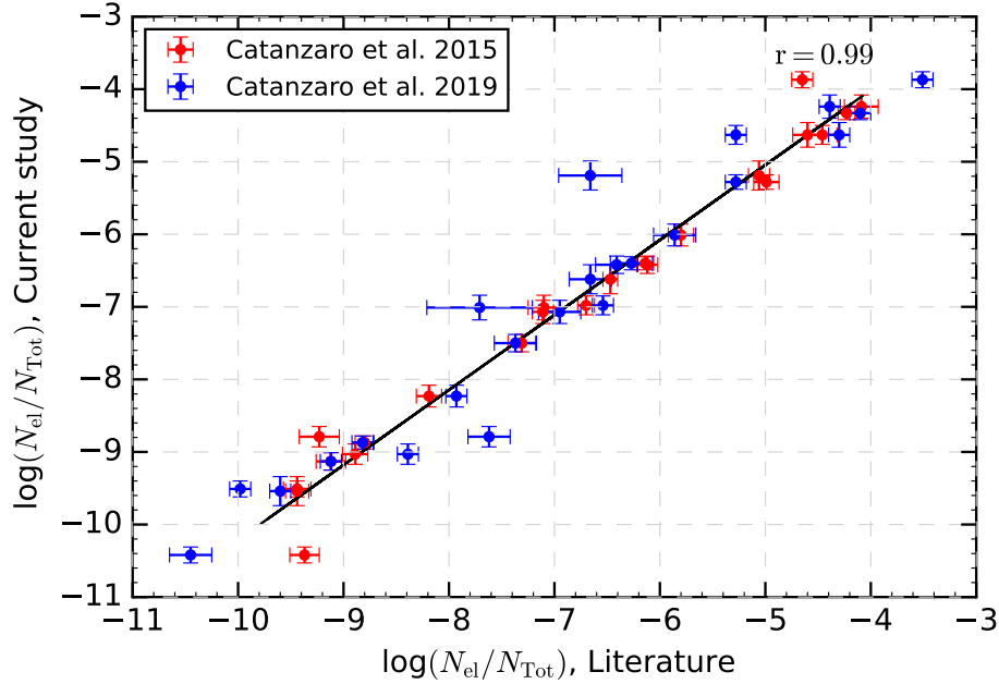
Figure 9. A comparison of our individual chemical abundances with those determined by Catanzaro et al. (2015) and Catanzaro et al. (2019) . The corresponding correlation coefficient ( r ) is given in the top-right corner.
