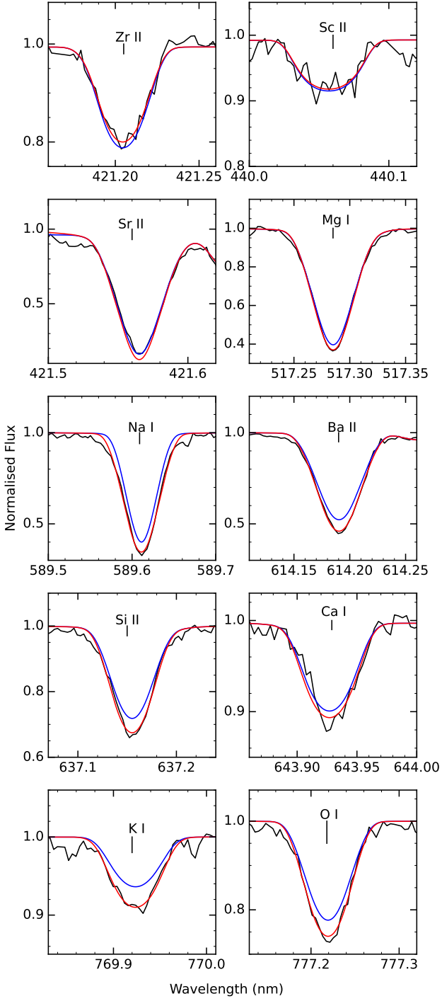
Figure 10. NLTE (red) fits of Zr II 421.188 nm, Sc II 440.039 nm, Sr II 421.552 nm, Mg I 517.285 nm, Na I 589.592 nm, Ba II 614.171 nm, Si II 637.137 nm, Ca I 643.929 nm, K I 769.897 nm, and O I 777.194 nm. For each line, the LTE (blue) profile was computed with the respective abundance obtained from NLTE analysis. In each panel, the black line represents the observed spectrum.
