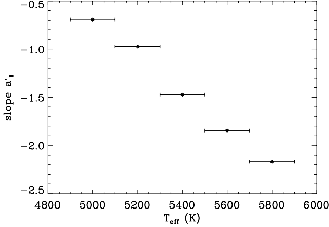
Figure 6. Slope a'_1 for Eq. 3 as a function of effective temperature bins.
