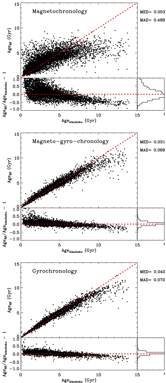
Figure 10. Comparison of ages predicted from the Random Forest with the model ages for late F, G, and K dwarfs. Top panel: magnetochronology. Middle panel: magneto-gyro-chronology. Bottom panel: gyrochronology. Same legend as in Figure 9.
