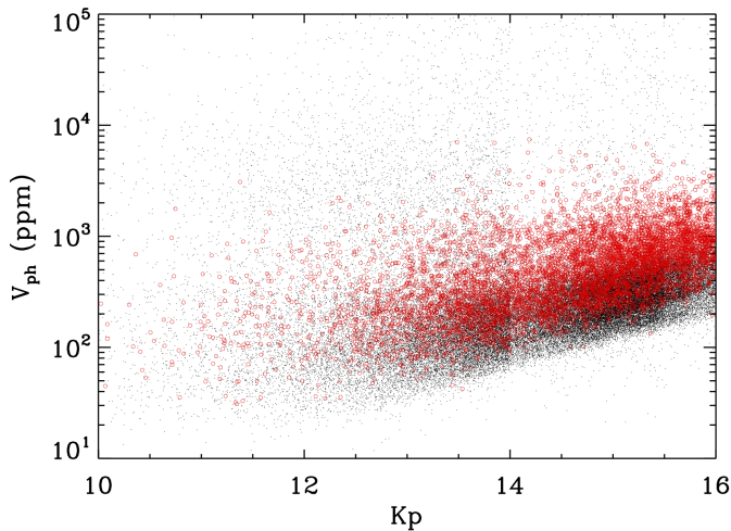
Figure 12. Variability index V_{\text{ph}} as a function of the Kp magnitude for stars without rotation periods (black dots) and stars with rotation periods and ages derived in this work above 5 Gyr (red circles).
