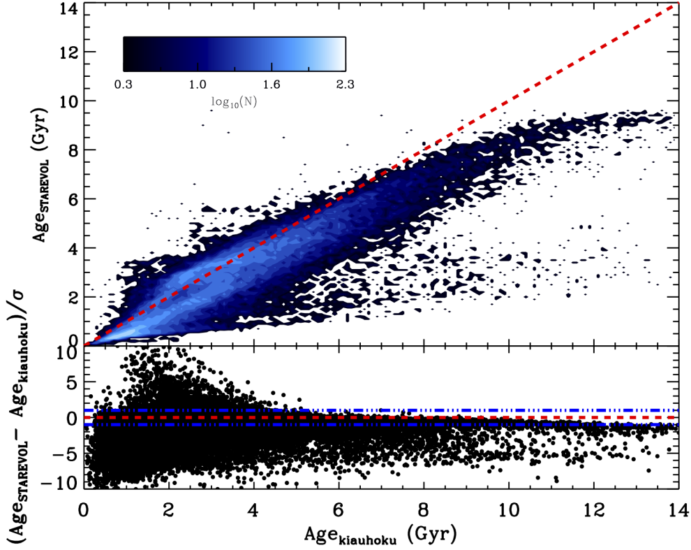
Figure 2. Top: Comparison of ages computed by kiauhoku and STAREVOL color-coded by density number of stars. The dashed line corresponds to the 1:1 relation. Bottom: Ratio of age differences over \sigma , the square root of the sum of the quadratic uncertainties from each method. The dotted-dashed lines represent \pm 1\sigma .
