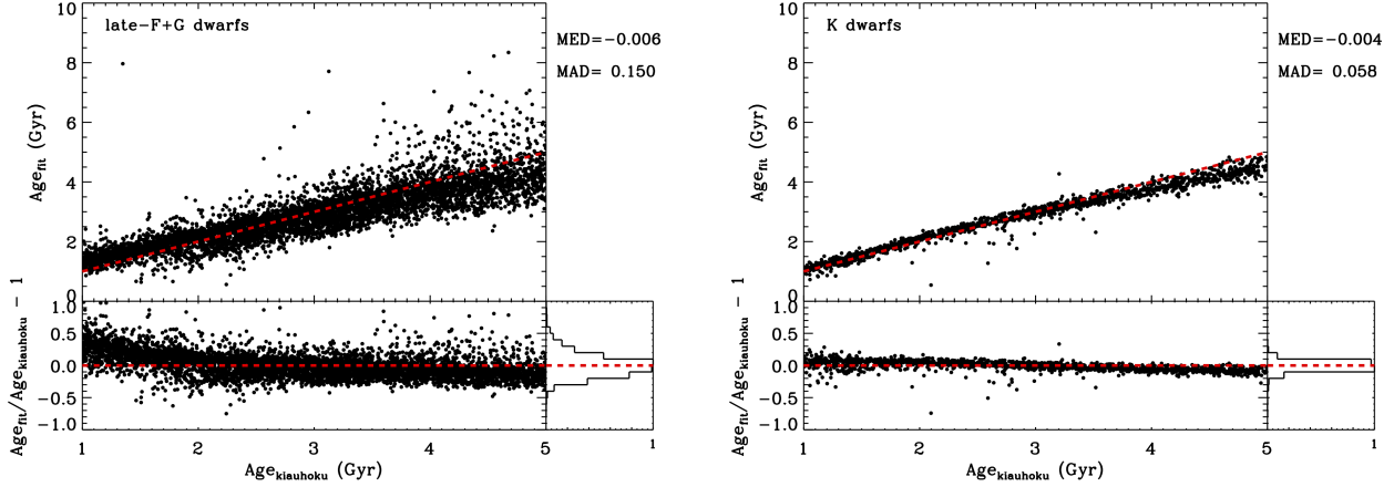
Figure 18. Age comparison for the predicted ages from Equation (5) without the S_{ph} term with the kiuhoku ones for the late-F and G dwarfs (left panel) and the K dwarfs (right panel). Same legend as in Figure 9.
