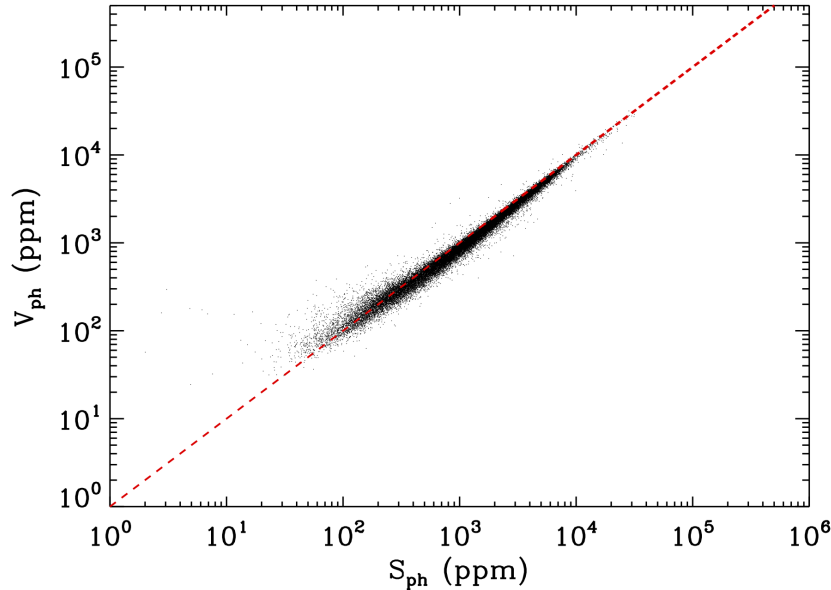
Figure 19. Comparison between the photometric magnetic activity index, S_{ph} computed on subseries of length 5 \times P_{rot} and a newly defined variability index, V_{ph} , computed on subseries of length 30 days. Both indexes were computed with the 55-d filtered data.
