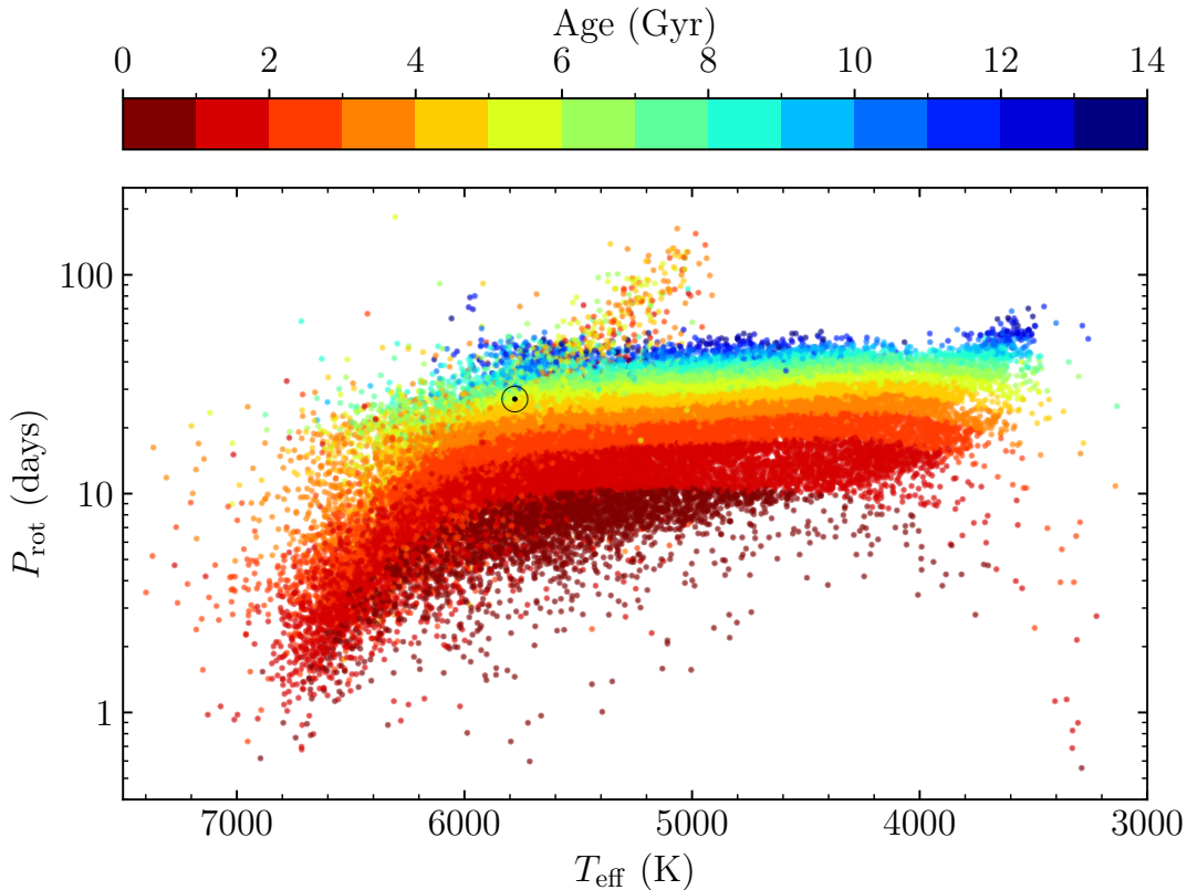
Figure 1. P_{\text{rot}} vs. T_{\text{eff}} color-coded by ages computed with kiauhoku for 41,440 stars. The Sun is represented with its usual symbol in black with a rotation period of 26.43 d (Santos et al. 2023).
