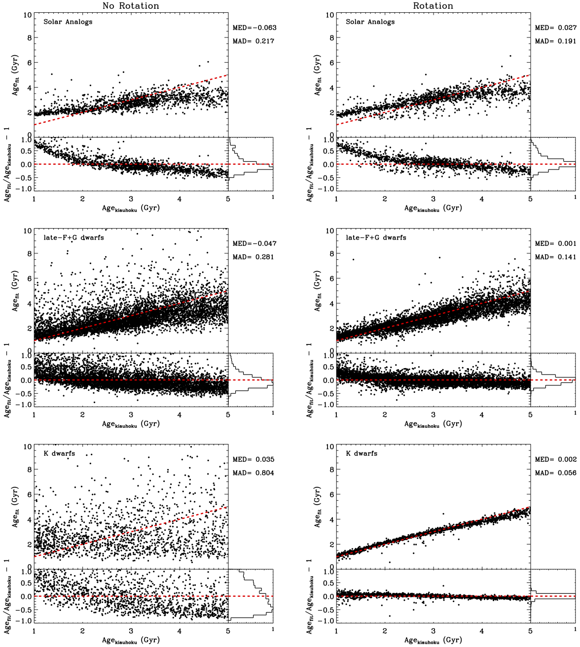
Figure 9. Magneto-chronology (without rotation, left column) and magneto-gyro-chronology (with rotation, right column) results from the Bayesian fits. Top row: linear fit for solar analogs. Middle row: multivariate fit for late F and G dwarfs. Bottom row: multivariate fit for K dwarfs. In each figure, the top panel shows the ages computed from the multivariate fit compared to the model ages and the dash red line corresponds to the 1:1 line. The bottom panels of each figure represent the ratio of the ages centered on 0 and the corresponding histogram (as a fraction). The median (MED) and Median Absolute Deviation (MAD) are given for each fit in the top right of each figure.
