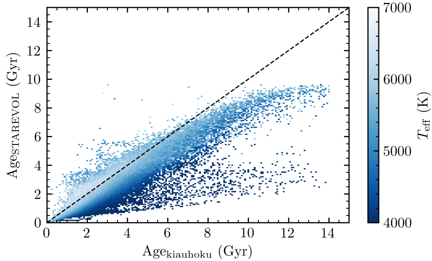
Figure 13. Ages from kiauhoku compared to STAREVOL as computed in Section 4.2 color-coded with T_{\text{eff}} .
