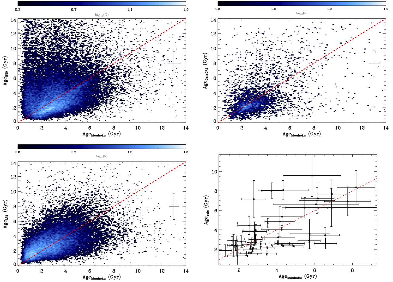
Figure 3. Literature ages as a function of the ages obtained in this work ( Age_{kiauhoku} ). Top left panel: Gaia-Kepler catalog (B20). Top right panel: Gaia DR3 FLAME ages (C22). Bottom left panel: gyro-kinematic ages (L21). Bottom right panel: seismic ages (SA17). The red dashed line corresponds to the 1:1 line. In the cases of the B20, Gaia DR3, and L21, only the average uncertainties are represented for clarity purposes.
