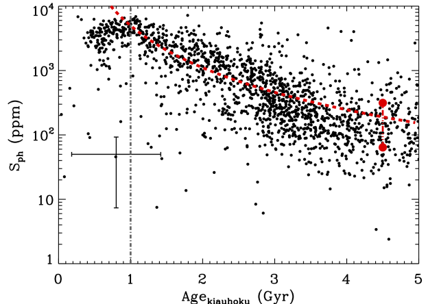
Figure 5. S_{\text{ph}} as a function of age for solar analogs where the red dashed line represents the results of the linear fit (Equation (3)) done in the log-log space. The fits were performed between 1 and 5 Gyr and the grey dotted-dashed line shows that lower limit in age. The red large circles represent the S_{\text{ph}} values of the Sun between minimum and maximum activity.
