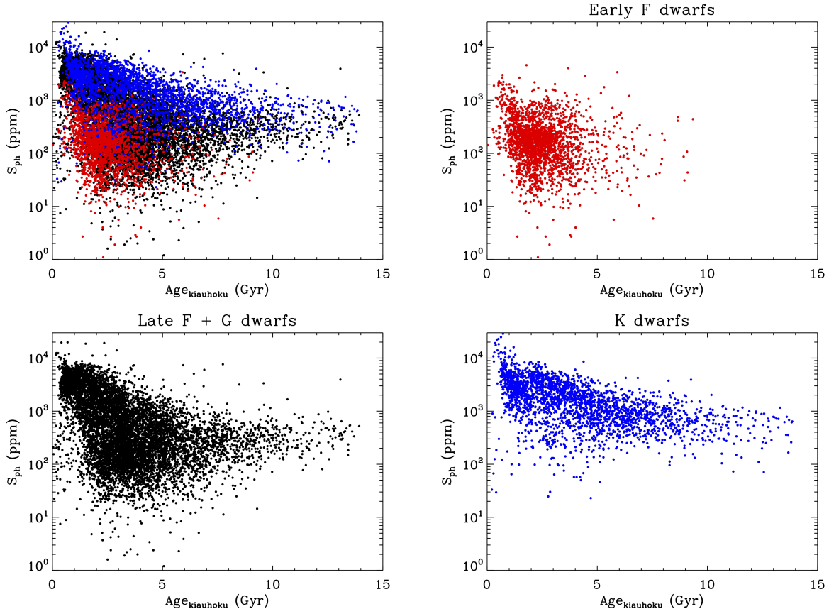
Figure 4. S_{\text{ph}} -age relation for early F (red symbols), late F and G (black symbols), and K (blue symbols) dwarfs all together with spectroscopic data and separated by spectral type.
