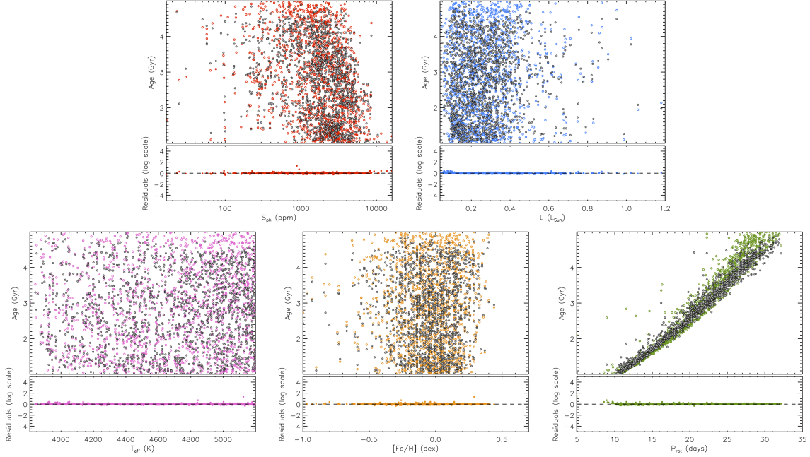
Figure 17. Residuals for K dwarfs for the multivariate regression of Section 5 with P_{\text{rot}} . Same legend as in Figure 14 but with also the residuals regarding P_{\text{rot}} (bottom right panel).
