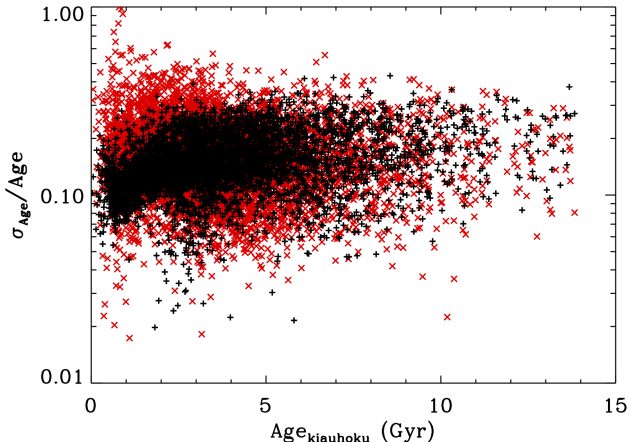
Figure 8. Relative errors from kiauuhoku (black crosses) and from the magnetochronology RF algorithm (red crosses) as a function of age.
