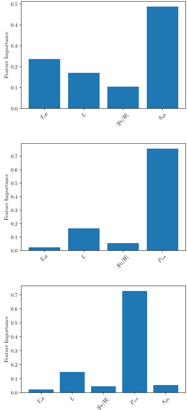
Figure 7. Random Forest Features importance for magnetochronology (top panel), gyrochronology (middle panel), and magneto-gyro-chronology (bottom panel).
