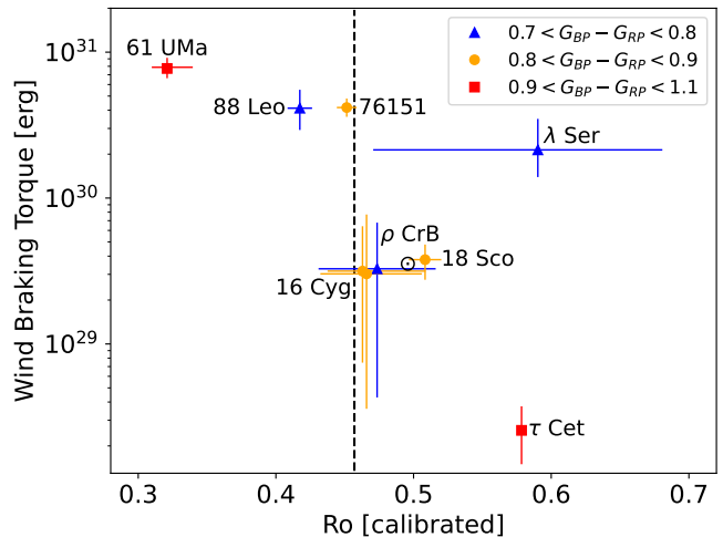
Figure 8. Evolution of the wind braking torque with \text{Ro} from the calibration of Corsaro et al. (2021). Points are grouped by Gaia color, corresponding to solar analogs (yellow circles), and hotter (blue triangles) or cooler stars (red squares). The empirical constraint for \text{Ro}_{\text{crit}} on this scale is shown with a vertical dashed line.
