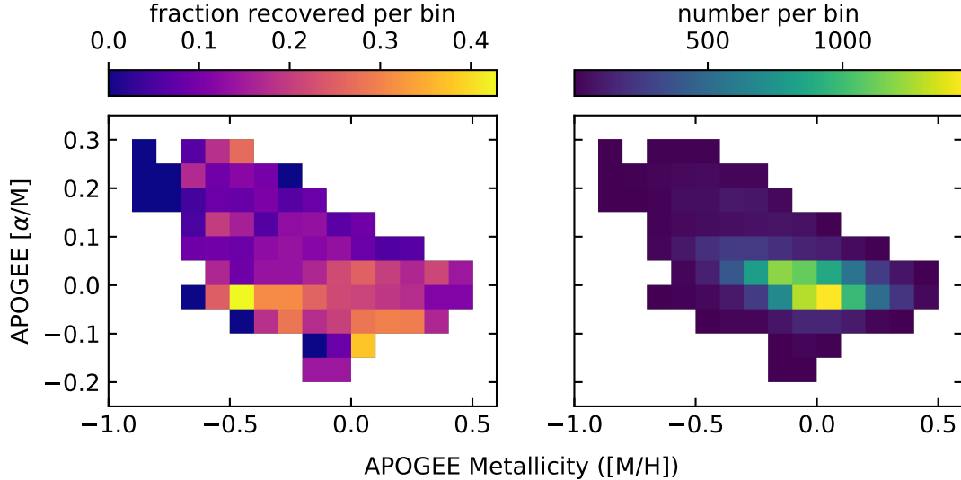
Figure 14. The detectability of rotation across APOGEE metallicity and \alpha -element abundance. We detect fewer stars in rotation at high [\alpha/M] because these stars tend to be old, slowly rotating, and less active. At fixed [\alpha/M] , there is scatter in the trend of detectability with metallicity from bin to bin.
