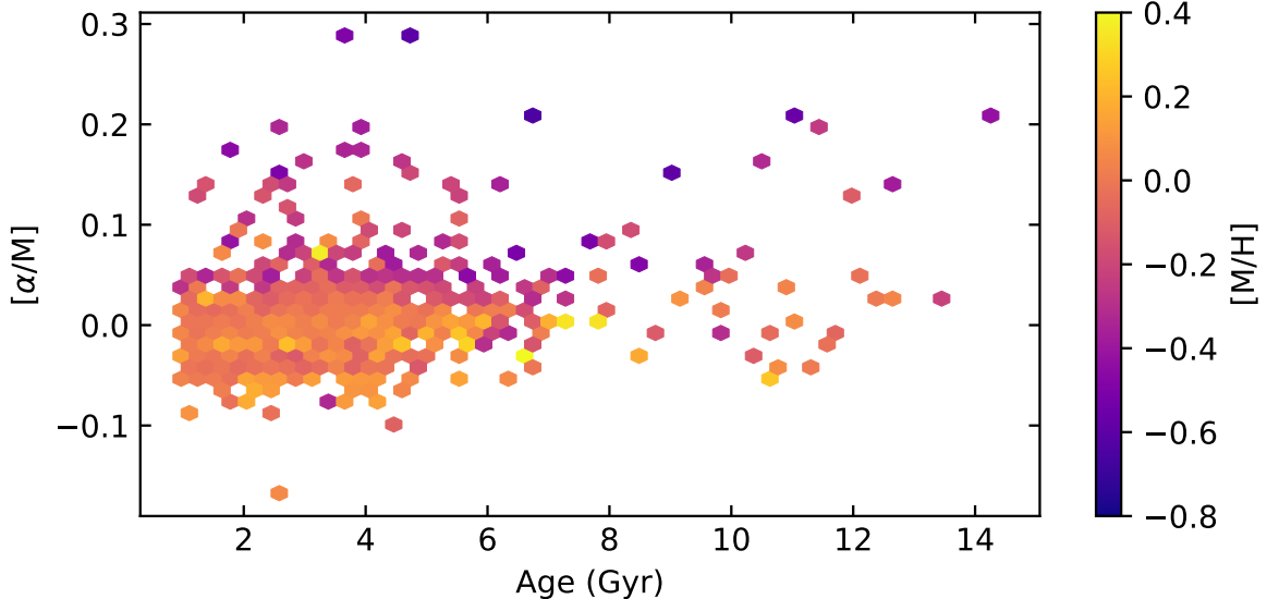
Figure 10. Stellar \alpha -element abundances vs. age in the TESS SCVZ (the Gold sample in Table 1), tracing Galactic chemical evolution of \alpha -enhancement from supernovae. Consistent with trends seen in the Kepler field (e.g., Silva Aguirre et al. 2018; Claytor et al. 2020a), there is a weak trend of increasing \alpha abundance with age below 8 Gyr associated with the classical “thin” Galactic disk. We expect but do not see a strong trend of increasing \alpha abundance with age above 8 Gyr (the classical “thick” disk), but this because we detect very few older stars due to (1) our 27-day detection edge, and (2) slow rotation and weak activity making stars more difficult to detect.
