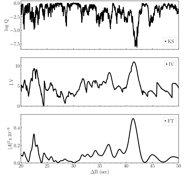
Figure 8. K-S (upper panel), I-V (middle panel), and F-T (bottom panel) significance tests to search for a constant period spacing in the case of G 29–38. The tests are applied to the pulsation periods in Table 3. A period spacing of \sim 41 s is evident.
