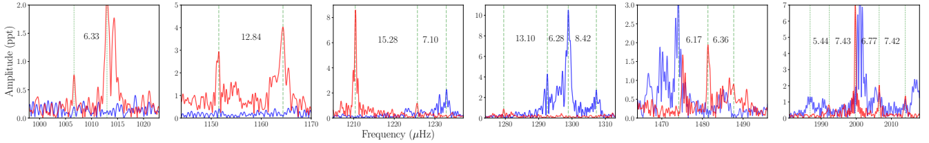
Figure 6. Same as in Fig. 5 to display rotational quintuplets. The sub-plots present rotational splittings in three different regions in the amplitude spectrum, with an average splitting of \delta\nu = 6.66 \mu\text{Hz} for \ell = 2 modes. See text for more details.
