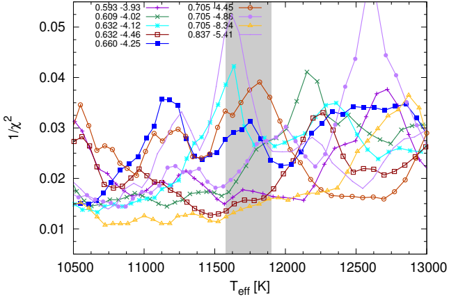
Figure 12. Inverse of the squared quality function \chi in terms of the effective temperature for the best-fit models that agrees with Gaia distance within 10% (labeled here according to their respective M_{\star} , \log(M_{\text{H}}/M_{\star}) values). The grey region represents the averaged T_{\text{eff}} and its error from MWDD. For comparison, we also include the model that best matches the pulsation periods of G 29–38.
