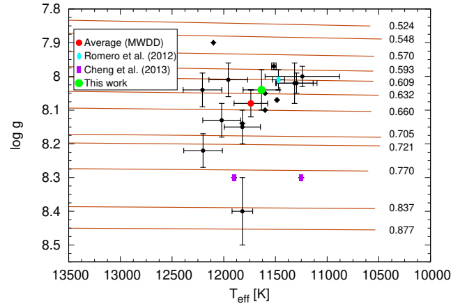
Figure 10. Determinations of \log g and T_{\text{eff}} (black dots) for G 29–38 from the Montreal White Dwarf Database (see the compilation in Table 1) together with their average (red circle), our asteroseismic solution (green circle), and asteroseismic solutions from previous works (cyan ellipse and magenta rectangles). Superimposed on these, we plot each of our canonical evolutionary sequences and their corresponding value of stellar mass in solar units (red lines)
