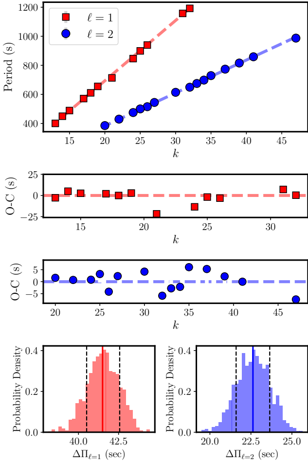
Figure 9. Linear least-squares fit the periods of G 29–38 marked with filled red squares ( \ell = 1 ) and blue dots ( \ell = 2 ). The derived period spacing from this fit is \Delta\Pi_{\ell=1} = 41.20 s and \Delta\Pi_{\ell=2} = 22.58 s. The residuals for \ell = 1 modes (second panel) and \ell = 2 modes (third panel) of the period distribution relative to the mean period spacing. The fourth panel shows the distribution of the resulting fits for \ell = 1 modes (left panel) and \ell = 2 modes (right panel). The lower and upper bounds, which are shown with vertical dashed black lines are calculated by determining the 16th and 84th percentiles of each distribution. The derived mean period spacing corresponds to the 50th percentiles, which are shown with a vertical red line for \ell = 1 modes and a vertical blue line for \ell = 2 modes.
