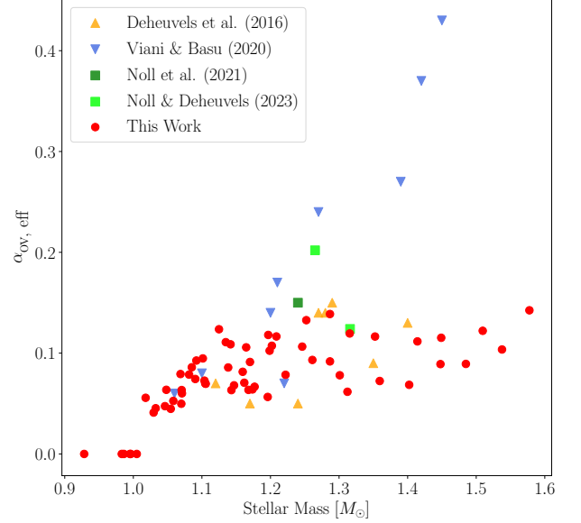
Figure 7. \alpha_{\text{ov, eff}} versus stellar mass results (red points) in comparison with other asteroseismic studies of convective core overshoot.
