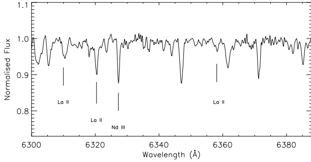
Figure B5. Segment of the LAMOST medium resolution spectrum of TIC 26833276.
