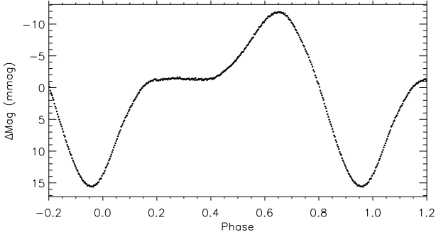
Figure 8. Phase folded SAP light curve of TIC 335457083, phased on a period of 2.9139 \pm 0.0001 d. Binned 50:1.
