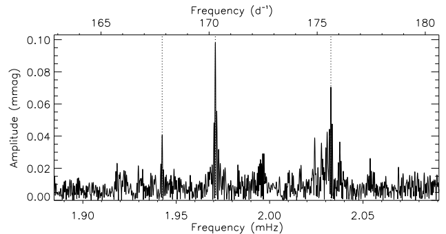
Figure 19. Amplitude spectrum of TIC 118247716, with three modes clearly identifiable. Further modes may be present close to the noise level.
