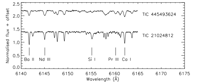
Figure B2. HERMES spectra of TIC 445493624 and TIC 21024812 in the red region.
