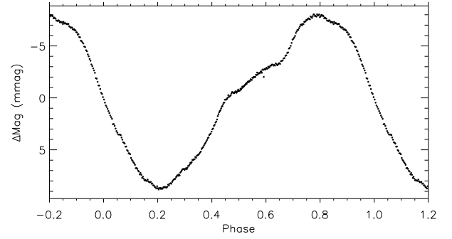
Figure 31. Phase folded SAP light curve of TIC 298052991, phased on a period of 10.5852 \pm 0.0001 d. Binned 200:1
