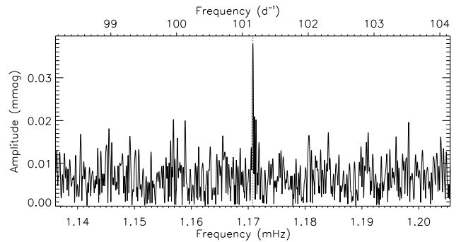
Figure 33. Amplitude spectrum of TIC 405892692 showing the detection of a pulsation mode (marked by the vertical dotted line).
