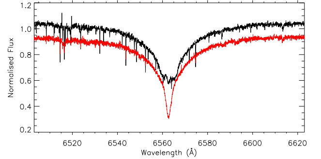
Figure B8. HERMES spectra of TIC 435263600 showing the binary nature of the system. The two epochs are plotted in black and red, offset in intensity for clarity. The top panel shows the region classically used for spectral classification (note the significant change in the Ca II K line profile), while the bottom panel shows the region around H_{\alpha} . It is easy to see how multiple different classifications can arise from observing the star at different epochs.
