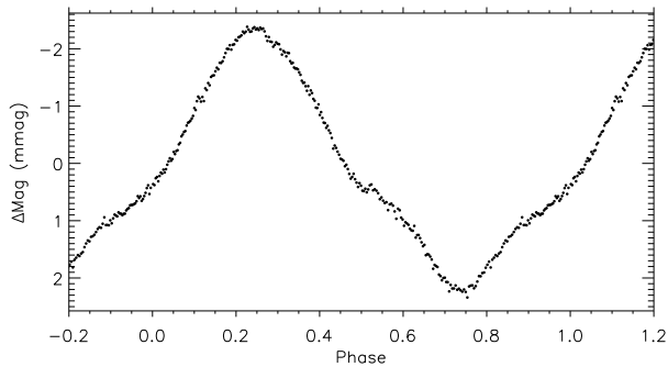
Figure 6. Phase folded light curve of TIC 259017938, phased on a period of 5.0226 \pm 0.0005 d. Binned 100:1.
