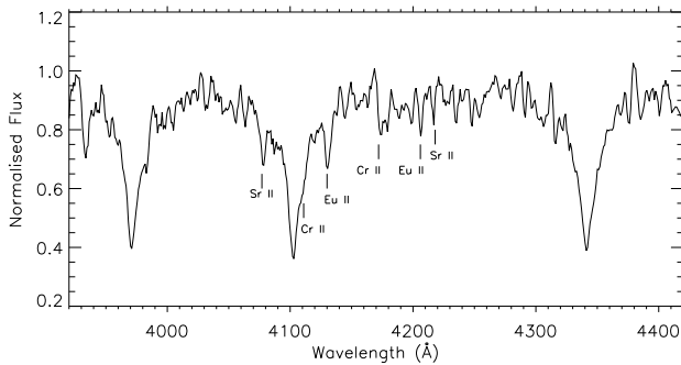
Figure B7. LAMOST low resolution spectrum of TIC 118247716 showing the clear presence of Sr II, Eu II and Cr II.
