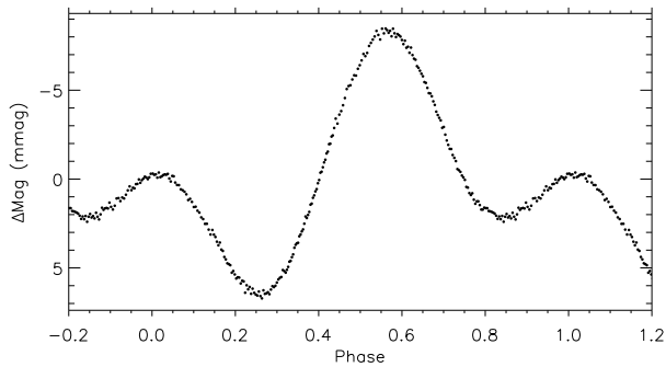
Figure 17. Phase folded light curve of TIC 72392575, phased on a period of 3.9016 \pm 0.0008 d. Binned 50:1.
