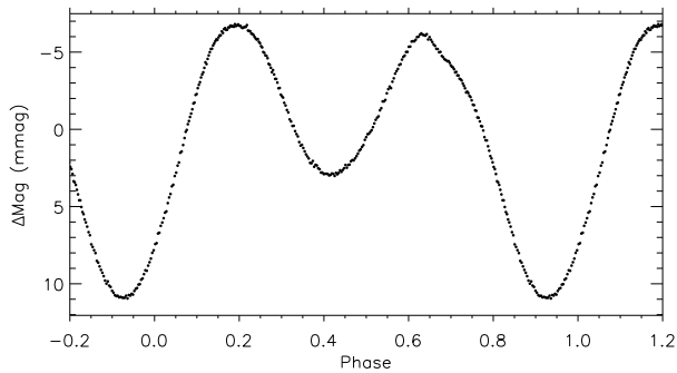
Figure 12. Phase folded light curve of TIC 467074220, phased on a period of 5.4195 \pm 0.0004 d. Binned 50:1.
