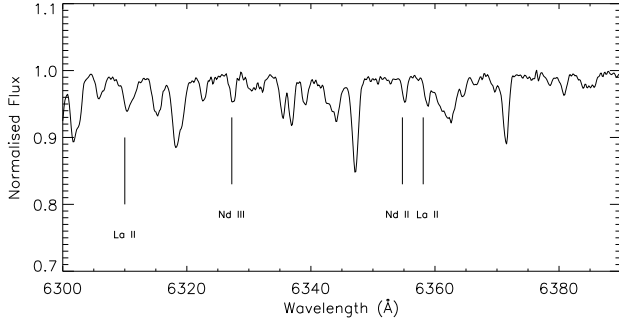
Figure B4. Segment of the LAMOST medium resolution spectrum of TIC 259017938.
