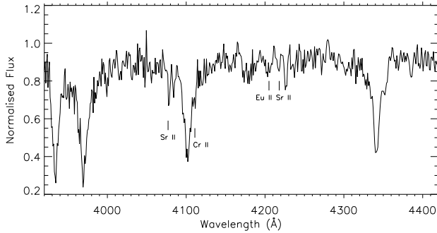
Figure B6. LAMOST low resolution spectrum of TIC 101624823 showing the clear presence of Cr II, with indications of Sr II and Eu II indicated.
