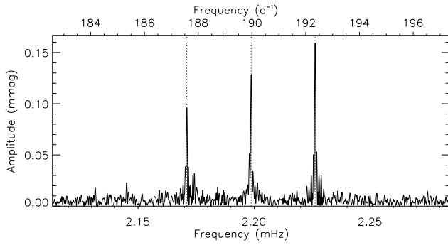
Figure 20. Amplitude spectrum of TIC 120532285
