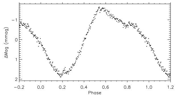
Figure 1. Phase folded light curve of TIC 101624823, phased on a period of 4.050 \pm 0.001 d. Binned 50:1.
