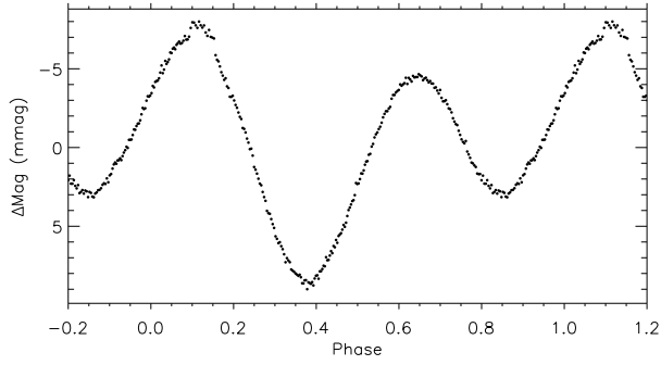
Figure 29. Phase folded light curve of TIC 275642037, phased on a period of 2.8745 \pm 0.0003 d. Binned 50:1
