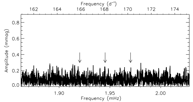
Figure C6. Amplitude spectrum for TIC 158216369. The arrows identify the locations of the pulsation modes listed in the literature. Their amplitudes are below the noise level in the TESS data.
