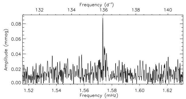
Figure 18. Amplitude spectrum of TIC 72392575, showing the pulsation mode. At slightly higher frequency there is a power excess which might be a rotational sidelobe.
