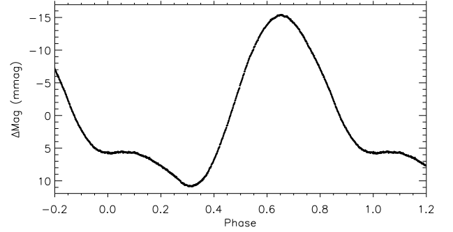
Figure 4. Phase folded light curve of TIC 233200244, phased on a period of 7.25002 \pm 0.00006 d. Binned 200:1.
