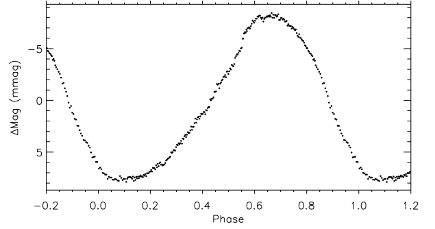
Figure 10. Phase folded SAP light curve of TIC 445493624, phased on a period of 7.288 \pm 0.002 d. Binned 50:1.
