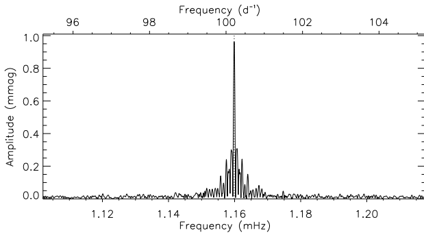
Figure 37. Amplitude spectrum of TIC 91224991
