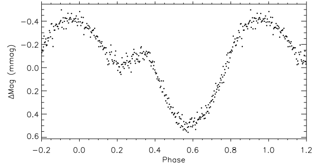
Figure 35. Phase folded light curve of TIC 445796153, phased on a period of 5.5721 \pm 0.0004 d. Binned 100:1
