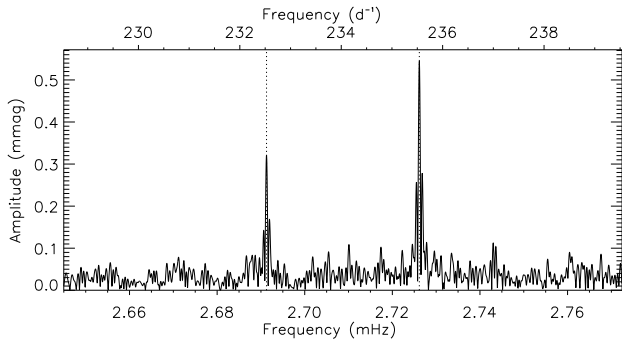
Figure C13. Amplitude spectrum for TIC 286992225. The vertical dotted lines identify the pulsation modes detected in the TESS data; the lowest frequency mode is a new detection.
