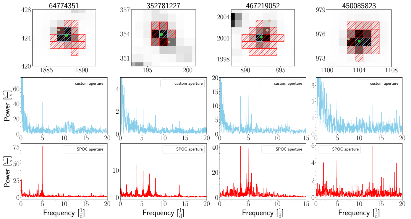
Figure 5. A plot of the TESS target pixel files of 4 of the 7 stars discussed in Appendix 1. These stars were the ones for which custom light curves were made. The top panel shows the target pixel files, with the star of interest shown in green (and indicated in the title) and the potentially contaminating stars shown in tan. The middle panel shows the light curve created using a custom aperture (shown in blue in the top panel); the bottom panel shows the light curve generated via the SPOC pipeline. Note that the y-axis scales differ between the middle and bottom panels as a result of the fact that the custom aperture imperfectly captures the flux from the star of interest. This, however, provides the advantage of allowing us to highlight the peak locations.
