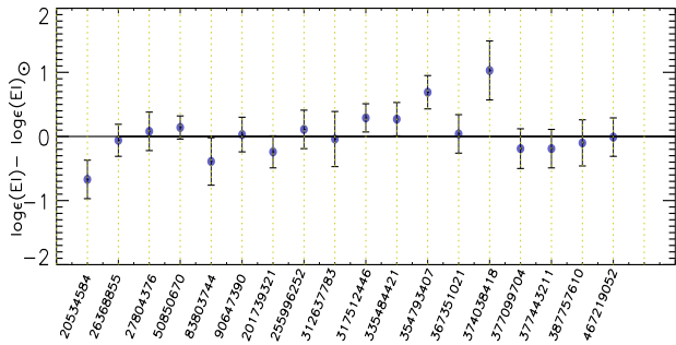
Figure 4. The differences between the obtained and solar (?) Fe abundances for each star. The x-axis represents the TIC numbers.
