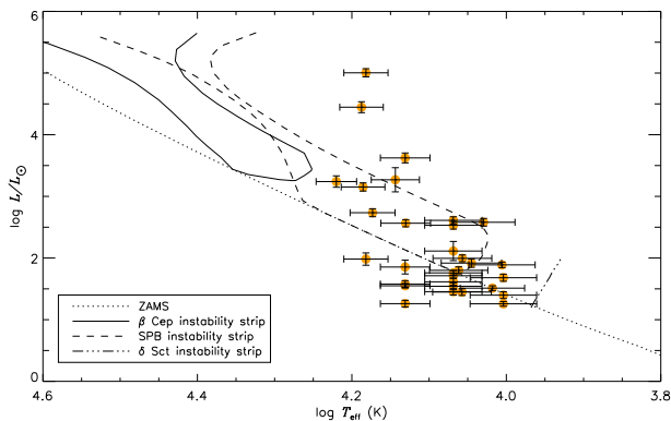
Figure 1. The initial positions of the selected candidates in the H-R diagram as derived by Balona & Ozuyar (2020). The theoretical instability strips of the \beta Cephei and SPB stars were taken from ?. The domain of the \delta Scuti stars was taken from Murphy et al. (2019).
