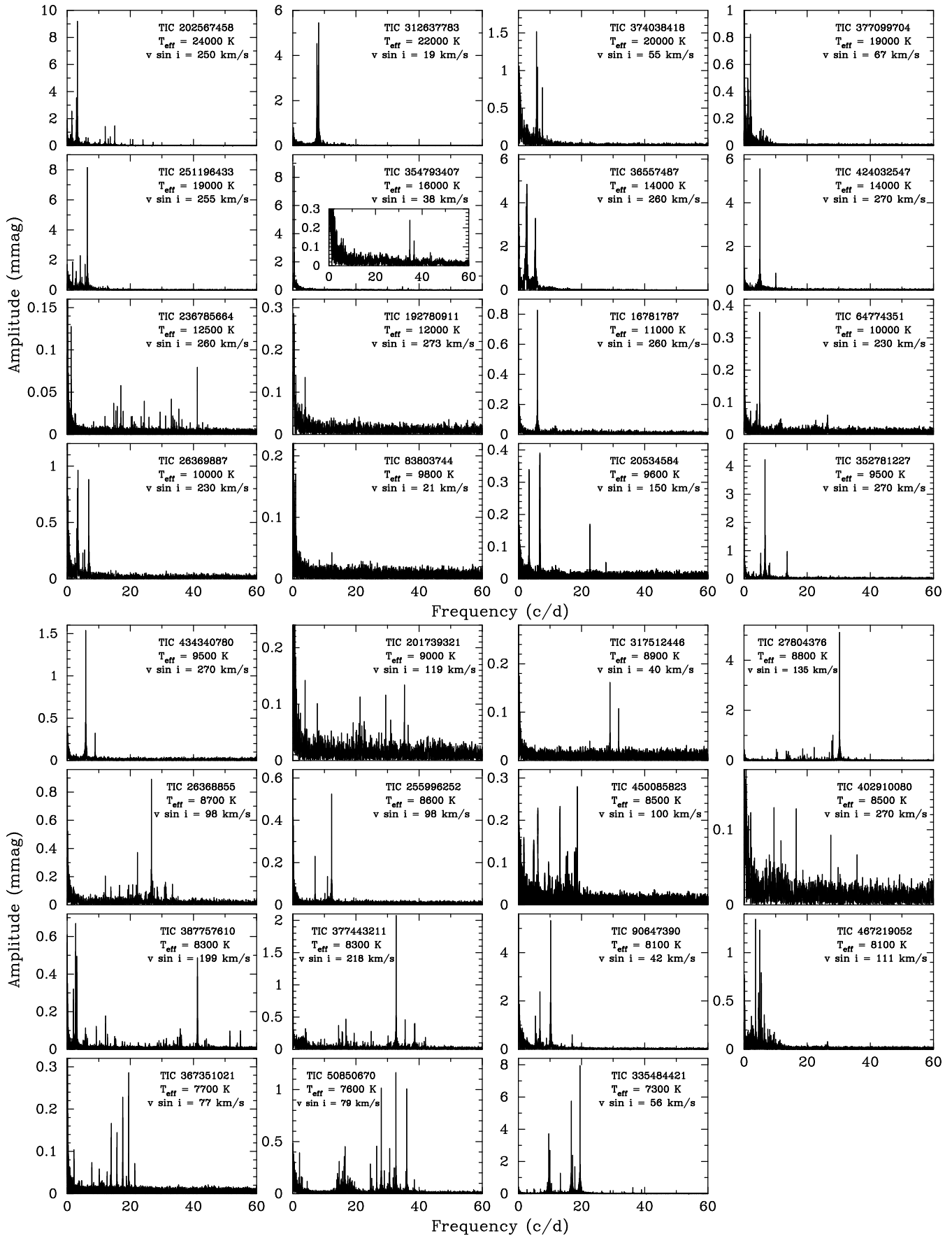
Figure A1. Amplitude spectra of the targets in order from the hottest star to the coldest star.
