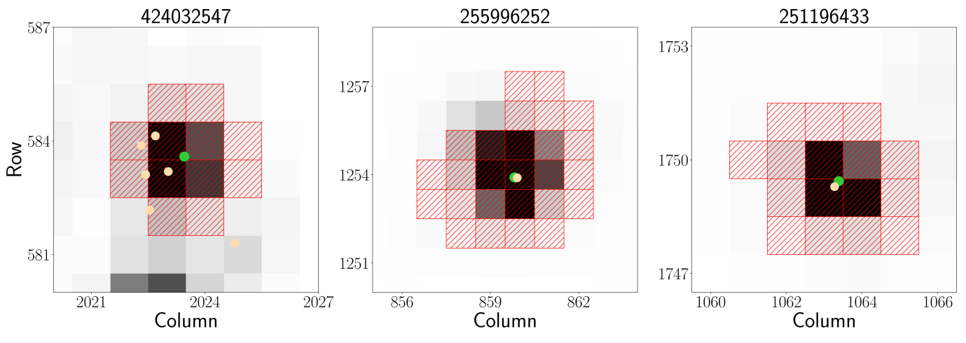
Figure 6. Each panel contains the target pixel file for a star that is so heavily contaminated that we are unable to determine where the true source of the frequency peaks in the periodogram lies. As in Figure 5, the green points represent the source of interest, while the tan points represent potentially contaminating stars.
