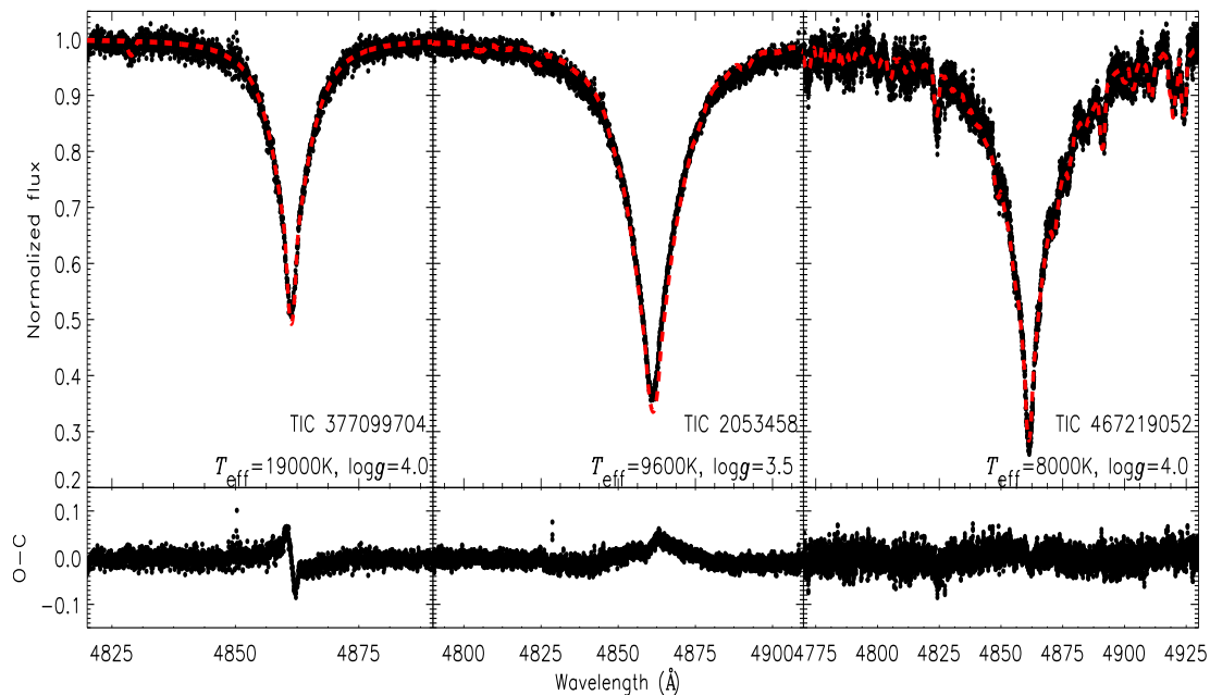
Figure 2. Upper panels: Theoretical spectral fits (red dashed lines) to the observed spectra of target stars. Lower panel: Residuals.
