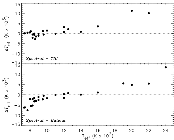
Figure 8. Comparison of the T_{\text{eff}} of the TIC (Stassun et al., 2019) (upper panel) and Balona & Ozuyar (2020) (lower panel) with the spectral T_{\text{eff}} determined in this study. The x-axis shows the spectral T_{\text{eff}} values while the y-axis illustrates the T_{\text{eff}} differences between the spectral and TIC (upper panel) and Balona & Ozuyar (2020) (lower panel).
