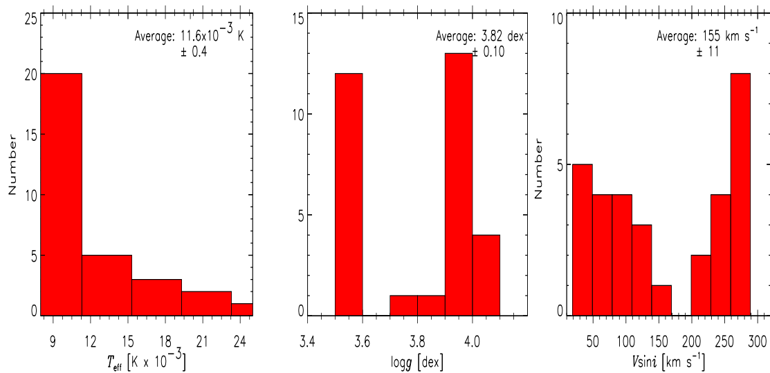
Figure 3. Distributions of the T_{\text{eff}} , \log g and v \sin i parameters.
