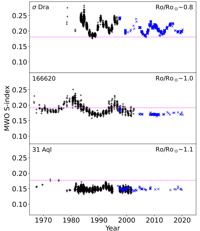
Figure 6. Evolution of stellar activity cycles through the critical activity level that corresponds to Ro_{\text{crit}} (magenta dashed lines). Mount Wilson data are shown with black plus symbols, while Keck data are shown with blue crosses (Baum et al. 2022). Close to the onset of WMB, the critical activity level is near cycle minimum as in \sigma Dra (top). As the mean activity level decreases with age, the cycle can develop intermittency as in HD 166620 (middle). Continued evolution pushes the mean activity level permanently below the critical value, and cycles disappear entirely as in 31 Aql (bottom).
