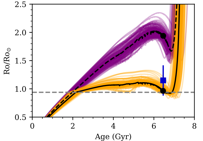
Figure 5. Evolution of the Rossby number for \beta Hgi in the YREC model grid, with samples drawn from the posterior of the standard spin-down model (purple curves) and from the WMB model (orange curves). The value of \text{Ro}_{\text{crit}} is shown as a gray dashed line, while the best-fit value of the Rossby number is shown as a circle for both braking law prescriptions. The actual position of \beta Hgi (assuming the convective turnover time of the best fit model but the measured period and age) is shown as a blue square with an error bar.
