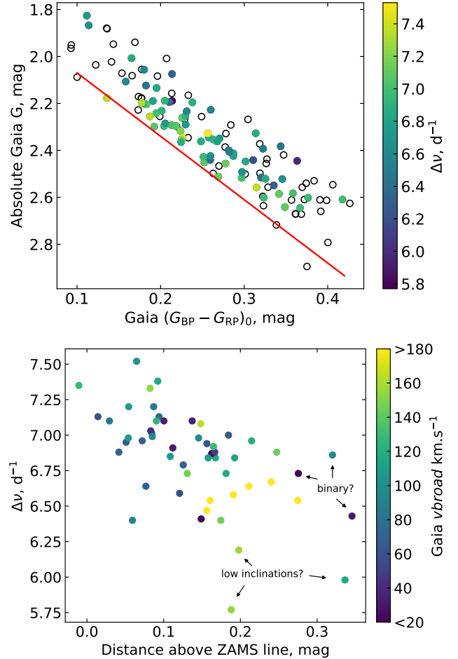
Figure 12. Top: The colour–magnitude diagram for the ZAMS group of stars in Cep–Her, colour-coded by measured \Delta\nu . Open black symbols show stars for which no \Delta\nu could be measured, 40% of which are rapid rotators. The red line is the ZAMS line introduced in Sec. 2.6. Bottom: the subset of stars for which \Delta\nu was measurable and Gaia v_{\text{broad}} was available, showing \Delta\nu as a function of the height above the ZAMS line. Stars farther from the ZAMS line should have a lower density, either due to rapid rotation or due to evolutionary effects such as pre-MS status. Stars indicated with arrows are discussed in the text.
