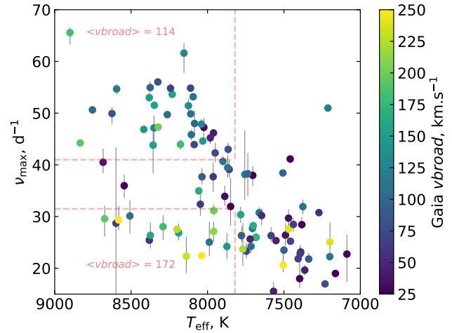
Figure 8. The \nu_{\max} and T_{\text{eff}} values for Cep–Her stars in the ZAMS group, colour-coded by their Gaia \text{vbroad} values. Dashed lines separate stars that are unambiguously on the bottom ridge from those on the upper ridge, and the mean \text{vbroad} within each division is shown.
