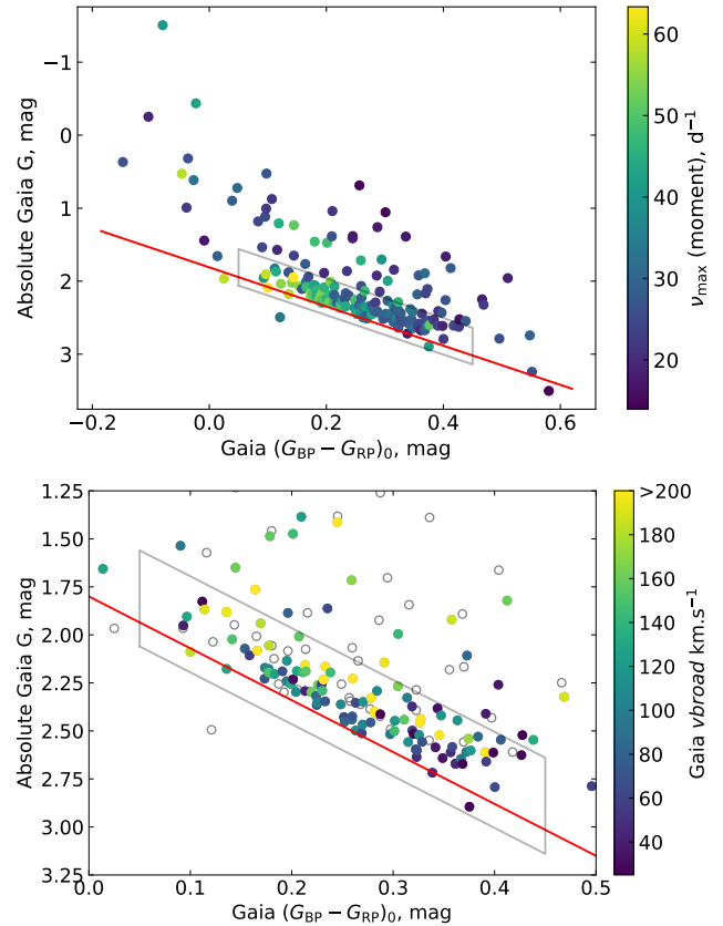
Figure 4. Top: colour–magnitude diagram of the \delta Sct stars in the Cep–Her association, with plot symbols colour-coded by \nu_{\max} , as measured by the moment (amplitude) method. The location of the ZAMS is estimated with the red line. The grey box encloses the ‘ZAMS group’ of coeval stars, which is described in the text and used for detailed analysis. Bottom: Zoom-in on the ZAMS group, showing the range of rotation velocities of the stars. Open grey symbols show stars without Gaia v broad data.
