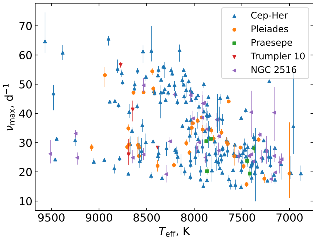
Figure 7. The distributions of \nu_{\max} and T_{\text{eff}} for the handful of clusters described in Sec. 3.3. Symbols denote the mean of the aggregate methods for measuring \nu_{\max} , while vertical bars span the range of \nu_{\max} from those methods for each star. Of interest is the emerging structure of two ridges that merge around 8000 K.
