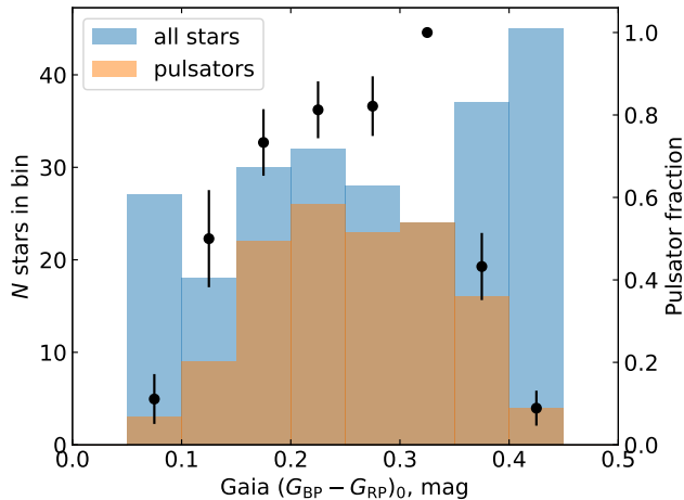
Figure 9. Histograms of the total number of stars and the number of those that are pulsating (left y-axis), as a function of colour. The right y-axis shows the ratio of those quantities as the pulsator fraction, with uncertainties calculated via Eq. 6.
