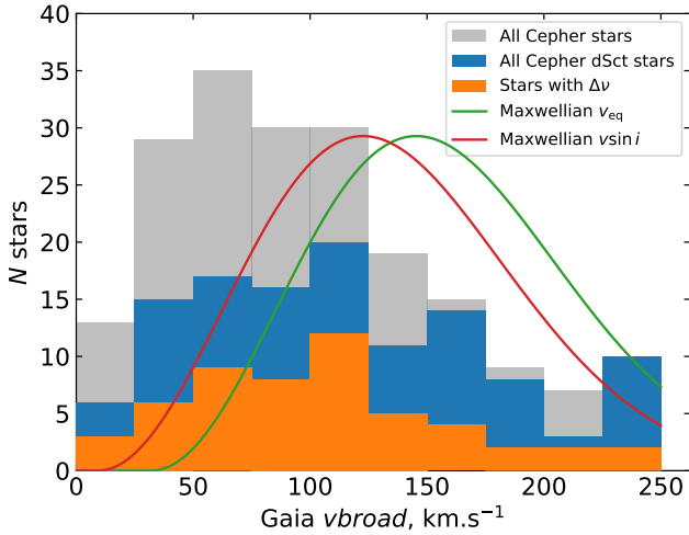
Figure 11. Gaia v_{\text{broad}} distribution for Cep–Her stars, based on pulsation properties. All three samples have been confined to the colour where \delta Sct stars are found. The grey histogram shows all Cep–Her stars in the ZAMS group, the blue histogram shows those that are \delta Sct stars, and the orange histogram shows \delta Scuti stars for which a \Delta\nu value could be measured. The green curve is the Maxwellian distribution of equatorial rotation velocities from Zorec & Royer (2012) for stars of mass 1.6 to 2.0 M_{\odot} . Note that close binaries and chemically peculiar stars are removed from that sample to give the distribution for (superficially) normal, single stars. The red curve is the same distribution divided by \sqrt{3}/2 to (crudely) reproject it into an observed ( v \sin i ) distribution.
