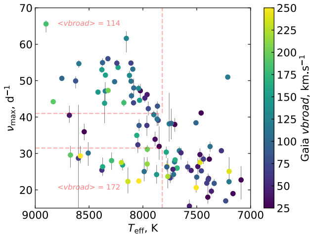
Figure 8. The v_{\max} and T_{\text{eff}} values for Cep–Her stars in the ZAMS group, colour-coded by their Gaia v_{\text{broad}} values. Dashed lines separate stars that are unambiguously on the bottom ridge from those on the upper ridge, and the mean v_{\text{broad}} within each division is shown.
