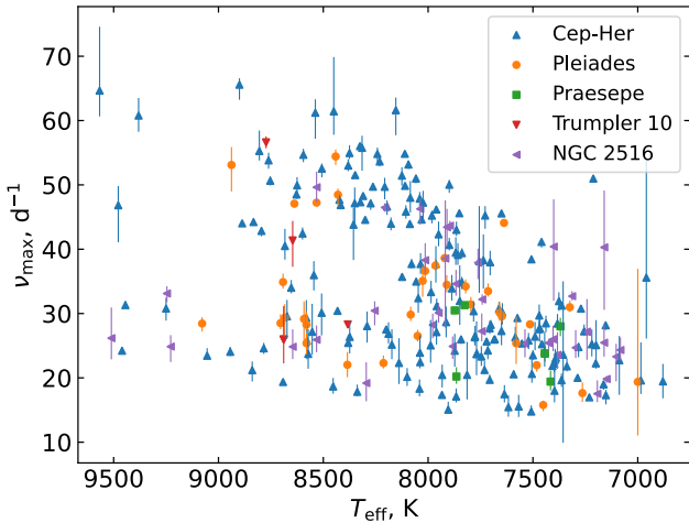
Figure 7. The distributions of v_{\max} and T_{\text{eff}} for the handful of clusters described in Sec. 3.3. Symbols denote the mean of the aggregate methods for measuring v_{\max} , while vertical bars span the range of v_{\max} from those methods for each star. One of the Praesepe stars lies outside the plot range (TIC 30307085, v_{\max} = 61.0 \text{ d}^{-1} , T_{\text{eff}} = 9931 \text{ K} ), but consistency with Fig. 6 was retained. Of interest is the emerging structure of two ridges that merge around 8000 K.
