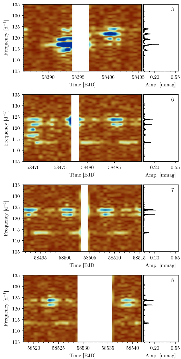
Figure A2. Wavelet plots by sector. The time is BJD – 2400000. The amplitude modulations from both the changing view of oblique pulsation with the 7.679696-d rotation and the secular changes can be seen. The colours range linearly from amplitude zero (red) to amplitude 0.6 mmag (blue). The sectors are numbered in the top right corner of each plot. The plots are for 120-s cadence data, unless otherwise noted.
