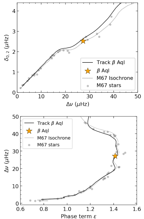
Fig. 14. Small frequency separations \delta\nu_{0,2} (top) and phase term \epsilon (bottom) sequences from M67 stars, taken from Reyes et al. (in press) and Reyes et al. (submitted), respectively. \beta Aql is shown with a star symbol.
