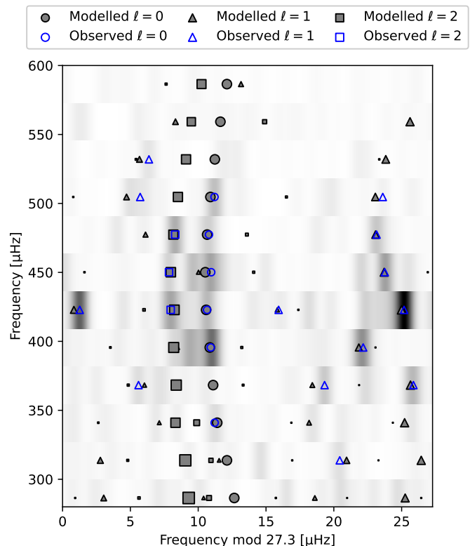
Fig. 13. Reconstructed power spectrum of \beta Aql (greyscale) with the observed frequencies (open blue symbols; Table 1) and model frequencies (filled black symbols).
