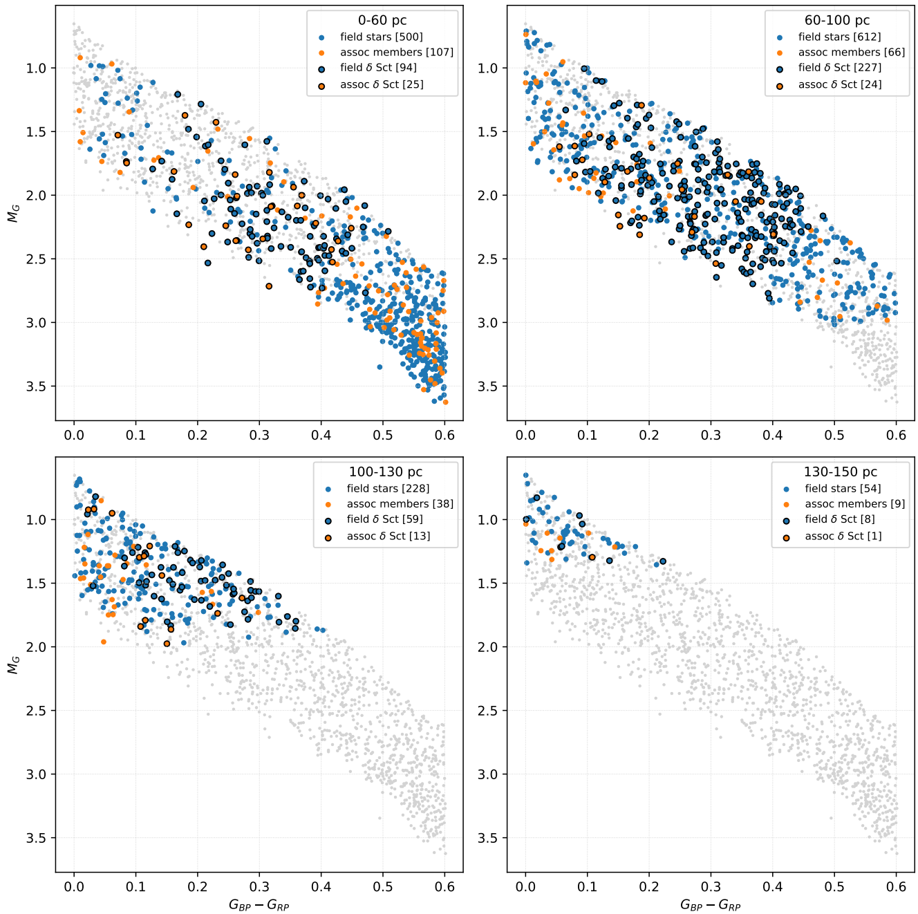
Figure 10. Colour-magnitude diagrams for the examined subsample described in Section 3.4. The stars are colour-coded according to their membership. In each panel we plot stars selected by distance, on top of the whole subsample, which we marked with grey dots.
