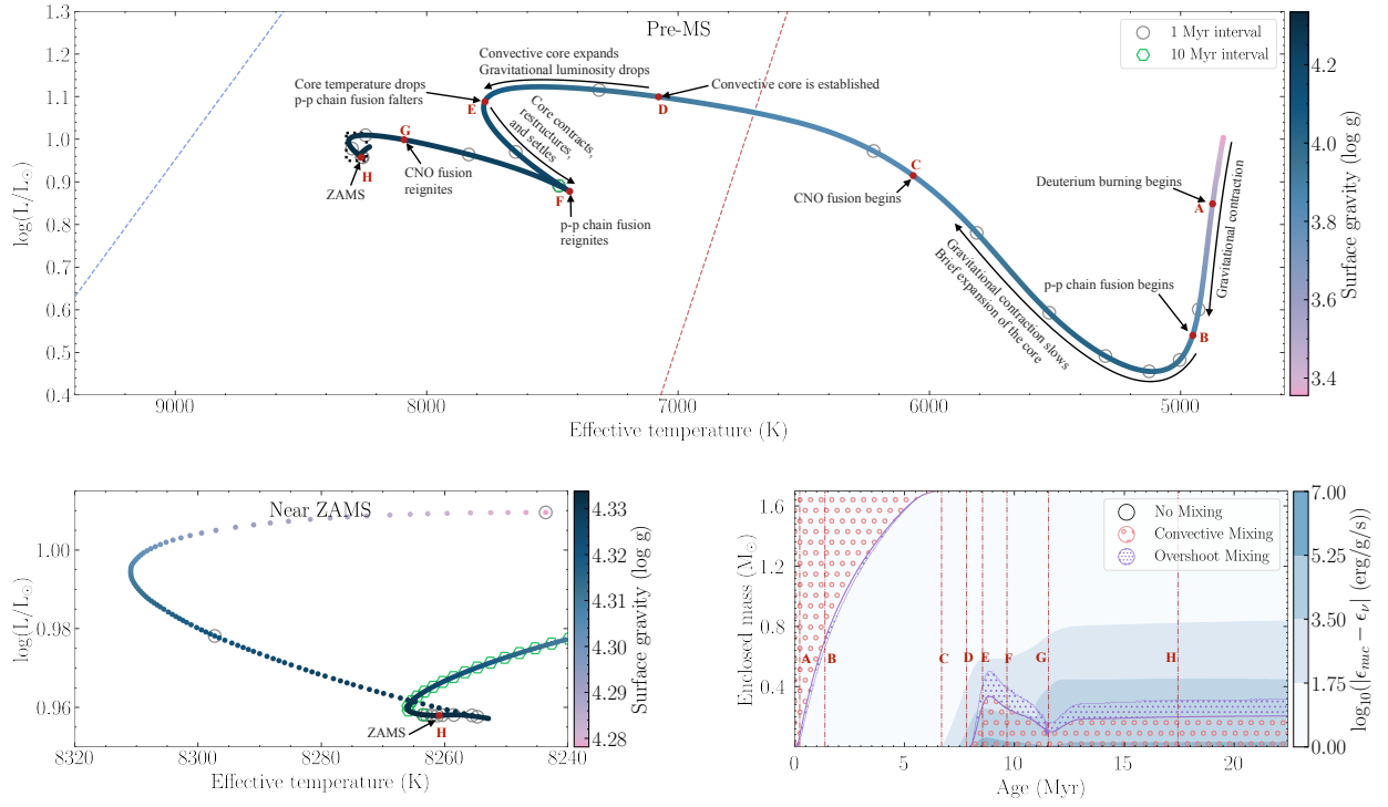
(a) Pre-MS evolution up to ZAMS
