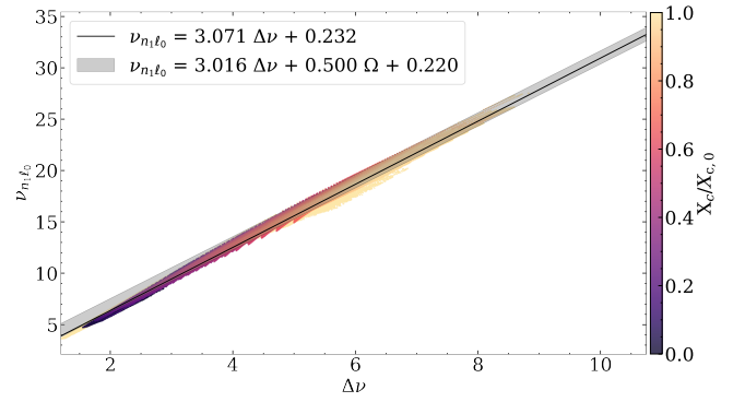
Figure 10. Relationship between the fundamental radial mode frequency ( \nu_1 ) and the large frequency separation ( \Delta\nu ) across our grid of models that lie within the instability strip. The points represent individual models spanning pre-MS, MS, and post-MS contraction phases.
