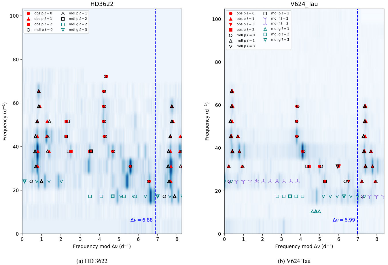
Figure 8. Échelle diagrams for HD 3622 and V624 Tau. The red filled markers indicate the identified modes and the overlaid unfilled markers represent modes from the least squares best-fit model.
