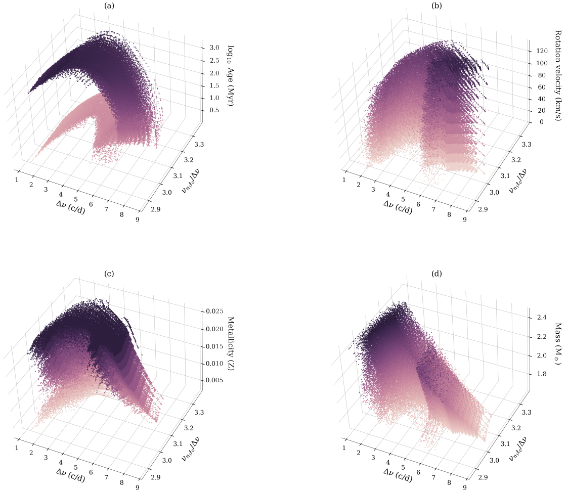
Figure 11. Visualization of the offset parameter \nu_{n_1 \ell_0} as a function of large frequency separation \Delta\nu , for models within the classical instability strip (Dupret et al. 2004). The four panels display trends with stellar parameters shown along the vertical ( z -) axis and indicated by colour: (a) \log(\text{Age}/\text{Myr}) , (b) equatorial rotation velocity ( v_{\text{eq}} , \text{km s}^{-1} ), (c) metallicity ( Z ), and (d) stellar mass ( M/M_{\odot} ). To aid readability, every 100th model is plotted for ages below 50 Myr, and every 5th model beyond that. To further reduce visual clutter, a sparse sampling in metallicity is used.
