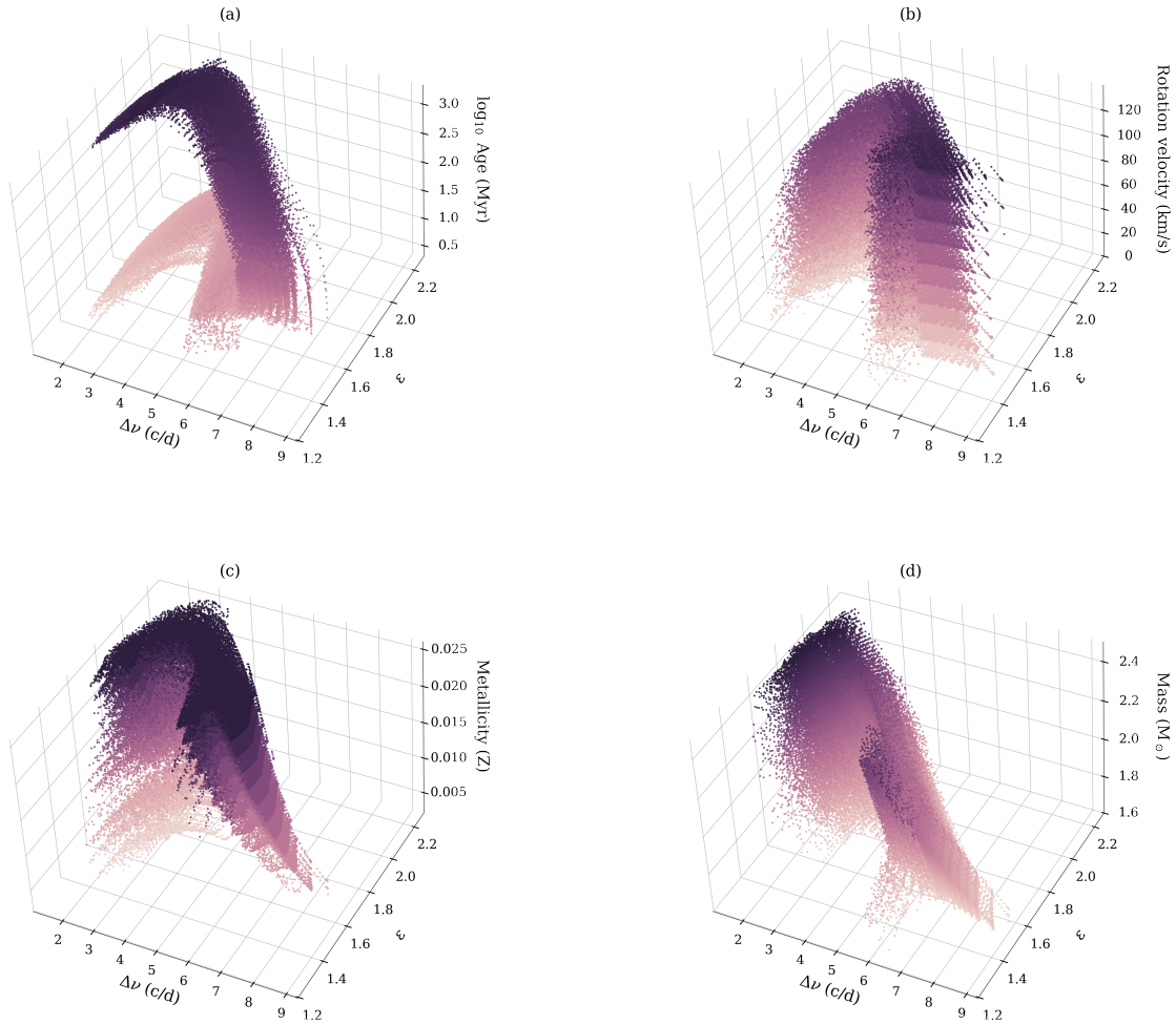
Figure 12. Three-dimensional visualization of \epsilon as a function of \Delta\nu , across all of our models that lie within the classical instability strip. Each panel shows a different global stellar parameter on the vertical ( z -) axis and encoded via colour: (a) \log(\text{Age}/\text{Myr}) , (b) equatorial rotation velocity ( v_{\text{eq}} , in \text{km s}^{-1} ), (c) metallicity ( Z ), and (d) stellar mass ( M/M_{\odot} ). Here we present models of mass \geq 1.6M_{\odot} , showing every 100th model for ages younger than 50 Myr, and every 5th model thereafter. Models are also thinned in metallicity.
