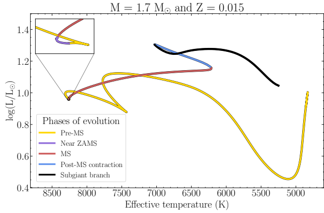
Figure 1. Phases of evolution of a typical 1.7 M_{\odot} , solar-metallicity \delta Sct star on the Hertzsprung-Russell diagram.
