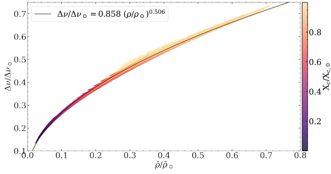
Figure 9. Power-law fit to the scaling relation between large frequency separation ( \Delta\nu ) and mean stellar density ( \bar{\rho} ) for models within the classical instability strip. Points are coloured by the central hydrogen fraction normalized to its initial value ( X_c/X_{c,0} ), providing a proxy for stellar age and evolutionary phase. Since our models are non-uniformly sampled in age, we display every 20th model for ages below 50 Myr to reduce visual clutter, while all MS and post-MS models are shown in full. The best-fit relation, shown in black, was derived using the full set of instability strip models.
