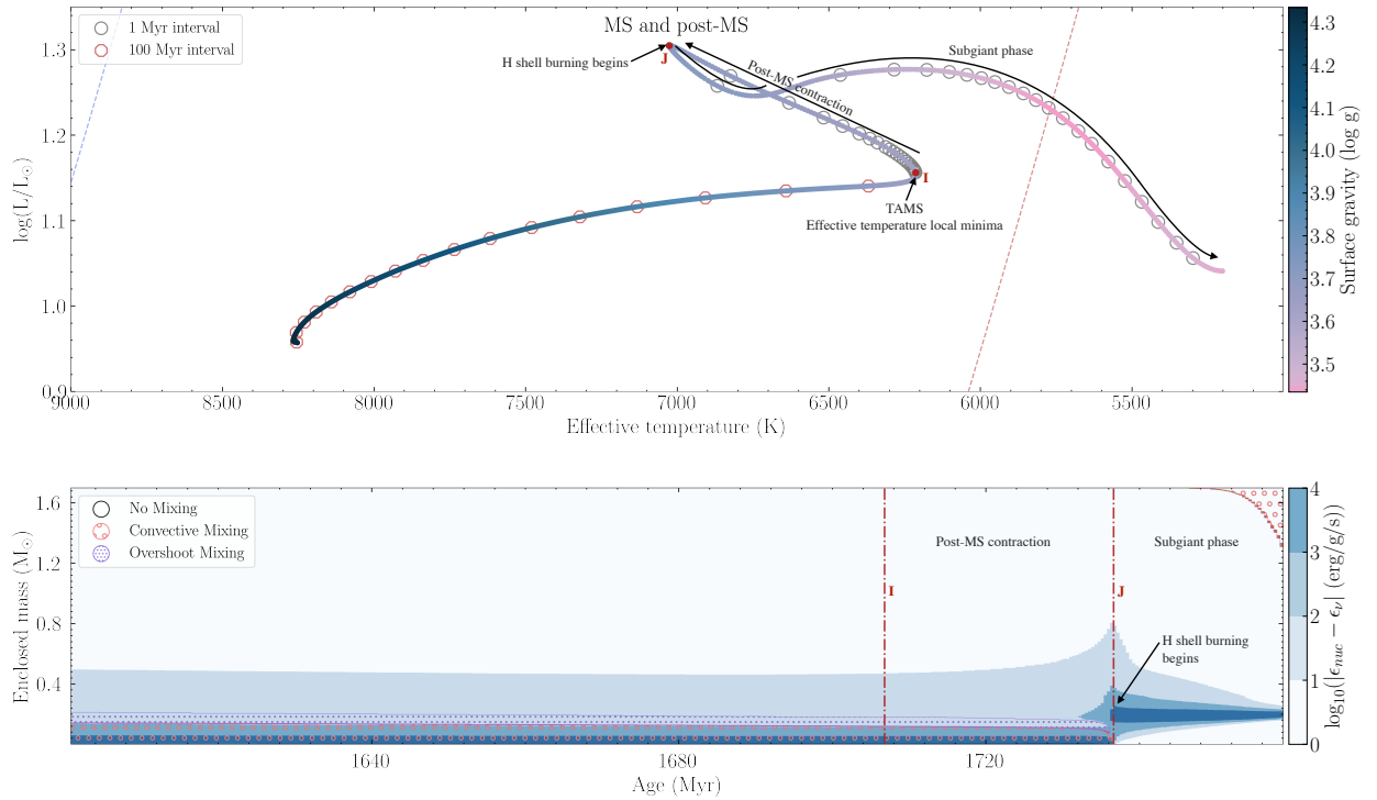
(b) MS and post-MS evolution
