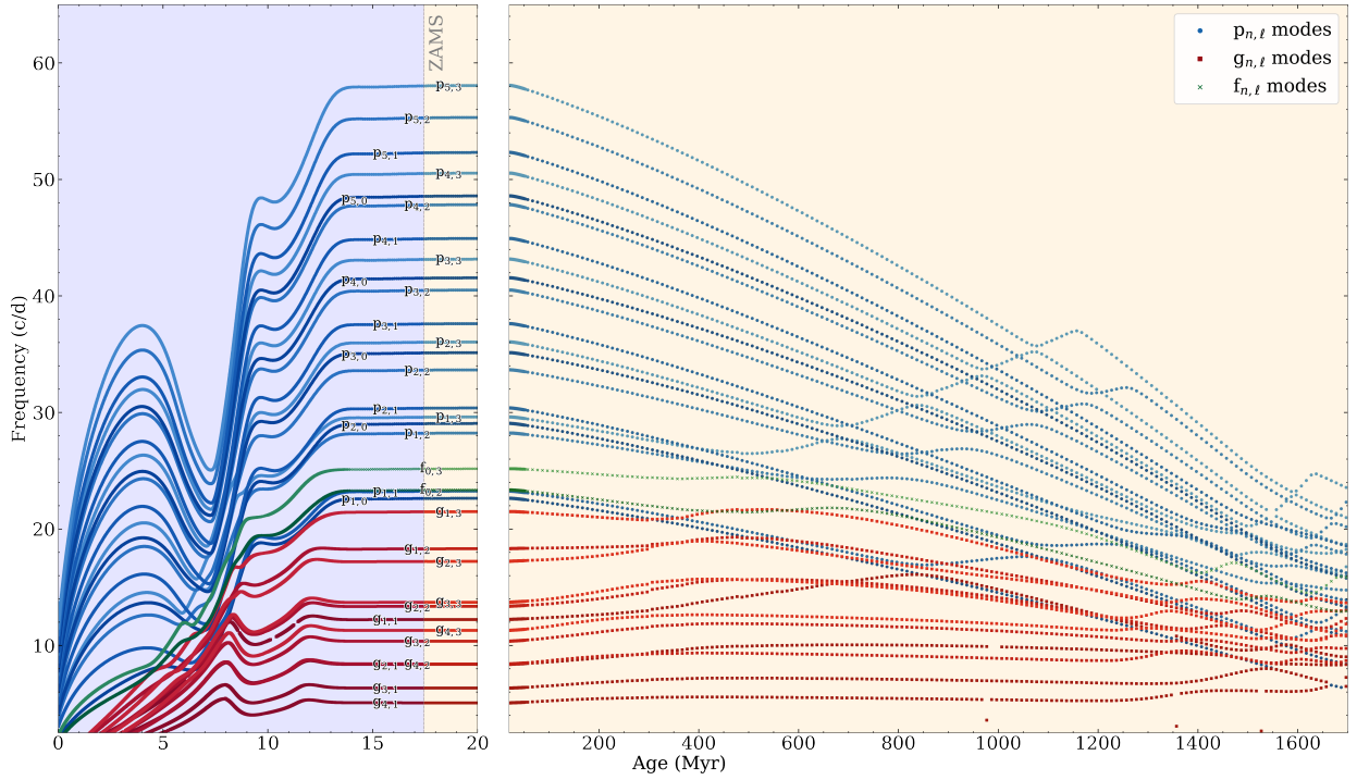
Figure 7. Evolution of stellar oscillation modes as a function of age for a 1.7\text{-}M_{\odot} , solar-metallicity star. The left panel shows the early evolution including the pre-MS and early MS phases, while the right panel displays the main sequence evolution. The vertical dashed line marks the ZAMS. Different mode types are colour-coded: p modes in blue, g modes in red, and f modes in green, with lighter shades for higher degree modes. The subscripts n, \ell denote the radial order and spherical degree of each mode. Only a subset of modes is shown for clarity, and rotational splittings are omitted.
