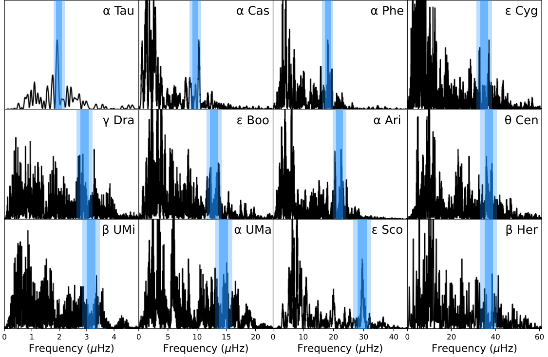
Figure 5. A gallery plot showing the power spectral density of the 12 RGs with measurable \nu_{\max} . The first panels shows the RGs in the region 0–5 \mu\text{Hz} , the second in the region 0–23 \mu\text{Hz} , the third at 0–44.5 \mu\text{Hz} , and the fourth at 0–61 \mu\text{Hz} . The blue shaded regions indicate 1\sigma and 2\sigma uncertainties of the derived \nu_{\max} . We note that \beta Gem (Pollux) is not included in this figure.
