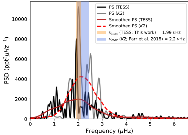
Figure 7. The power density spectrum of \alpha Tau (Aldebaran) from both TESS (black) and K2 (gray). The smoothed powers, which was smoothed with an Epanechnikov filter (Epanechnikov 1969), with a width of 2 \mu\text{Hz} , are shown as a dark red solid line (TESS) and as a red dashed line ( K2 ). The orange shaded region represents 1\sigma region of the derived \nu_{\max} from PYMON, while the blue shaded region represents 1\sigma region of the K2 \nu_{\max} from Farr et al. (2018).
