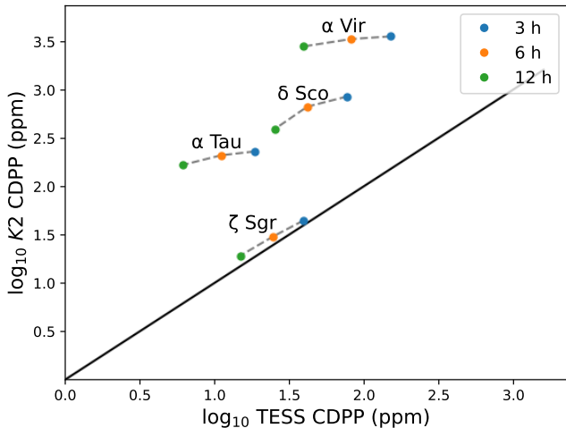
Figure 14. Correlation diagram of the 3, 6, and 12 h LIGHTCURVE-computed CDPP for both the TESS and K2 HALOPHOT light curves. Grey dashed lines connect the CDPPs associated with a given star.
